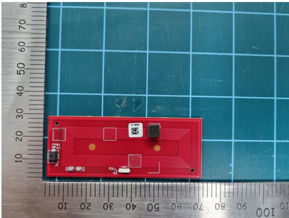
<Antenna C – Front>
