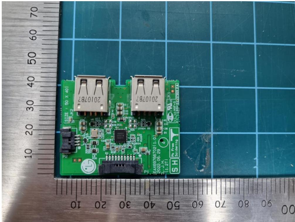
<USB Board – Front>
