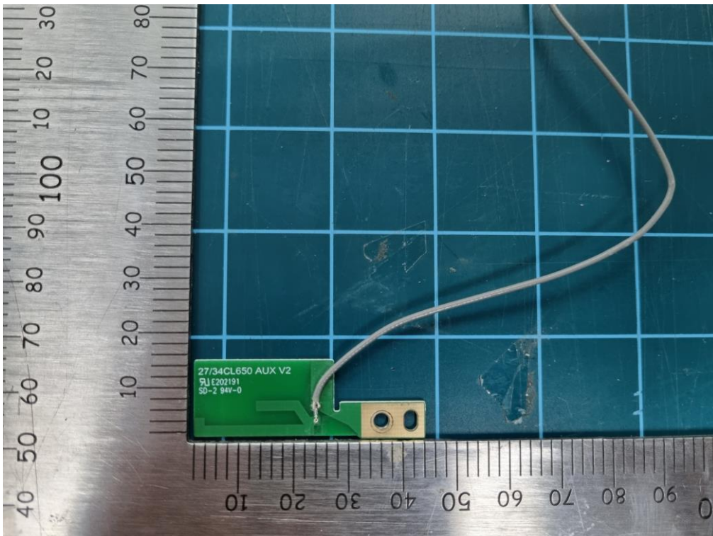
<Antenna B – Front>
