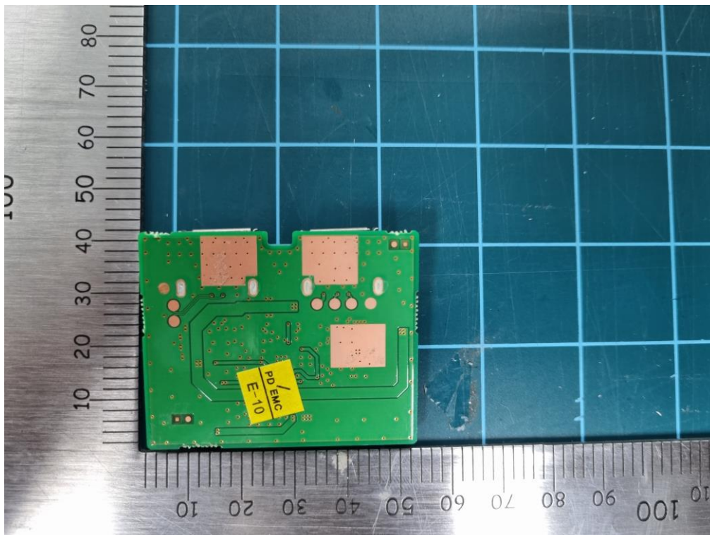
<USB Board – Rear>
