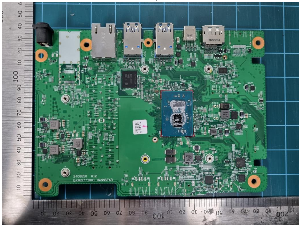
<Main board – Front(remove heat sink)>
