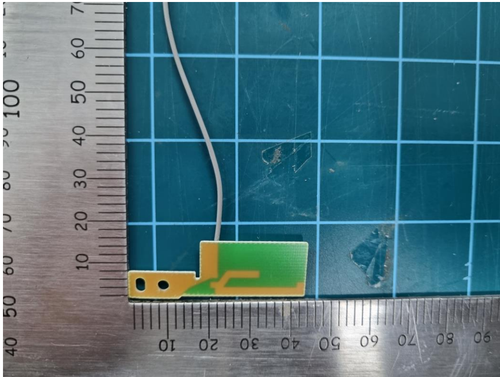
<Antenna B – Rear>
