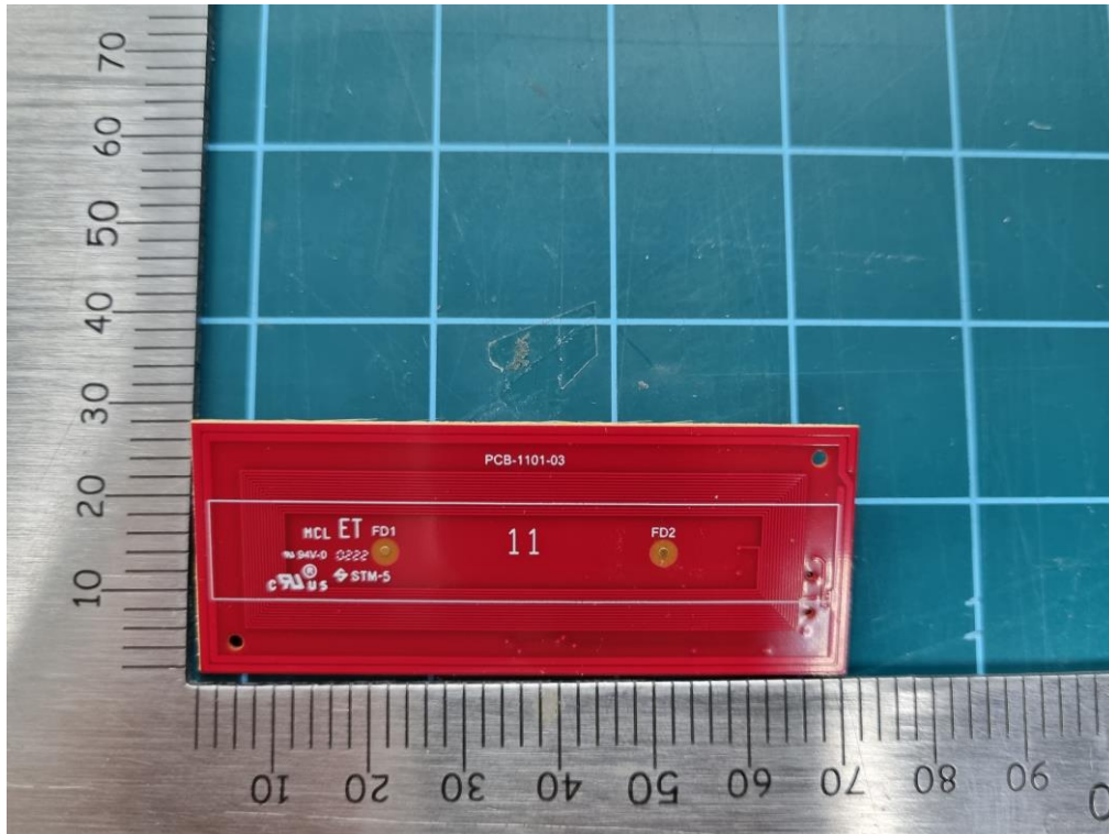
<Antenna C – Rear>
