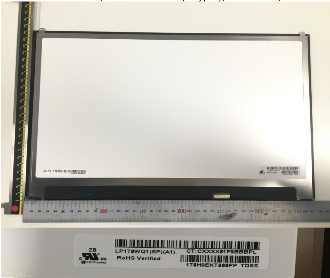
Figure 43 LGD, M/N LP170WQ1(SP)(A1), LCD Panel, Back View
