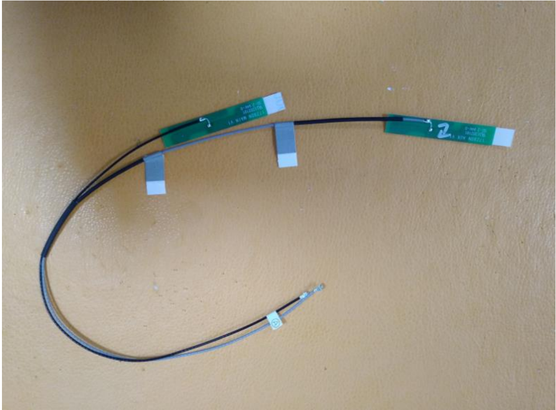
Figure 53 LG (INPAQ), M/N WA-P-LBLB-04-068 WLAN Combo Antenna
