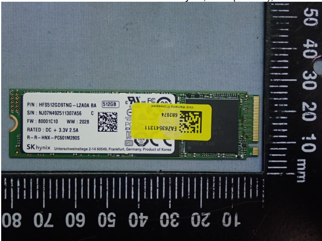
Figure 62 SK hynix, SSD (512GB), Front View
