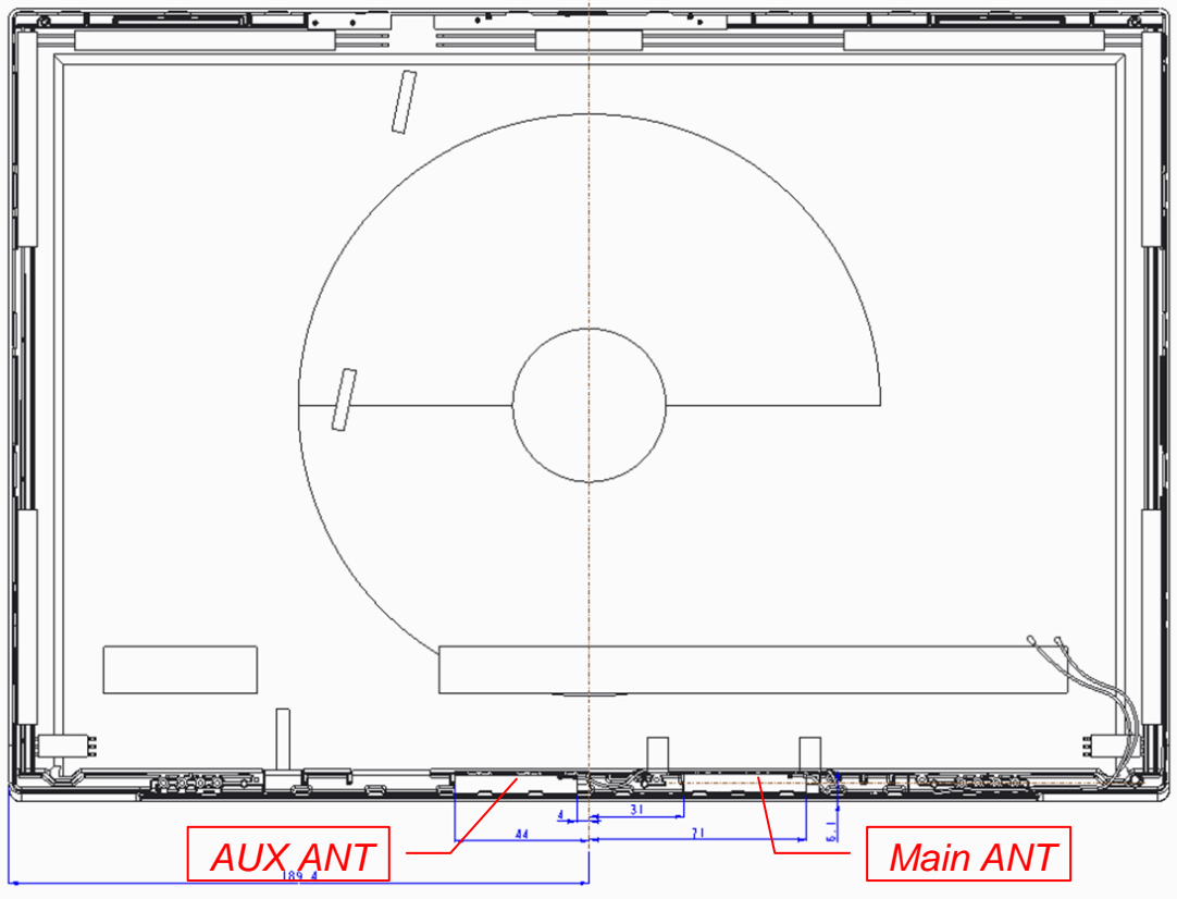
Figure 28 WA-P-LELE-04-011, WLAN Combo Antenna Position
