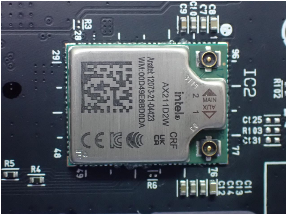
Figure 21 WLAN Combo Card, Front View
