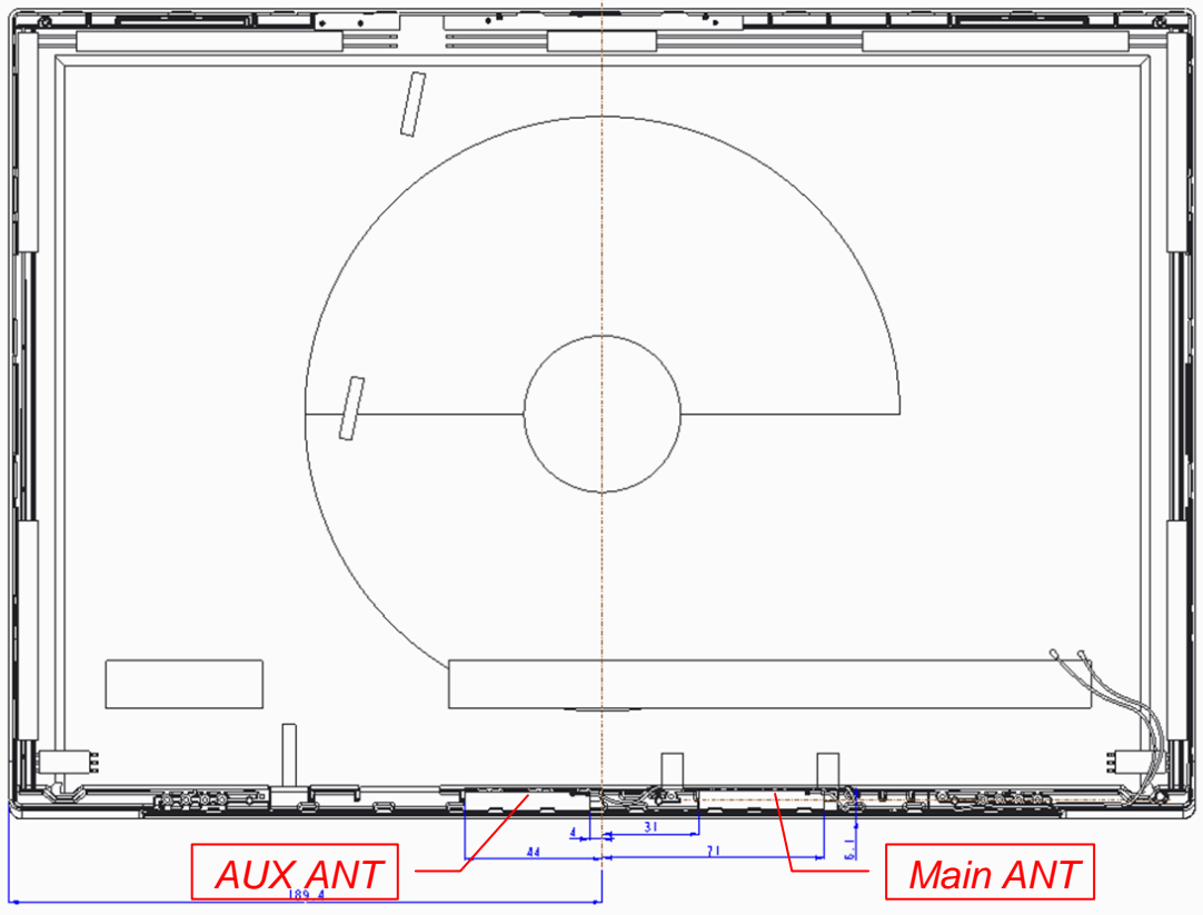
Figure 30 L1LRF009-CS-H, WLAN Combo Antenna Position
