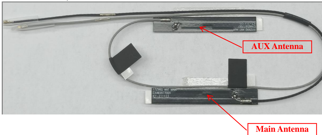
L1LRF009-CS-H, Antenna View
