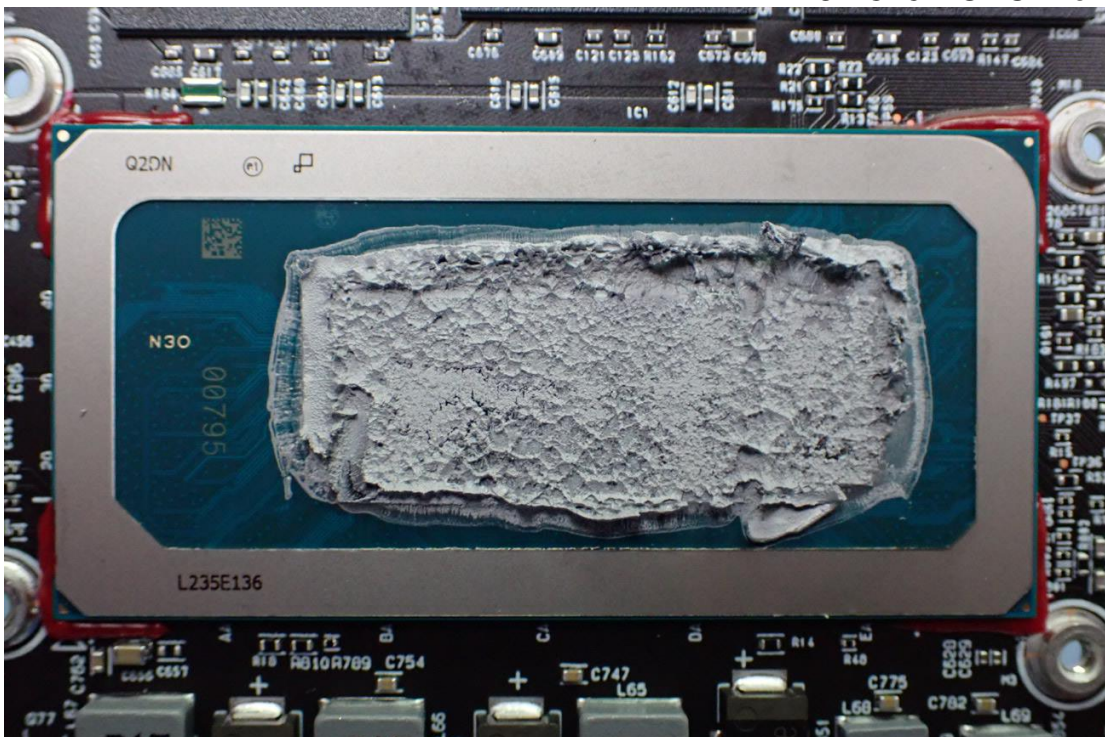
Figure 59 i5-1340P CPU View
