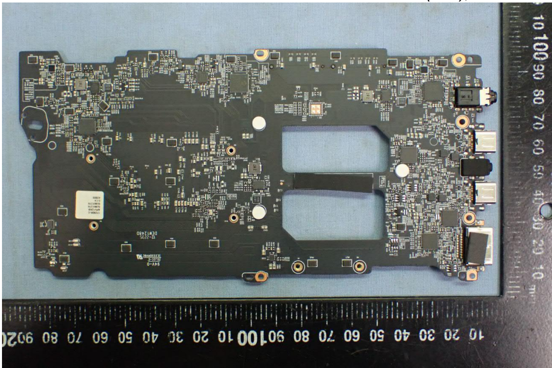
Figure 45 Main Board (GM), Back View
