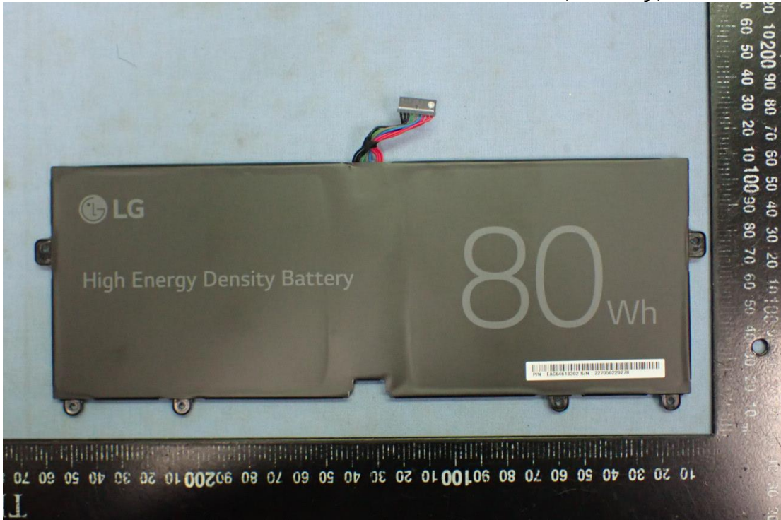
Figure 52 LBV7227E, Battery, Front View
