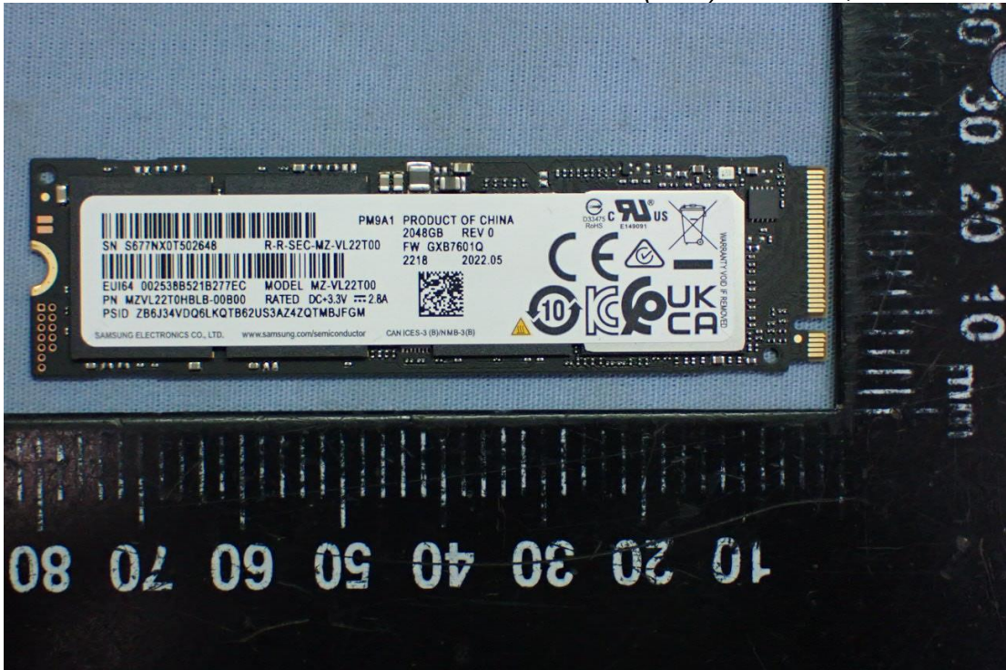
Figure 54 Worse (2TB) SSD #1 , Front View
