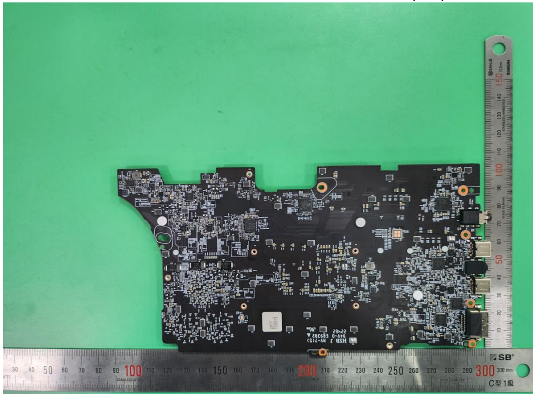
Figure 43 Main Board (PM), Back View
