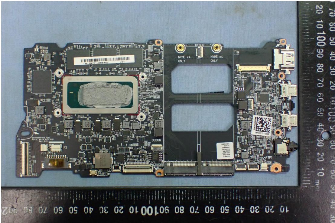
Figure 44 Main Board (GM), Front View
