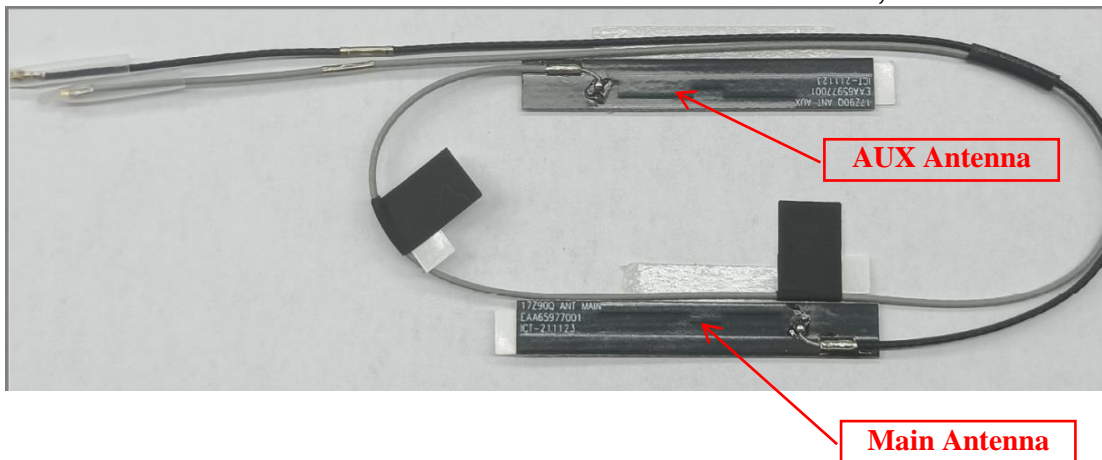
Figure 37 L1LRF009-CS-H, Antenna View
