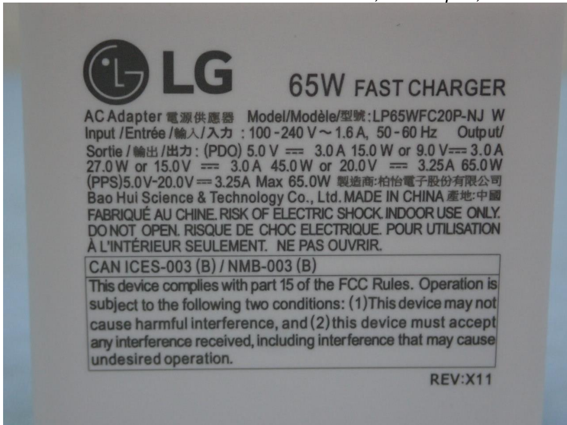
Figure 62 LP65WFC20P-NJ W, AC Adapter, Label View
