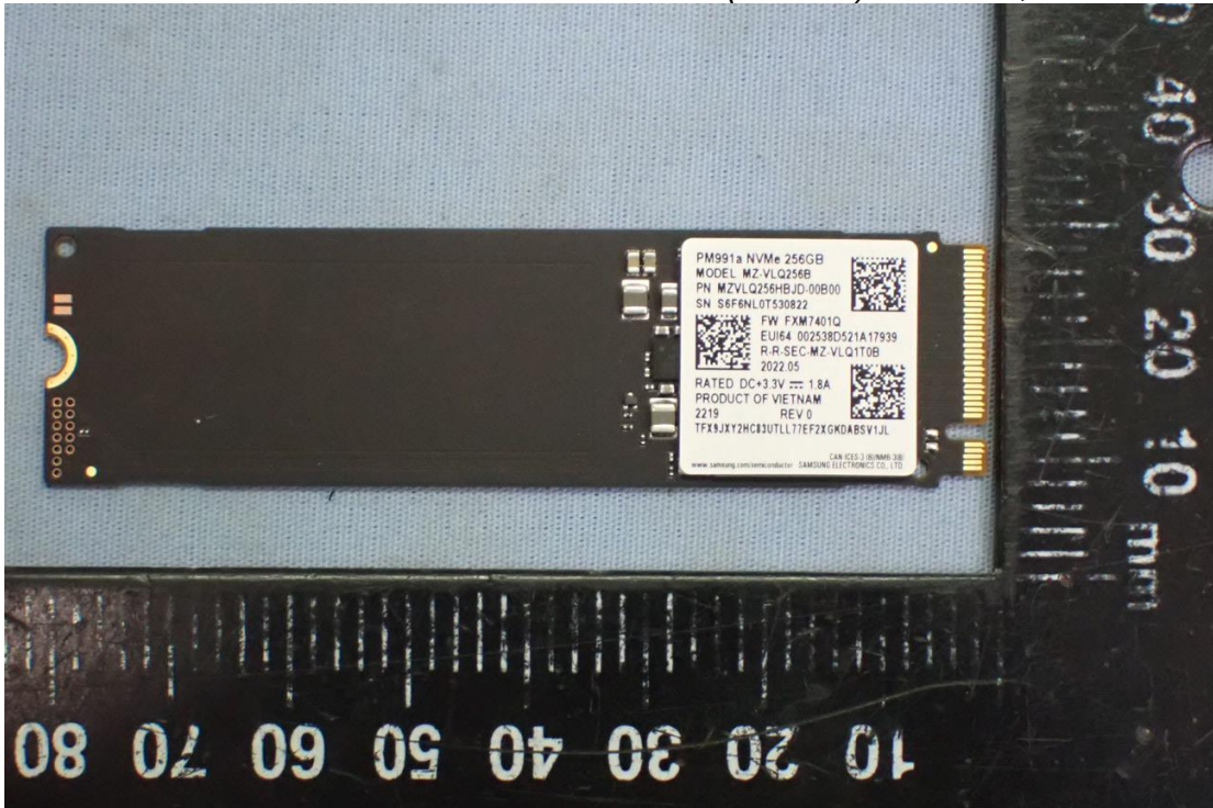
Figure 56 Worse (256GB) SSD #2 , Front View
