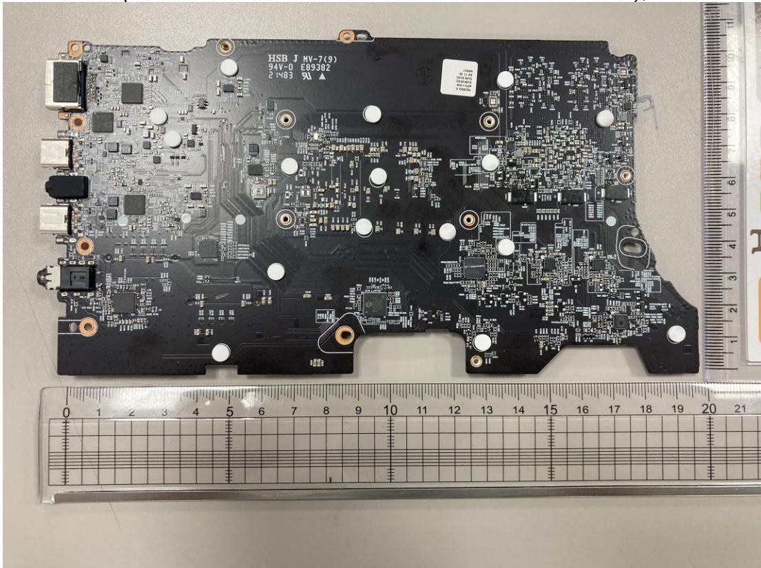
Figure 4 PM Main Board (Model: QUEEN NVIDIA MAIN B/D PCB w/ TPM), Back View
