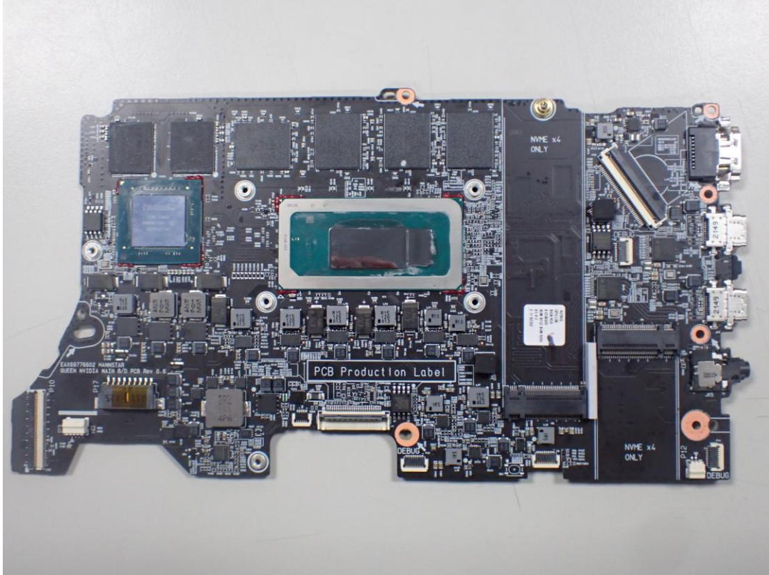
Figure 3 PM Main Board (Model: QUEEN NVIDIA MAIN B/D PCB w/TPM), Front View
