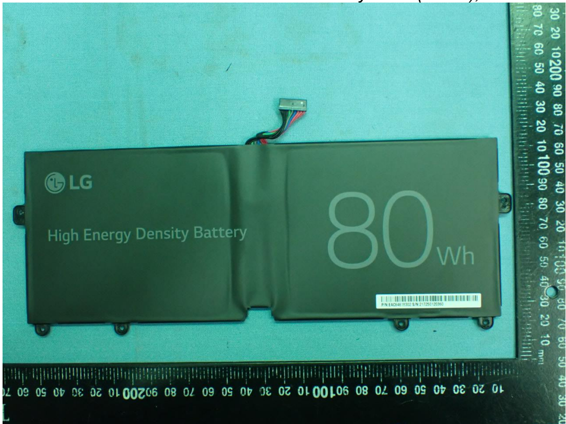
Figure 43 Battery Pack (80Wh), Front View
