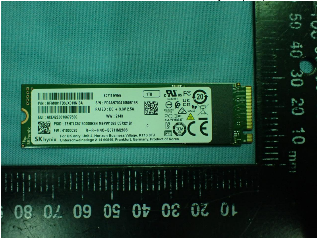
Figure 45 SSD, SK hynix, (1TB), Front View
