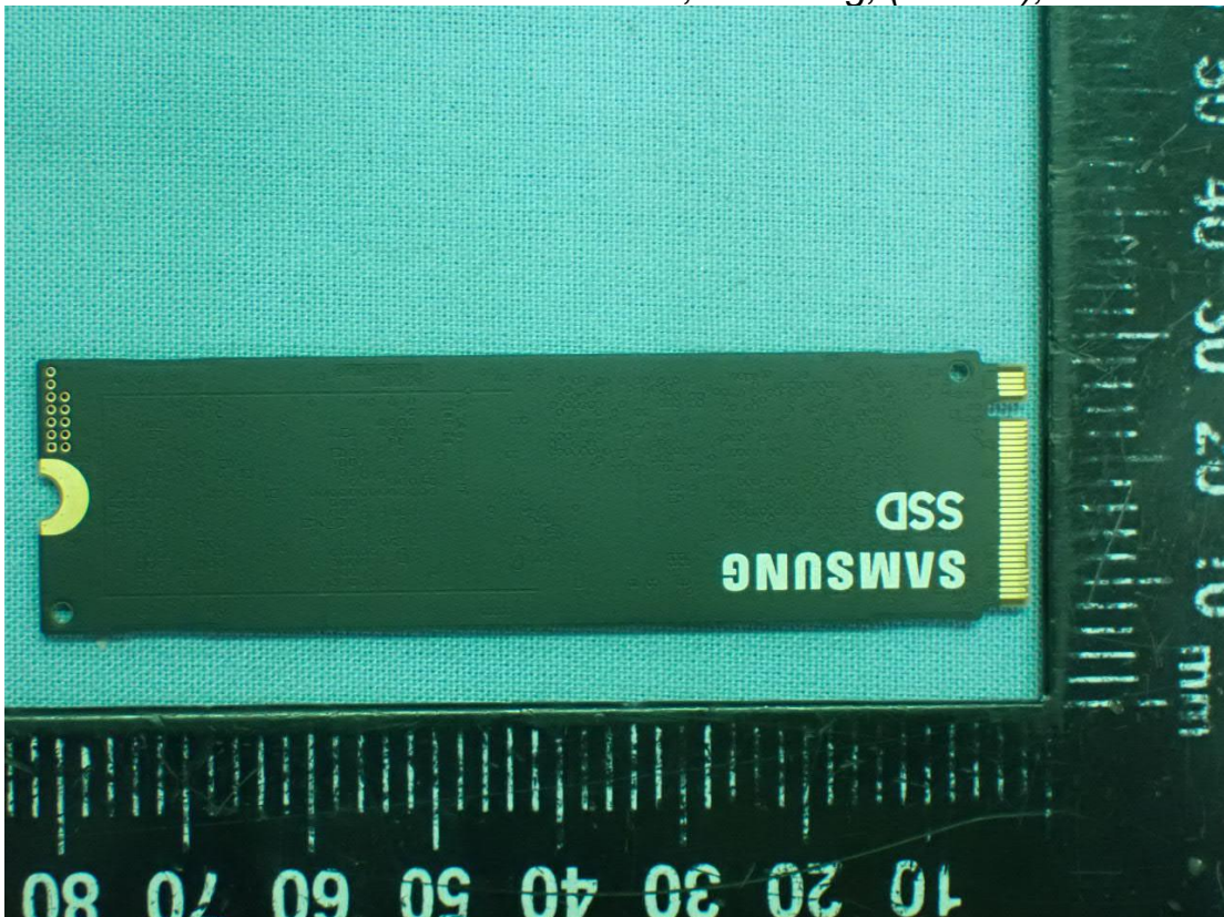
Figure 52 SSD, Samsung, (256GB), Back View
