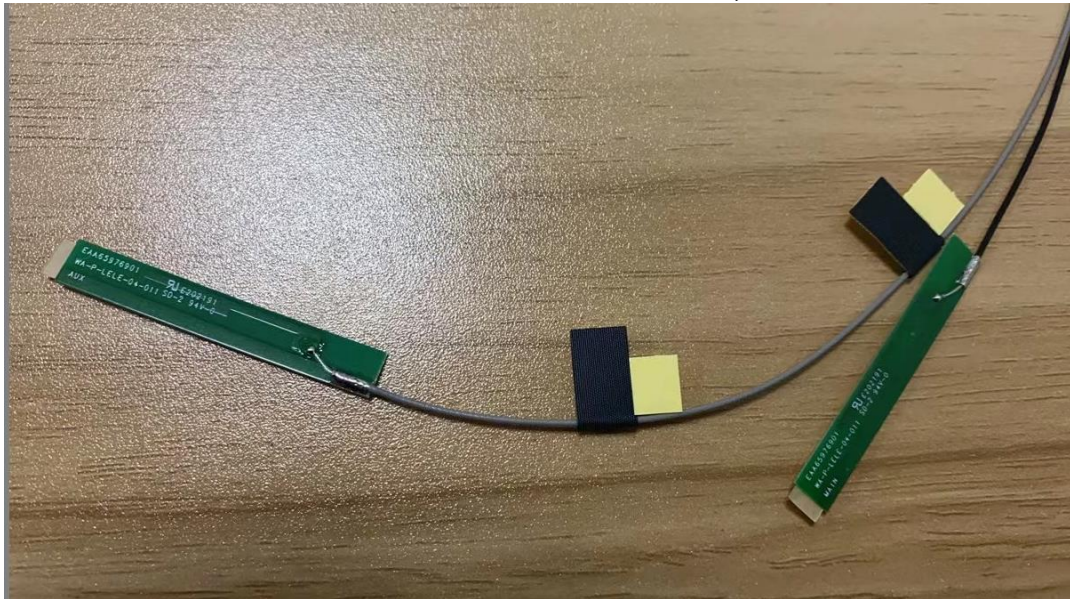
Figure 55 WA-P-LELE-04-011, WLAN Combo Antenna
