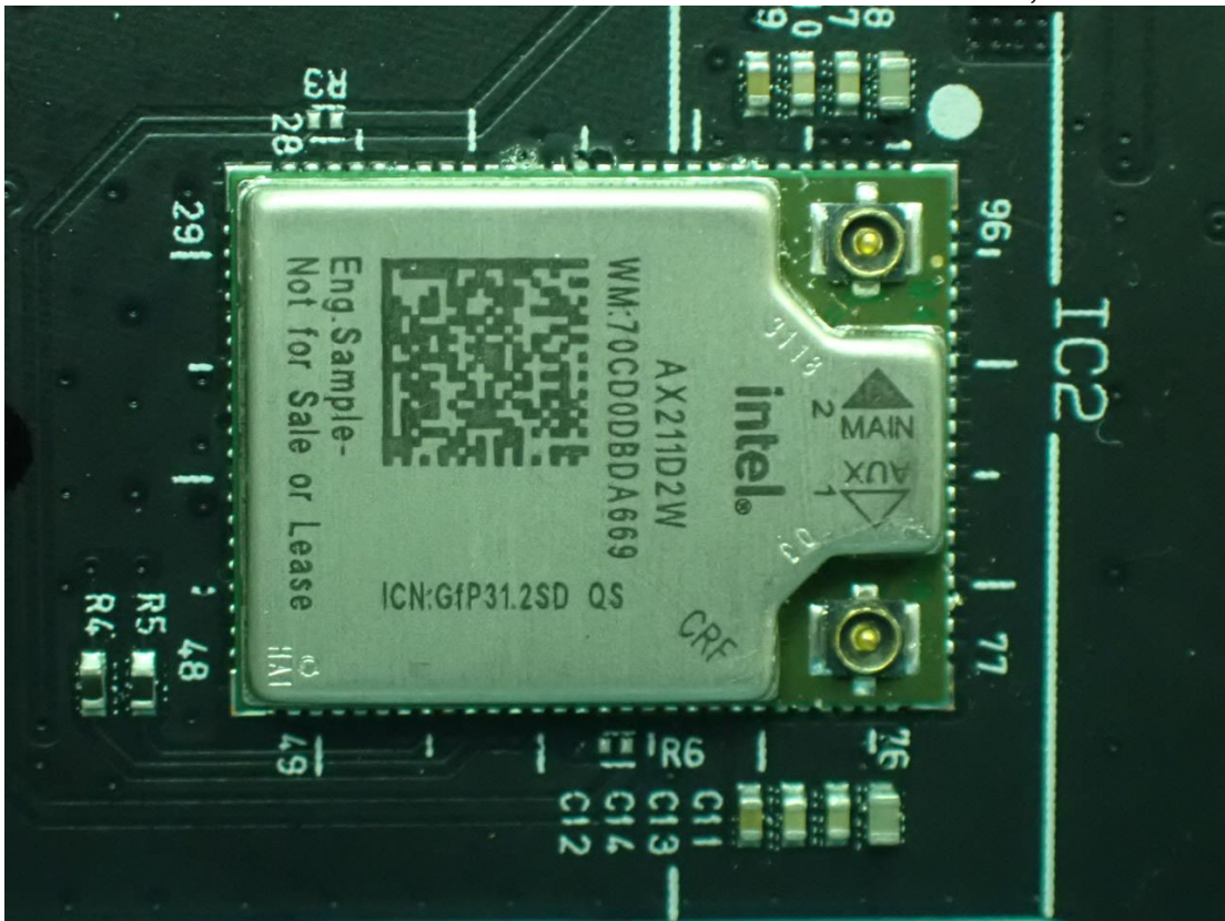
Figure 39 WLAN Combo Card, Front View
