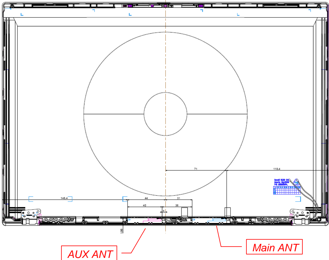
Figure 58 L1LRF009-CS-H, WLAN Combo Antenna Position
