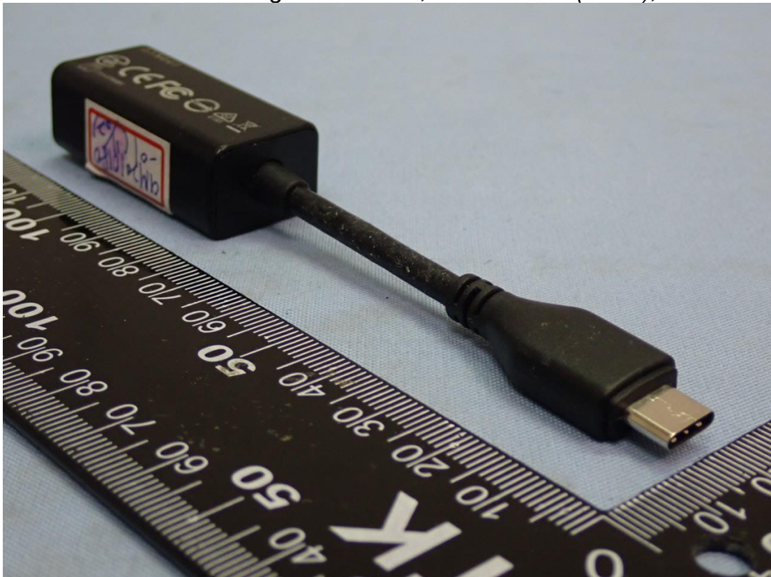
Figure 16 1000 Megabit Ethernet, LAN Gender (Black), Back View
