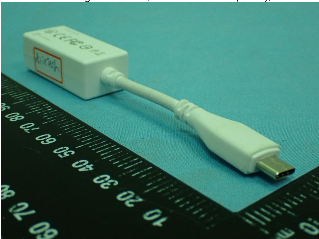
Figure 14 100 Megabit Ethernet, LAN Gender View (White), Front View
