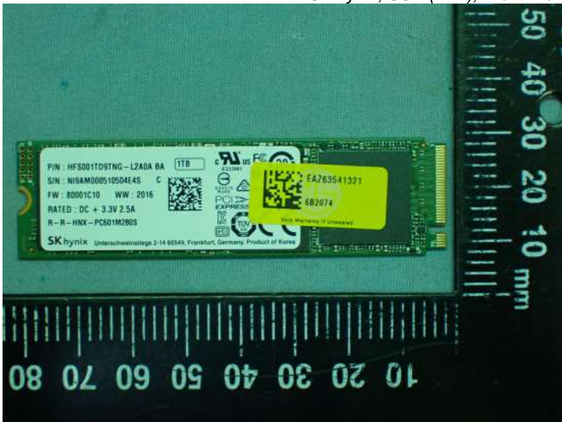
Figure 63 SK hynix, SSD (1TB), Front View
