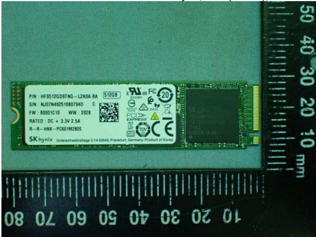
Figure 61 SK hynix, SSD (512GB), Front View
