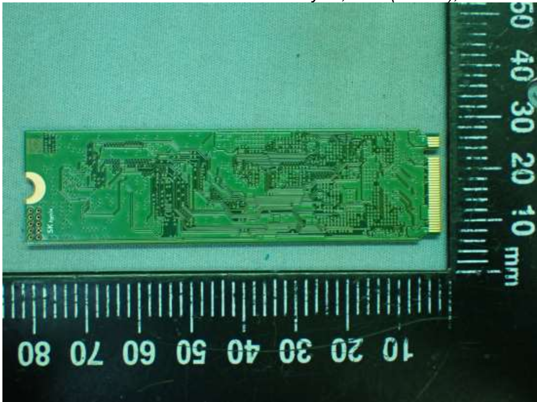
Figure 62 SK hynix, SSD (512GB), Back View
