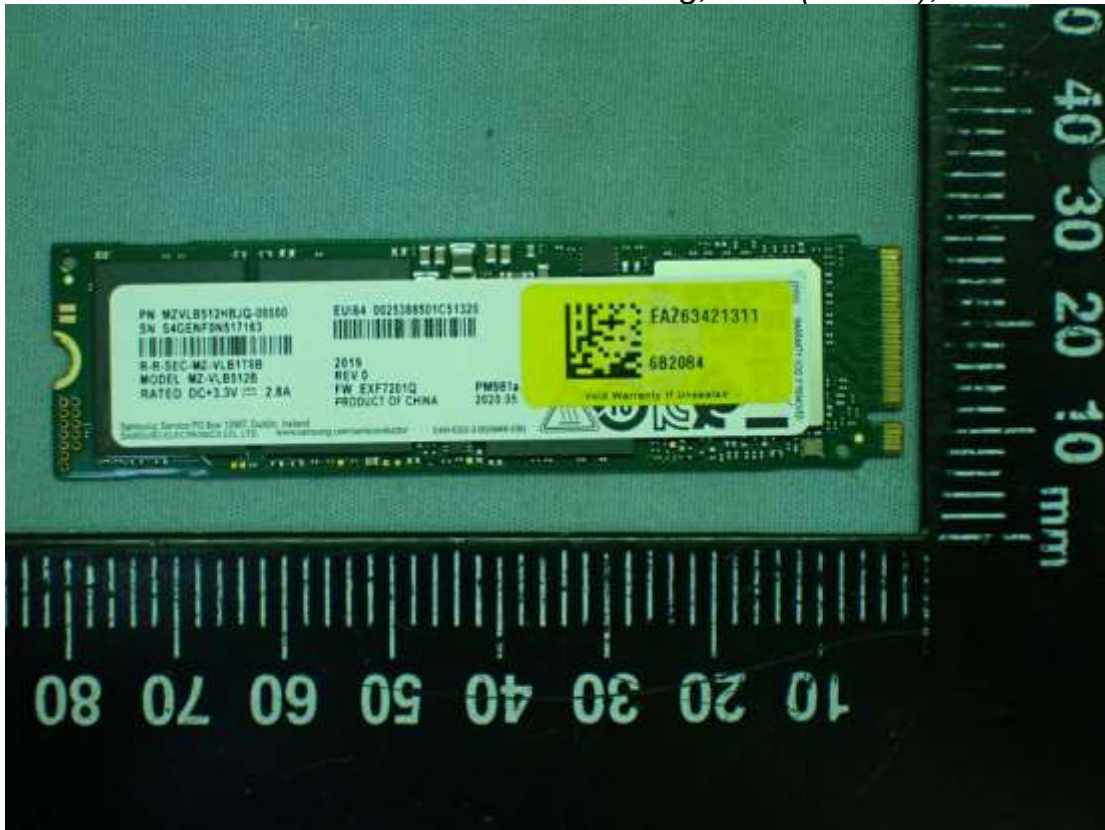
Figure 59 Samsung, SSD (512GB), Front View
