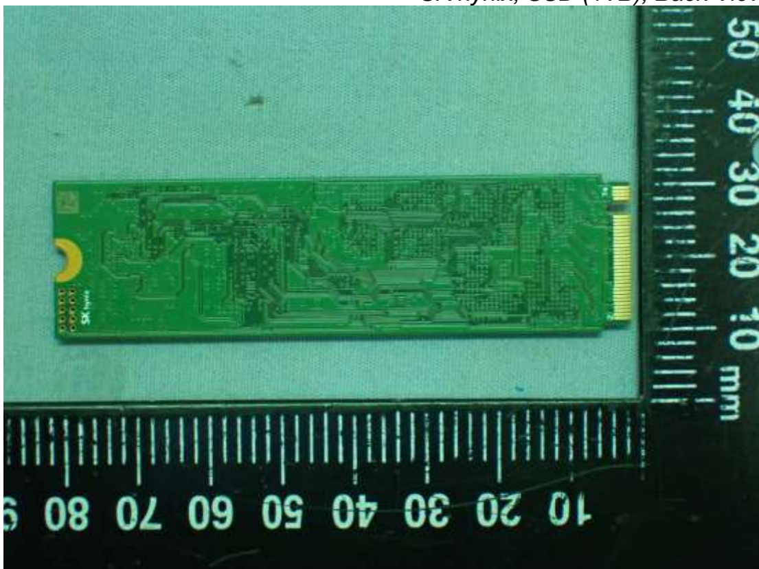
Figure 64 SK hynix, SSD (1TB), Back View
