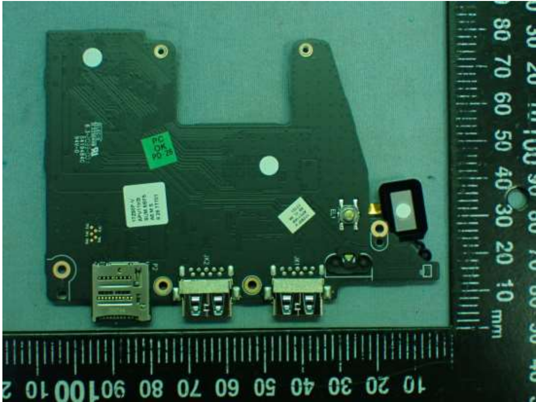
Figure 47 Elec&Eltek, WLAN SUB Board, Back View
