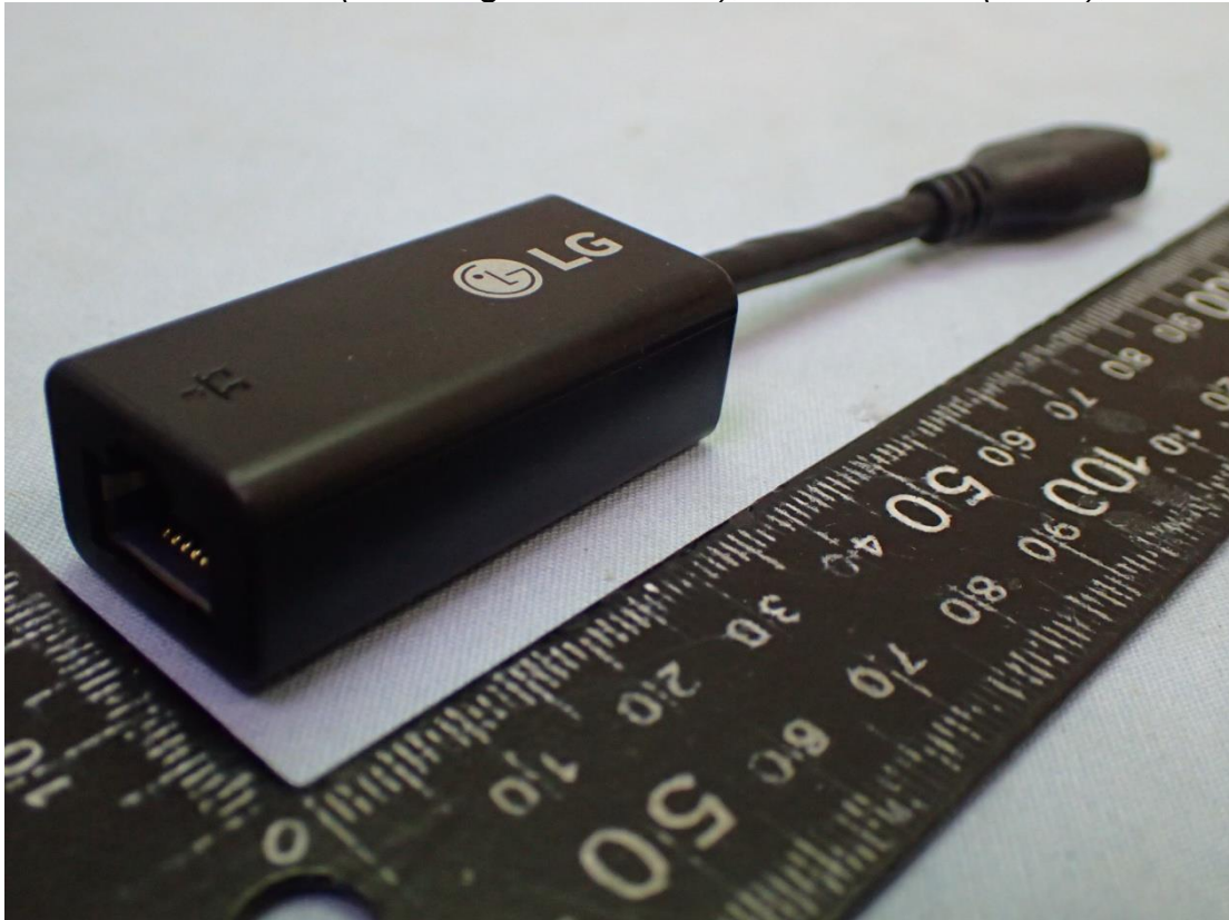
Figure 17 MEC & ARIN (100 Megabit Ethernet), LAN Gender (Black), Front View
