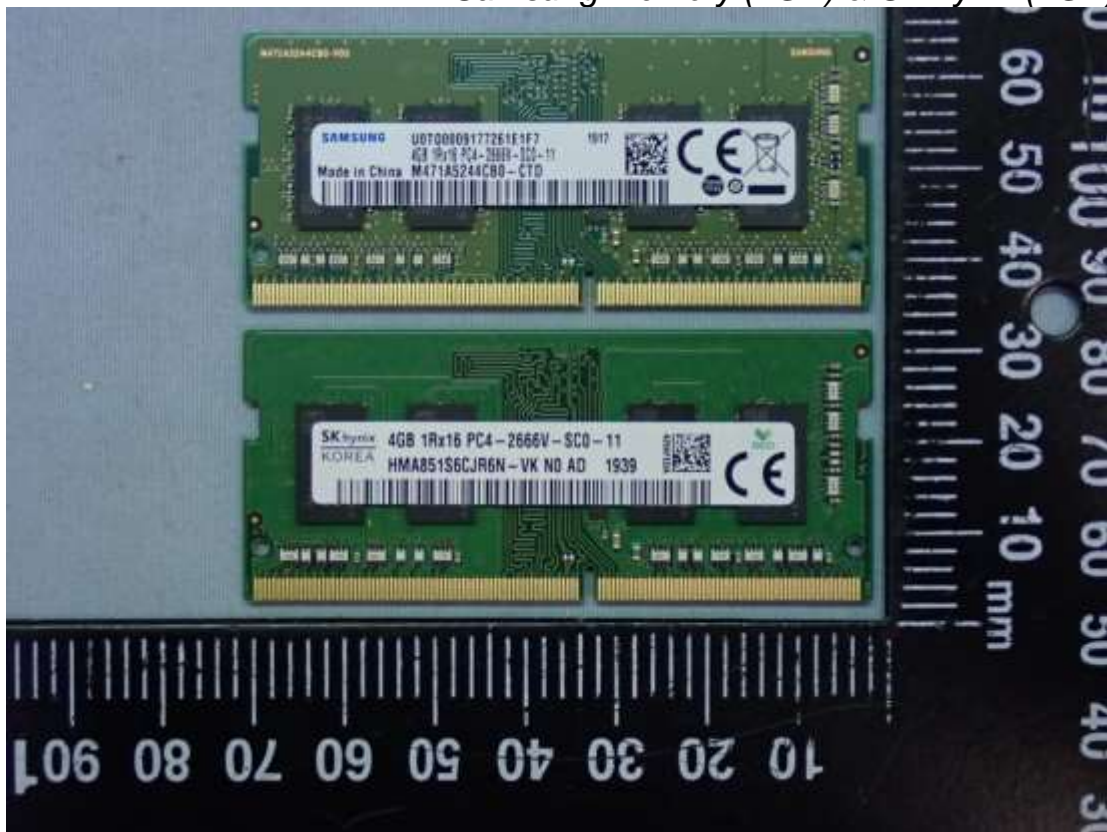
Figure 46 Samsung Memory (4GB) & SK hynix (4GB)
