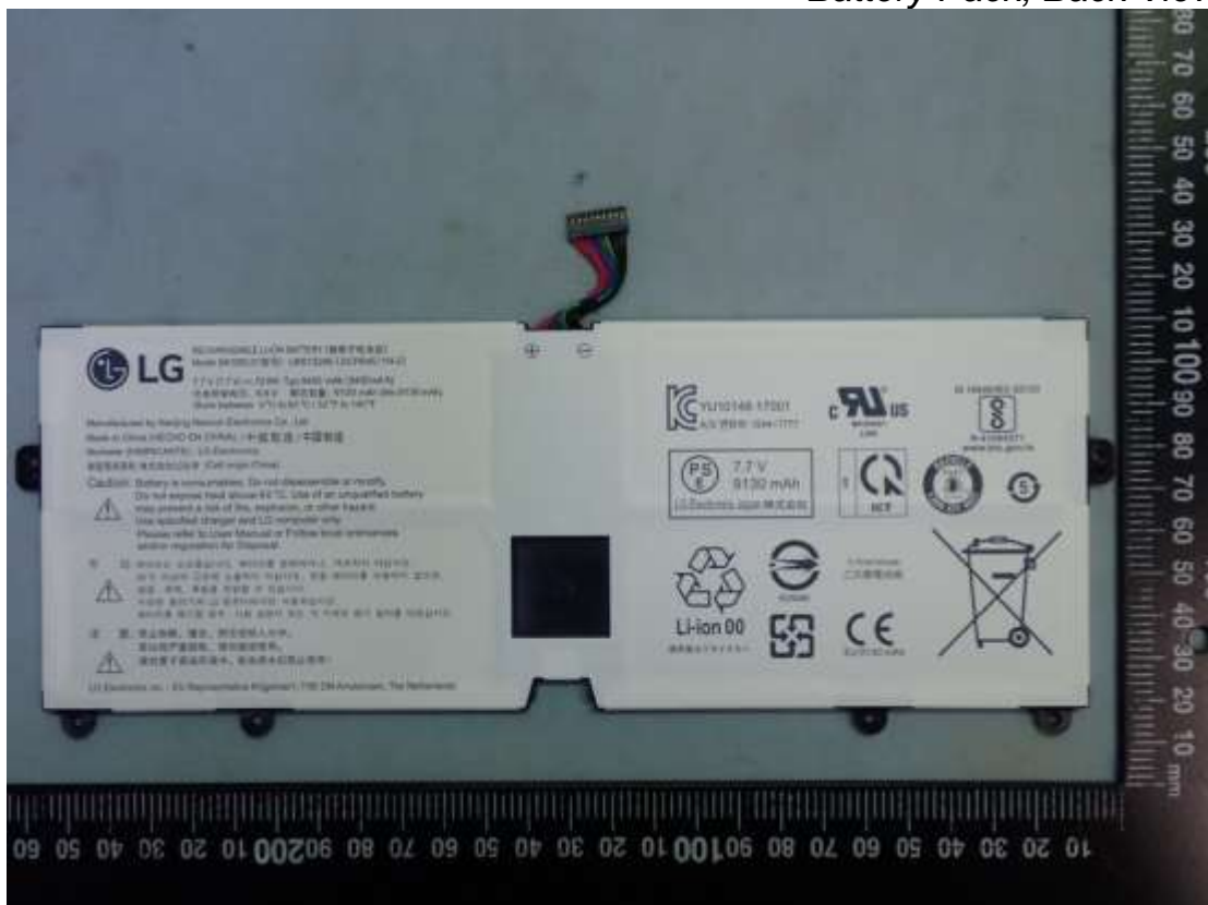
Figure 53 Battery Pack, Back View
