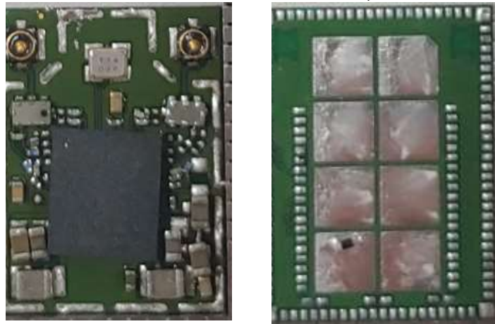
Figure 41 WLAN Combo Card, Remove Cover
