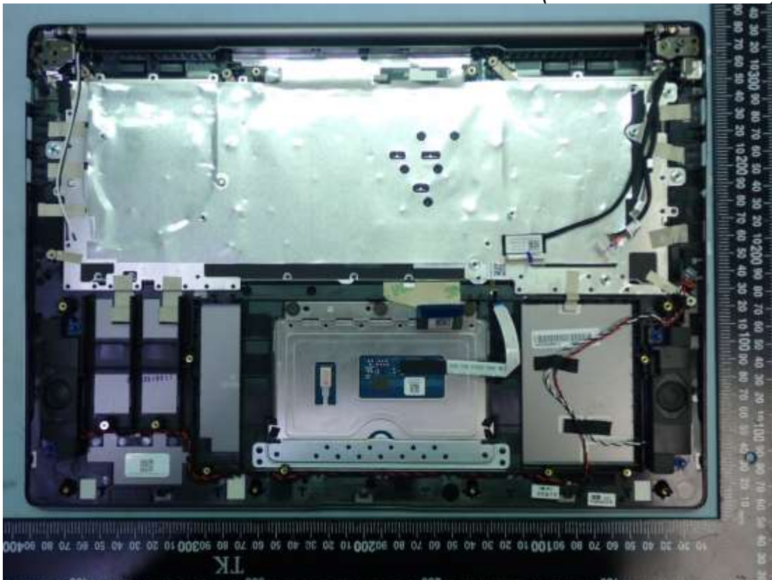
Figure 56 Internal View (with ELAN Click Pad)
