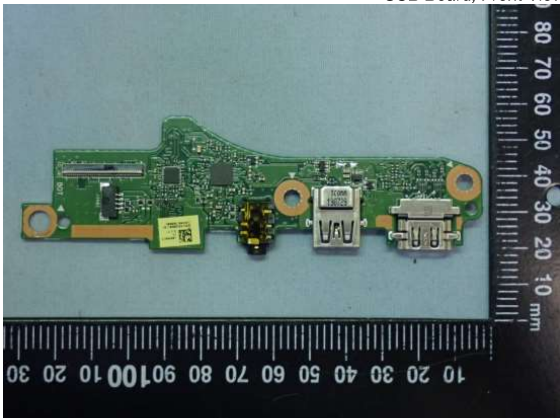
Figure 33 SUB Board, Front View
