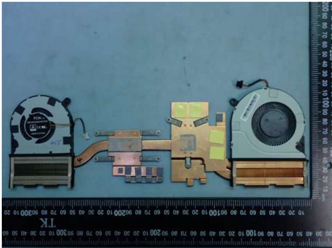
Figure 55 DC Fan & Heat Sink
