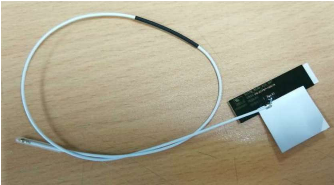
Figure 63 ACON(Advanced Wireless & Antenna Inc), M/N SJ17W_WLAN AUX ANT_HF Antenna
