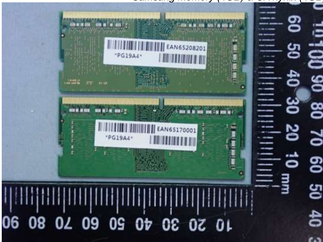
Figure 47 Samsung Memory (4GB) & SK hynix (4GB)
