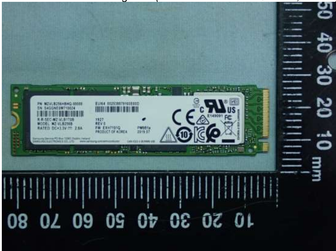
Figure 27 Samsung SSD (M/N MZVLB256HBHQ-00000, 256GB)
