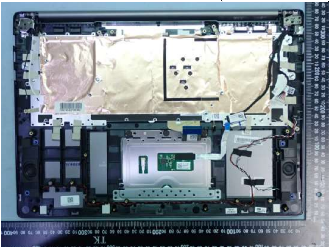
Figure 57 Internal View (with LITEON Click Pad)
