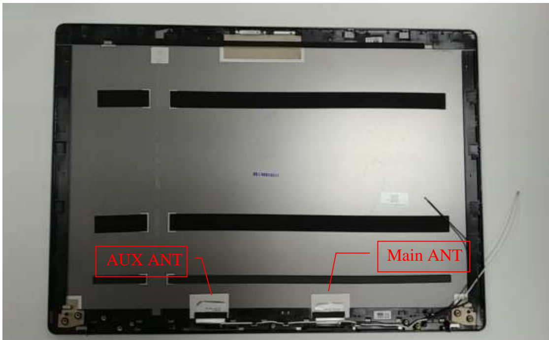
Figure 61 WLAN Combo Antenna Position
