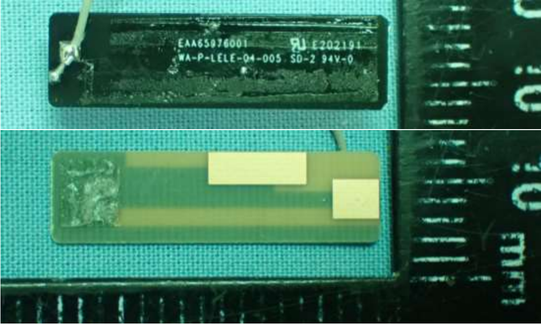
Figure 18 AUX Antenna View)
