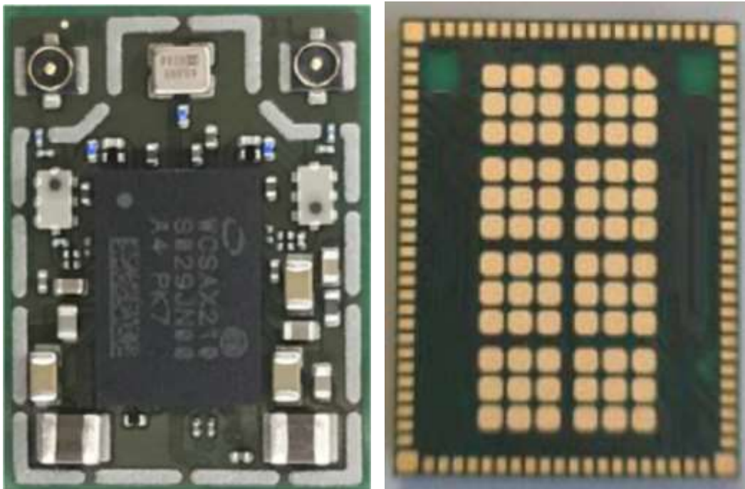
Figure 28 WLAN Combo Card, Without Shield and Back View
