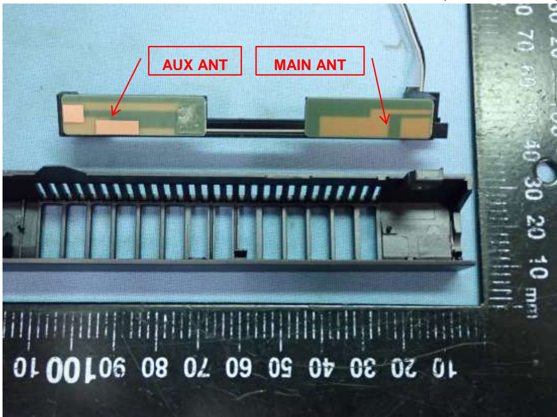
Figure 16 Internal View (Antenna View)
