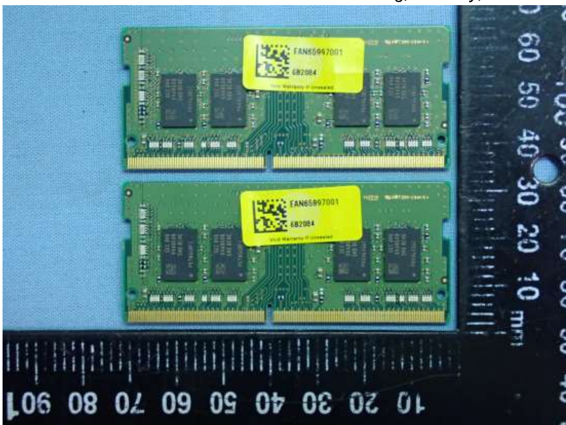
Figure 32 Samsung, Memory, Back View
