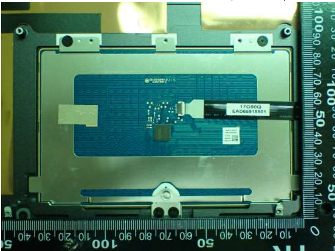
Figure 46 SD081A-36H0, Touch Pad, Back View
