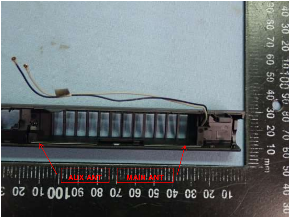
Figure 15 Internal View (Antenna Location)
