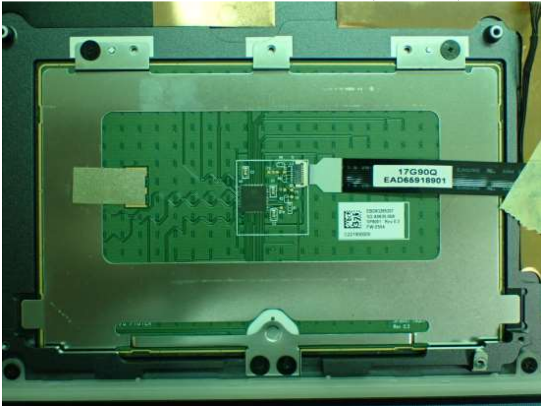
Figure 45 SP8001, Touch Pad, Back View
