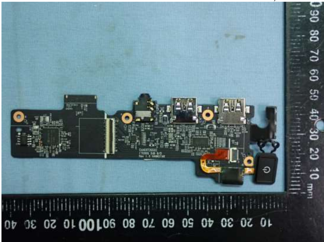
Figure 24 SUB Board, Back View
