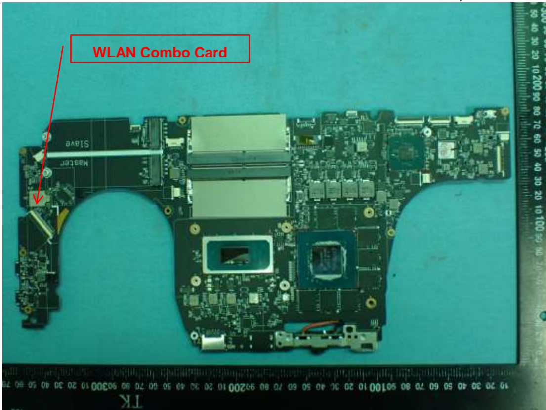
Figure 25 Main Board, Front View
