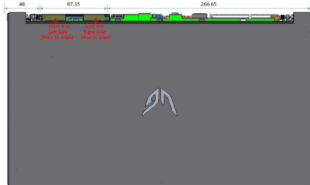
Antenna Location
