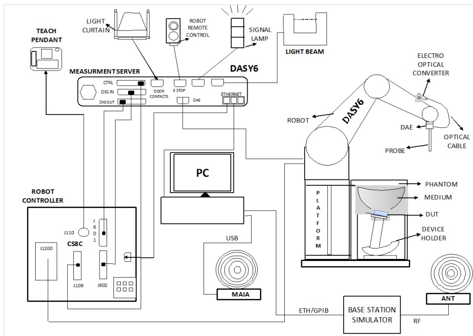
Fig-3.1 DASY6 System Setup
