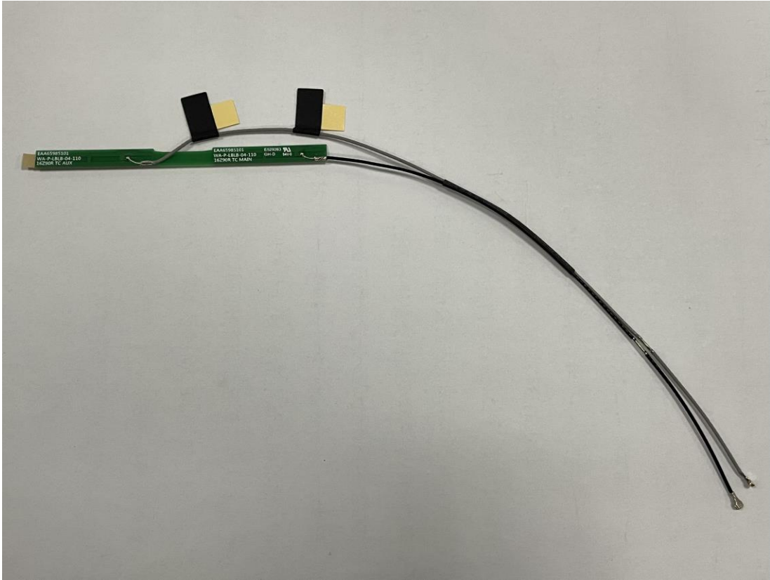
Figure 163 WA-P-LBLB-04-110 WLAN Combo Antenna View
