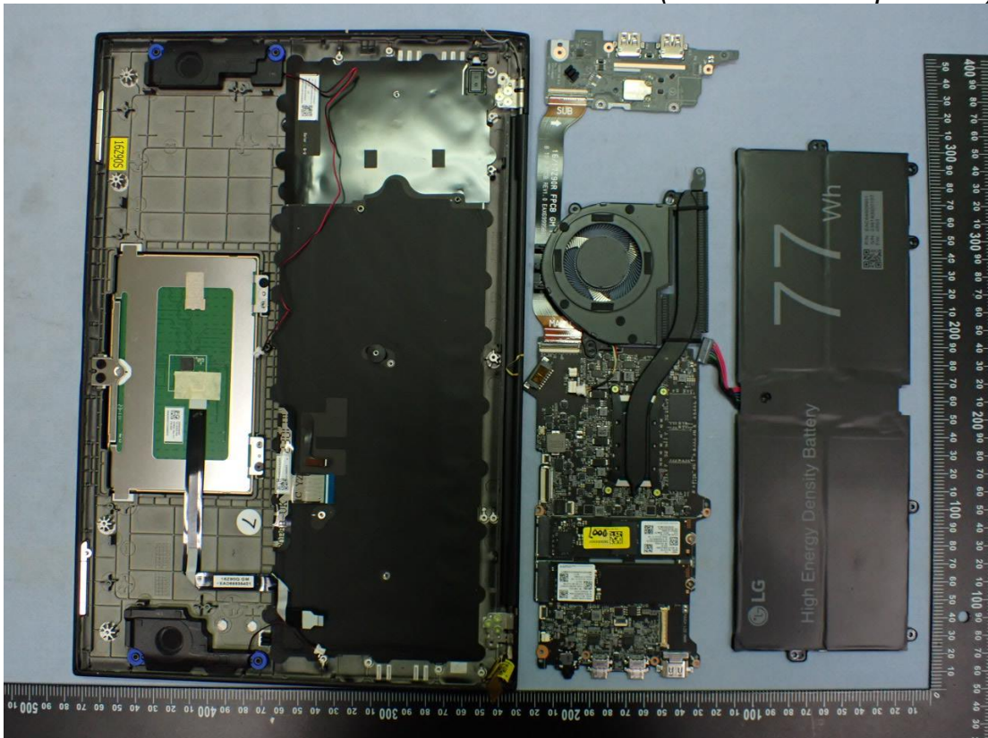
Figure 86 Internal View (Removed Components)
