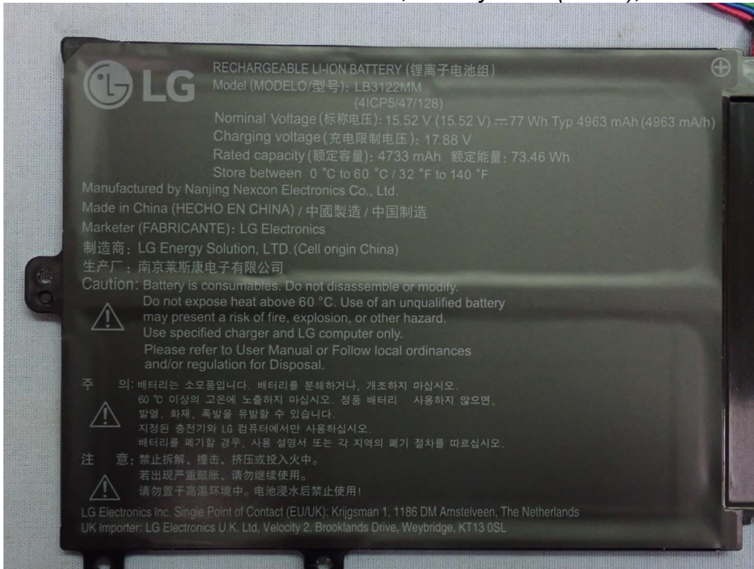
Figure 95 This Time add, Battery Pack (77Wh), Label View
