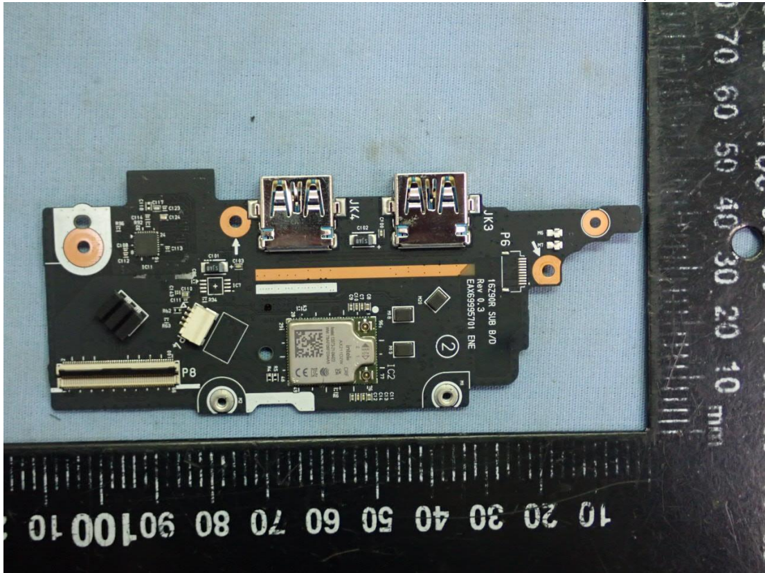
Figure 133 WLAN SUB Board, Front View
