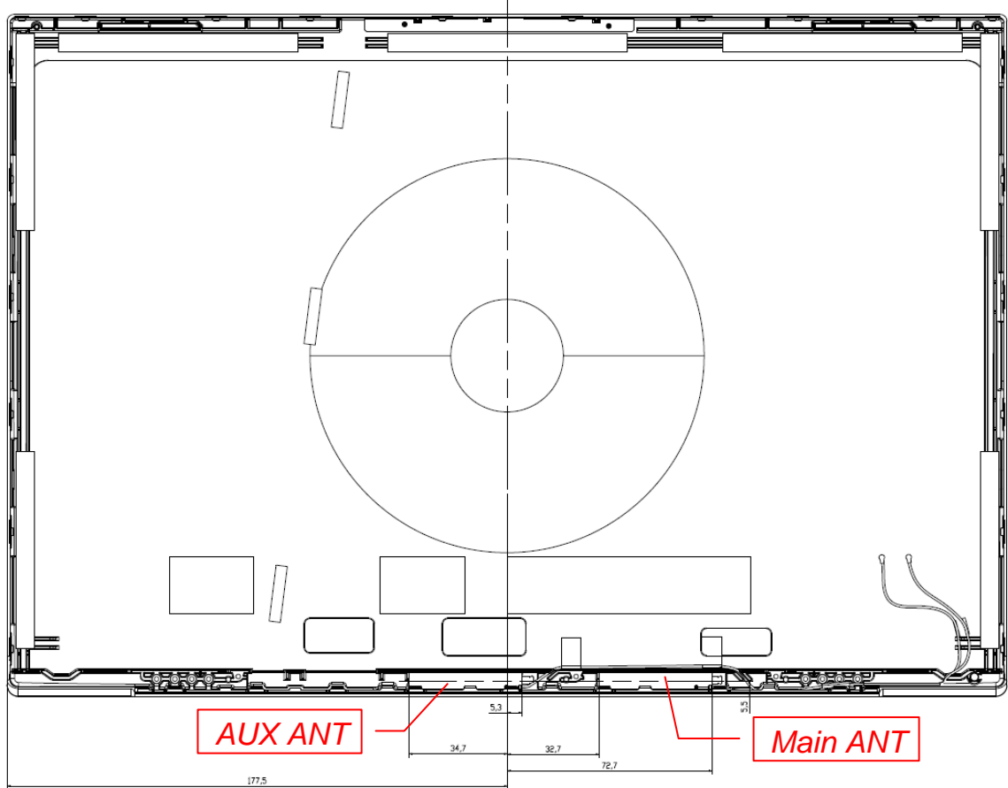
Figure 144 L1LRF008-CS-H, WLAN Combo Antenna Position
