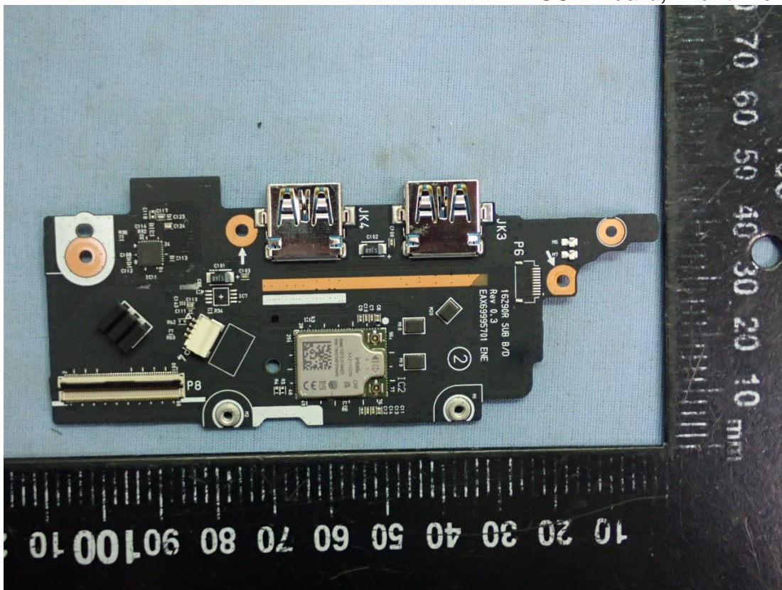
Figure 67 WLAN SUB Board, Front View
