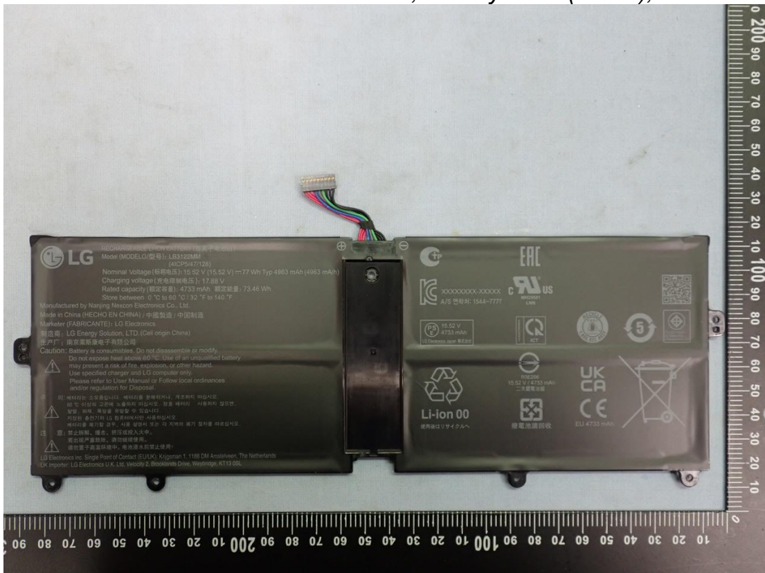
Figure 94 This Time add, Battery Pack (77Wh), Back View
