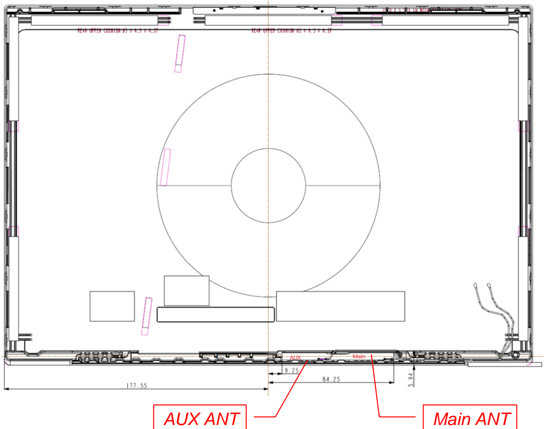
Figure 164 This Time Add WA-P-LBLB-04-110, WLAN Combo Antenna Position
