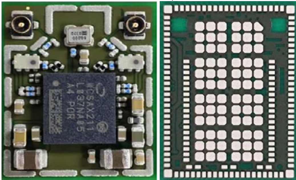
Figure 136 WLAN Combo Card, Without Shield and Back View
