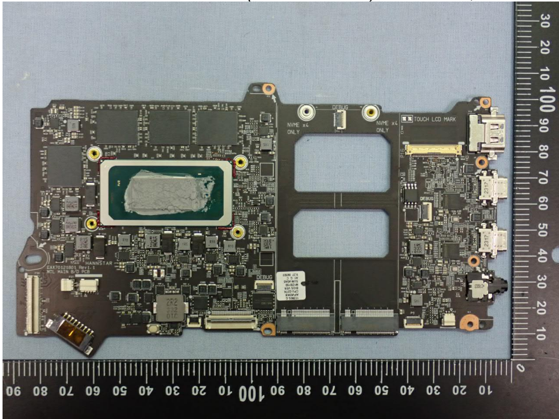
Figure 131 This Time add (MTL MAIN B/D) Main Board, Front View
