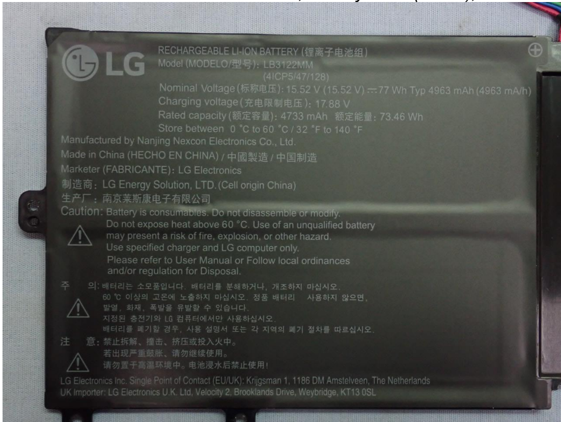
Figure 117 This Time add, Battery Pack (77Wh), Label View
