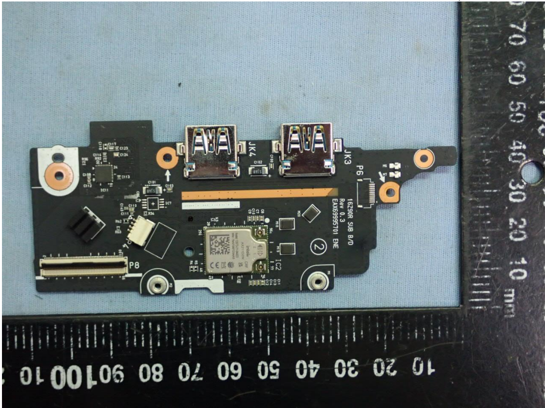
Figure 155 WLAN SUB Board, Front View
