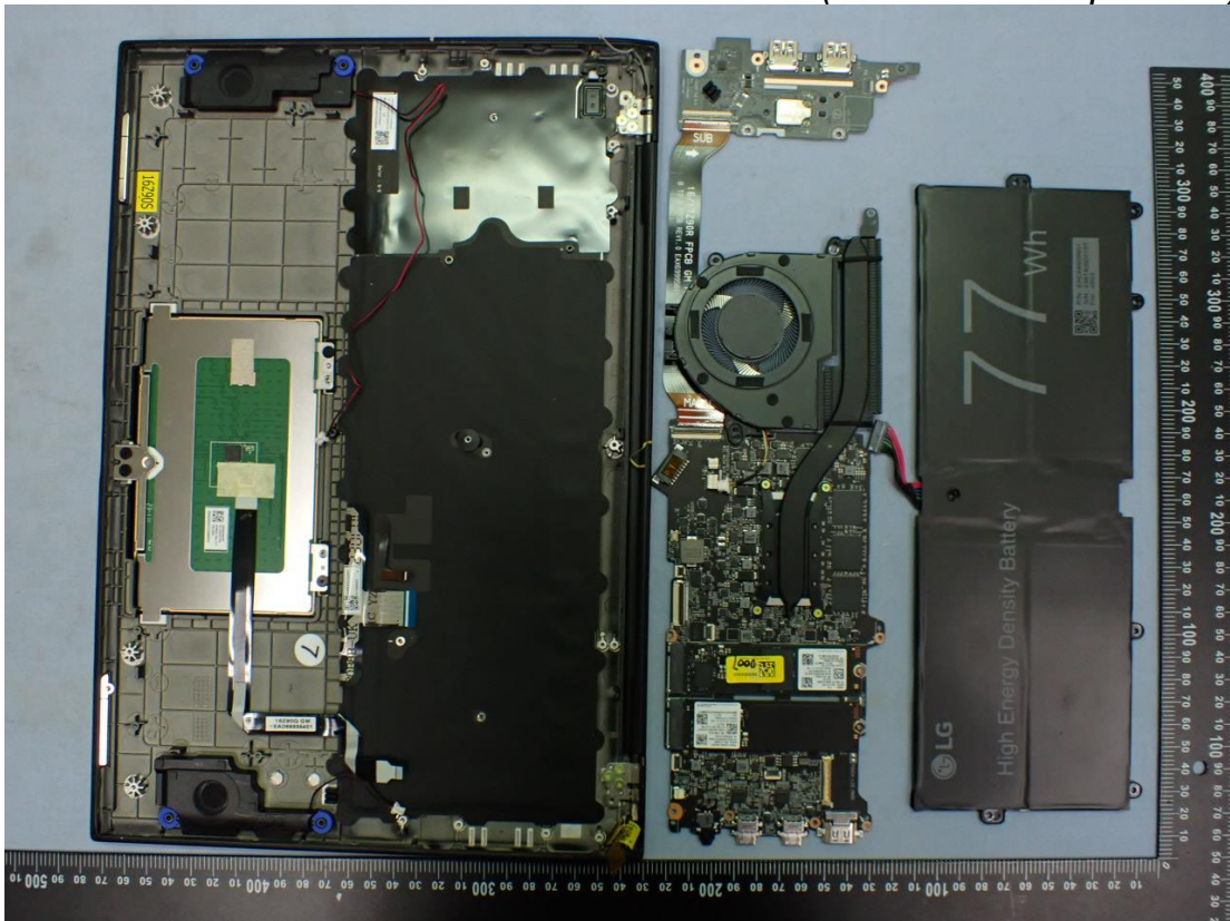
Figure 64 Internal View (Removed Components)
