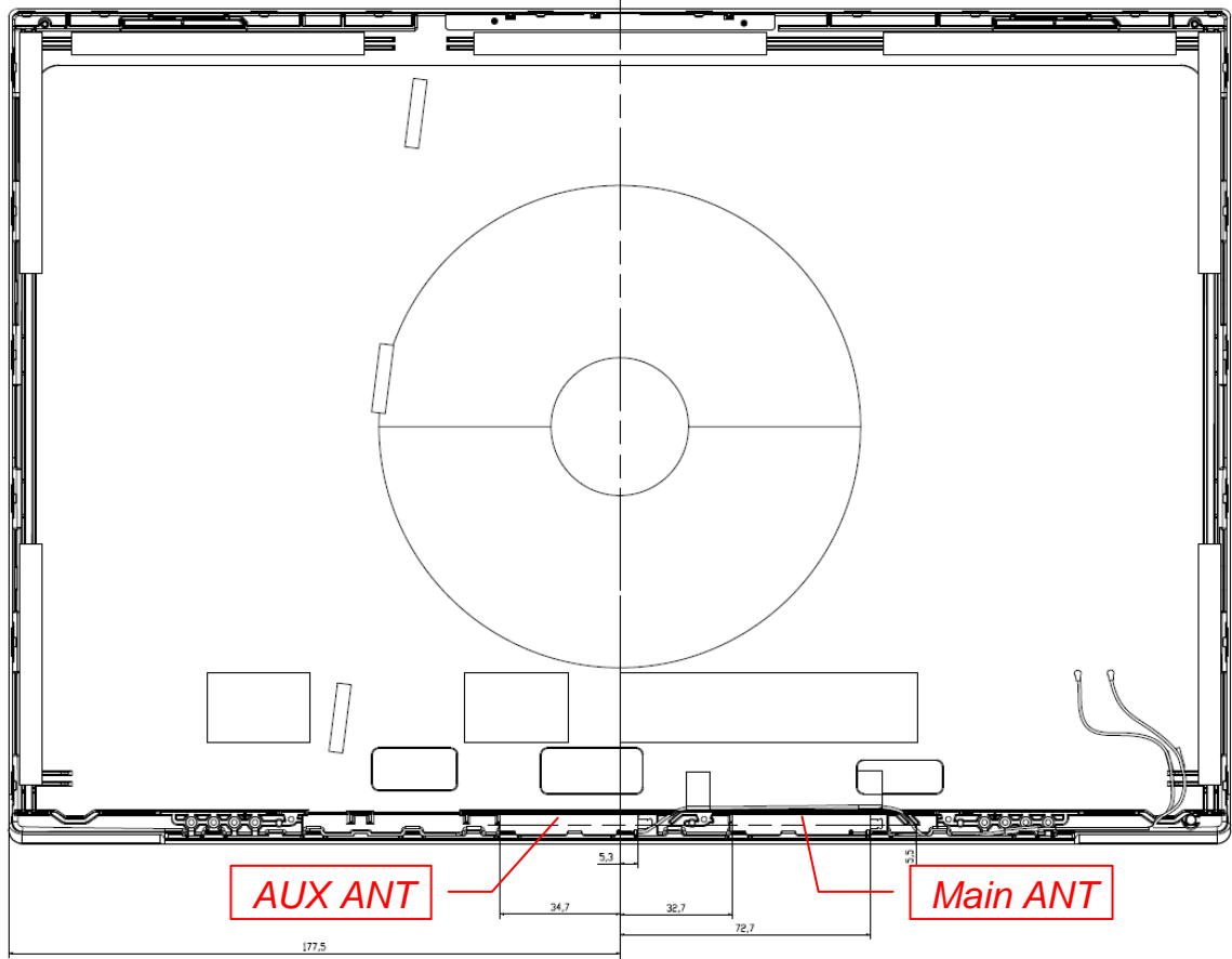
Figure 76 WA-P-LELE-04-009, WLAN Combo Antenna Position
