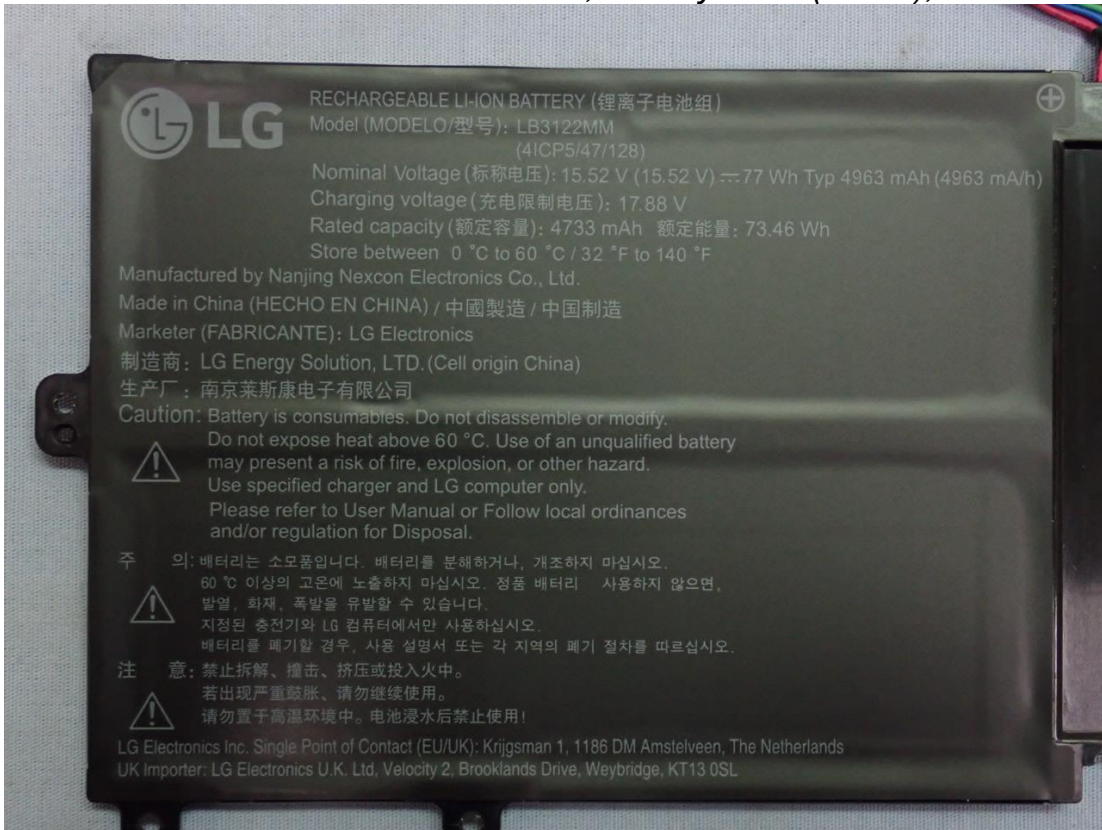
Figure 139 This Time add, Battery Pack (77Wh), Label View
