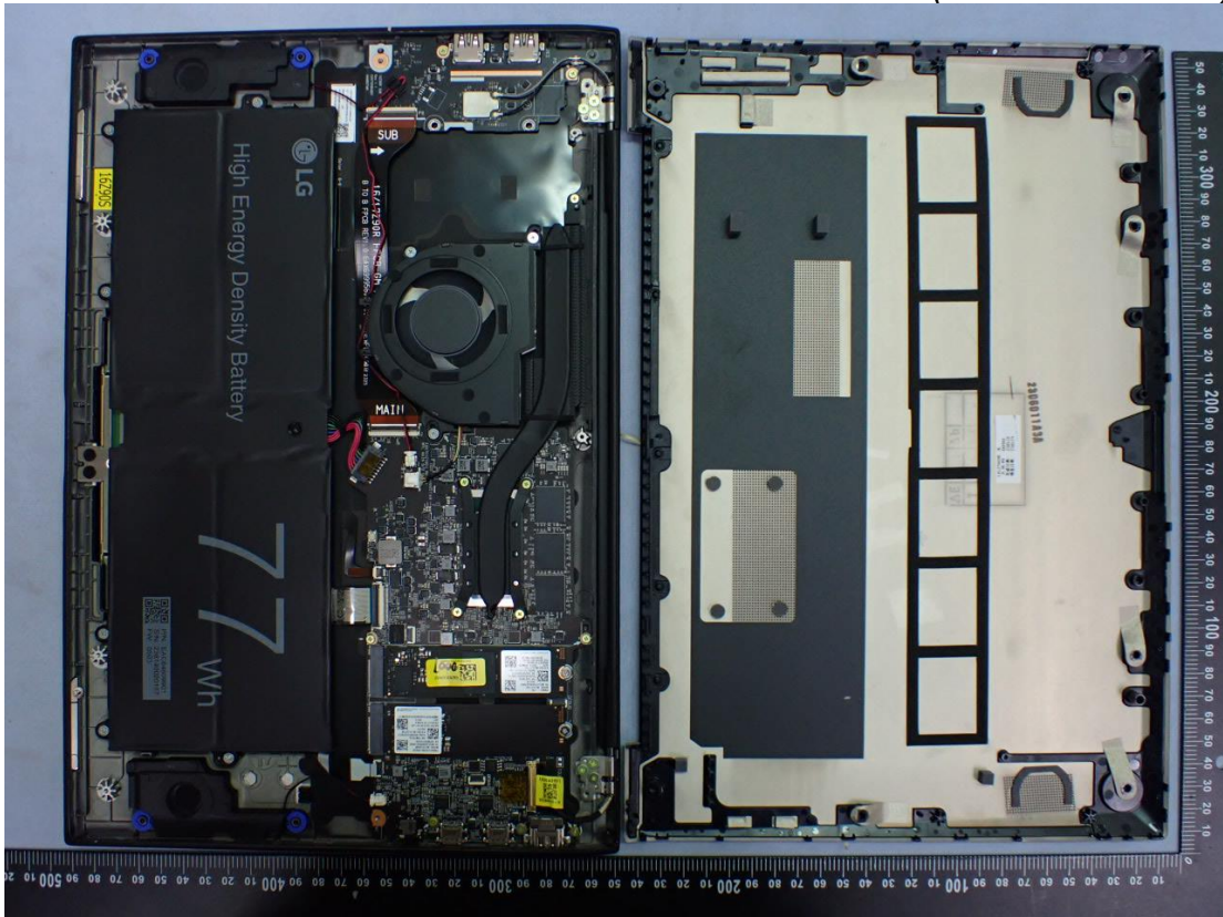
Figure 107 Internal View (Removed Cover)
