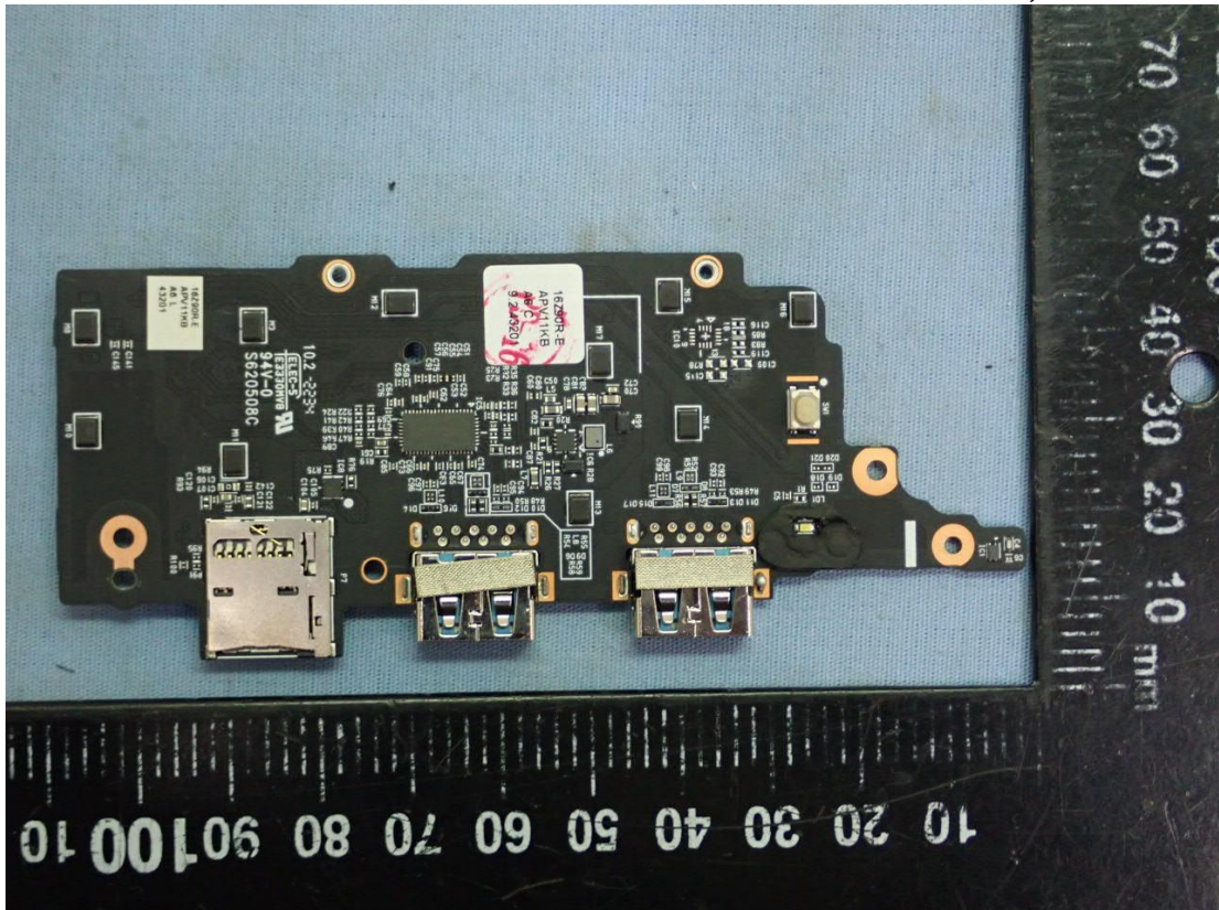
Figure 90 WLAN SUB Board, Back View
