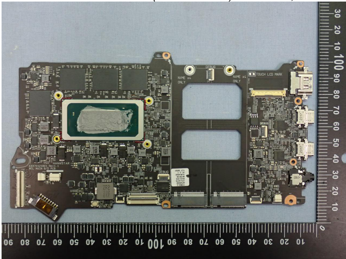
Figure 65 This Time add (MTL MAIN B/D) Main Board, Front View
