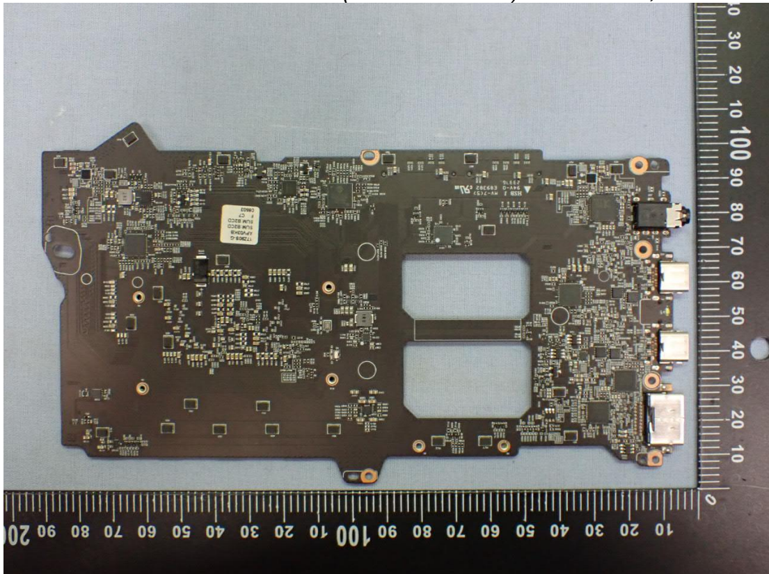
Figure 154 This Time add (MTL MAIN B/D) Main Board, Back View
