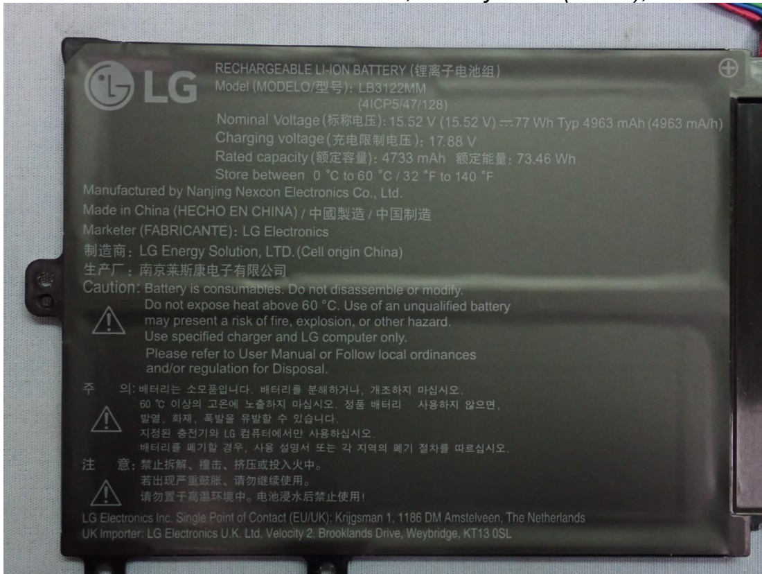
Figure 73 This Time add, Battery Pack (77Wh), Label View
