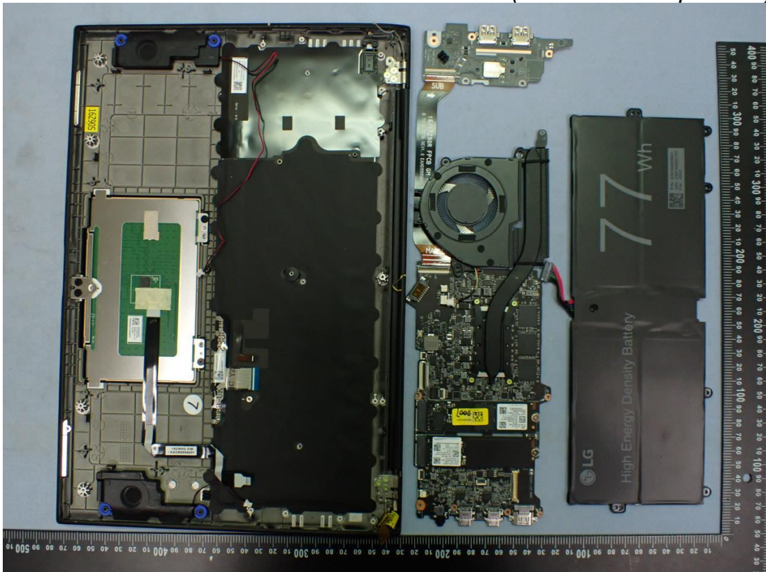
Figure 108 Internal View (Removed Components)
