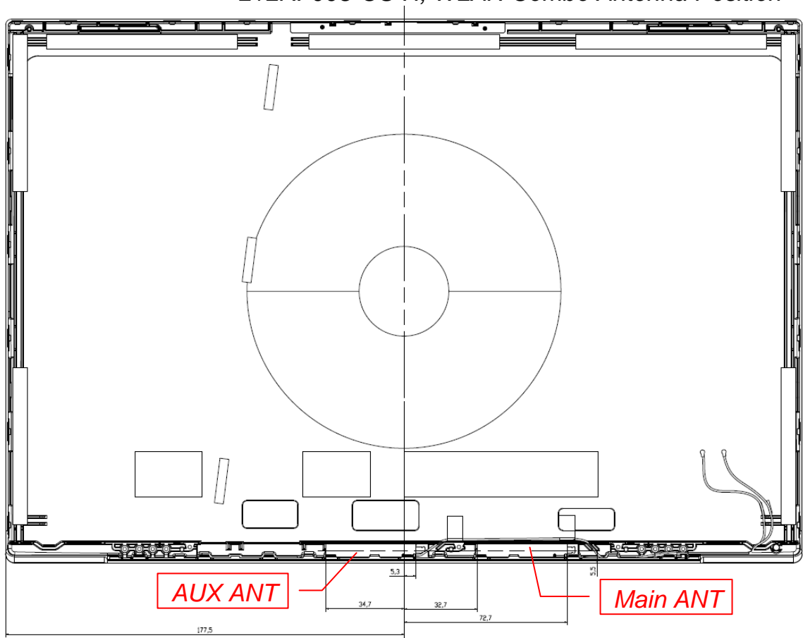
Figure 100 L1LRF008-CS-H, WLAN Combo Antenna Position
