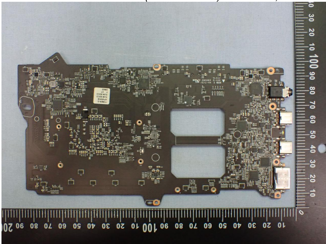
Figure 66 This Time add (MTL MAIN B/D) Main Board, Back View
