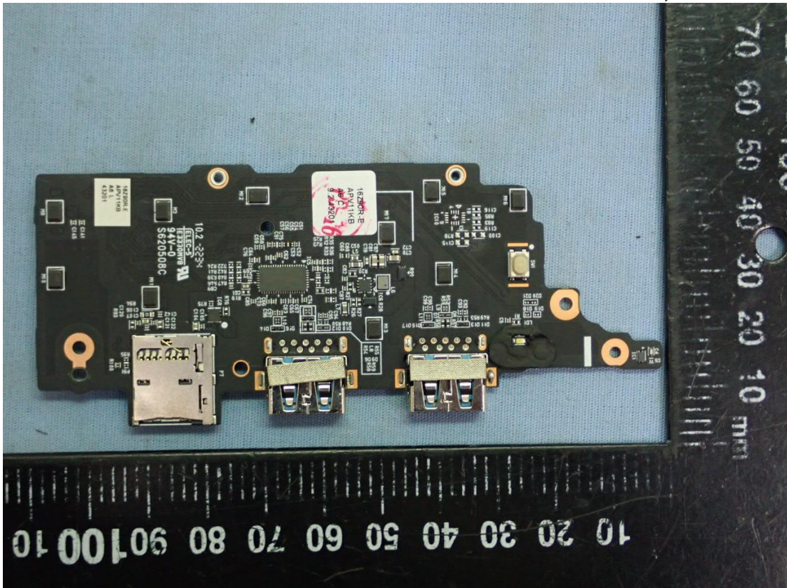
Figure 156 WLAN SUB Board, Back View
