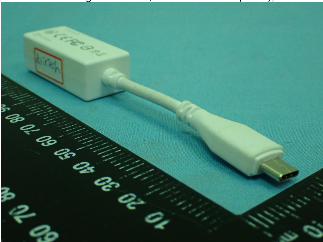
Figure 48 100 Megabit Ethernet, LAN Gender View (White), Front View
