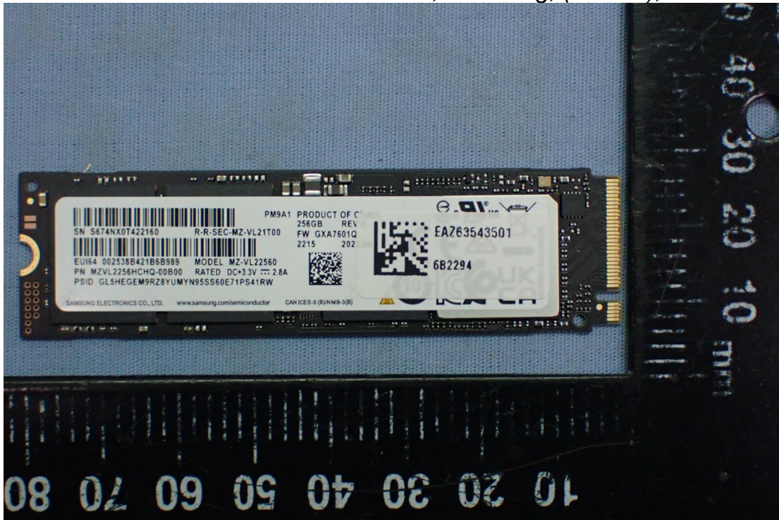
Figure 35 SSD, Samsung, (256GB), Front View
