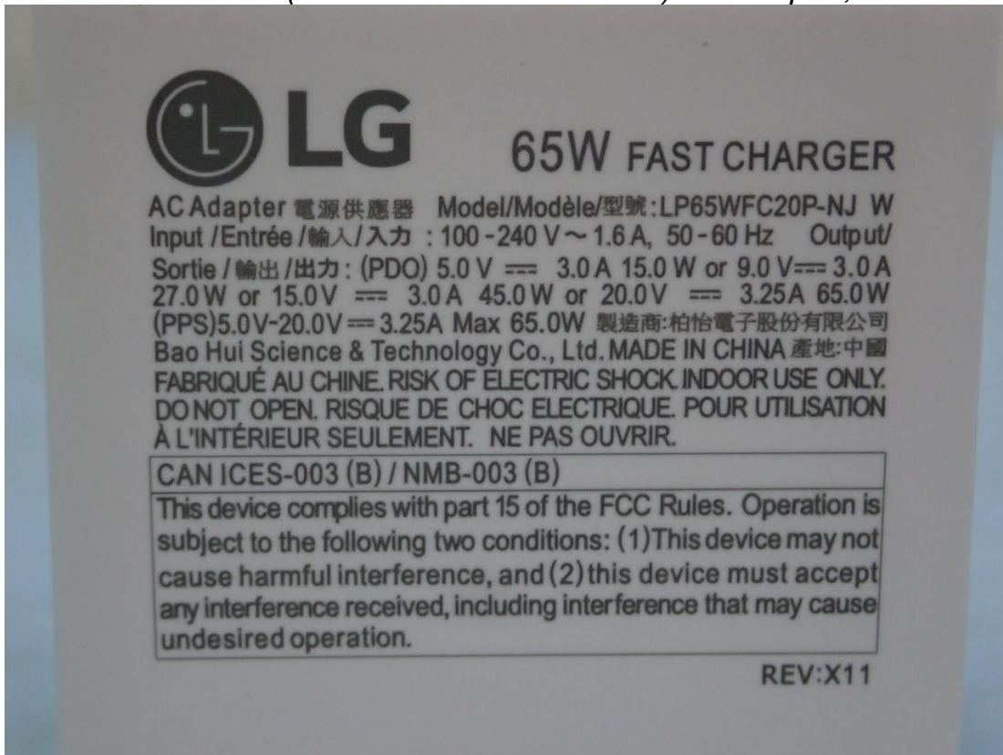
Figure 55 (M/N: LP65WFC20P-NJ W) AC Adapter, Label View
