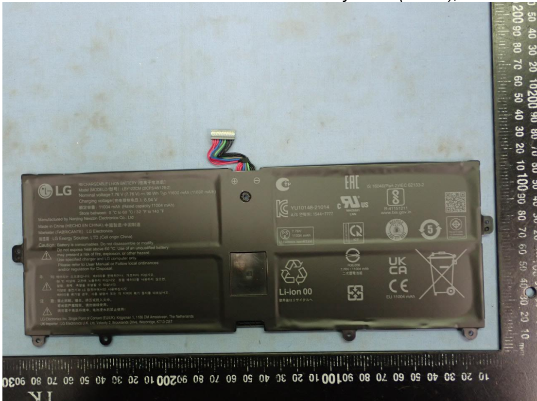
Figure 26 Battery Pack (90Wh), Back View
