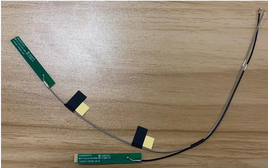
Figure 41 WA-P-LELE-04-009, WLAN Combo Antenna
