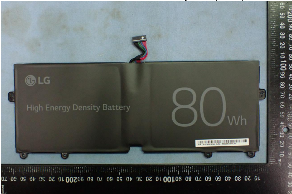
Figure 27 Battery Pack (80Wh), Front View
