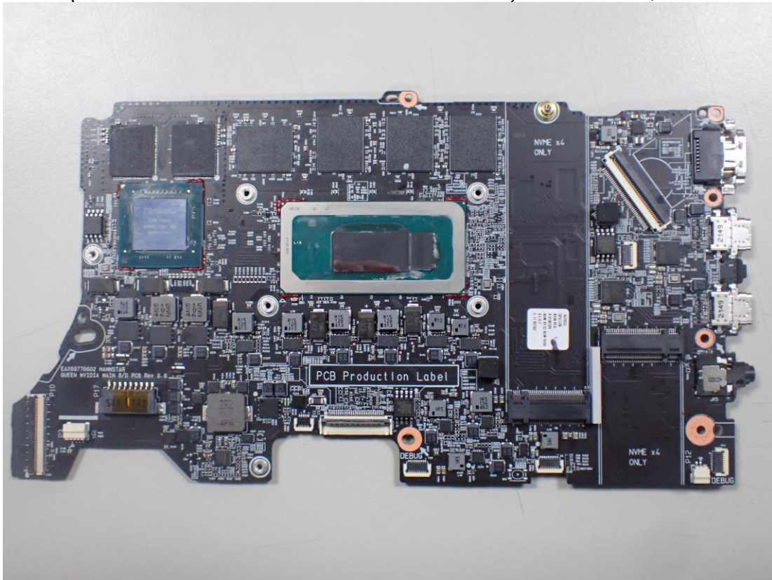
Figure 15 (QUEEN NVIDIA MAIN B/D PCB w/ TPM) Main Board, Front View
