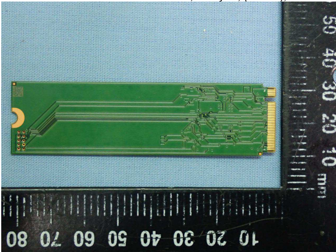
Figure 32 SSD, SK hynix, (512GB), Back View
