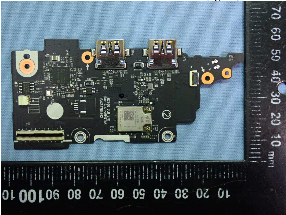
Figure 21 WLAN SUB Board (Type B), Front View
