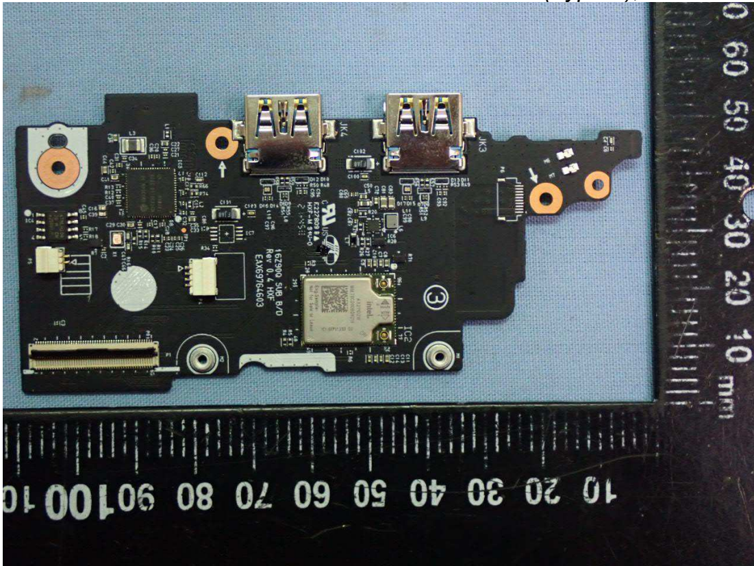
Figure 19 WLAN SUB Board (Type A), Front View
