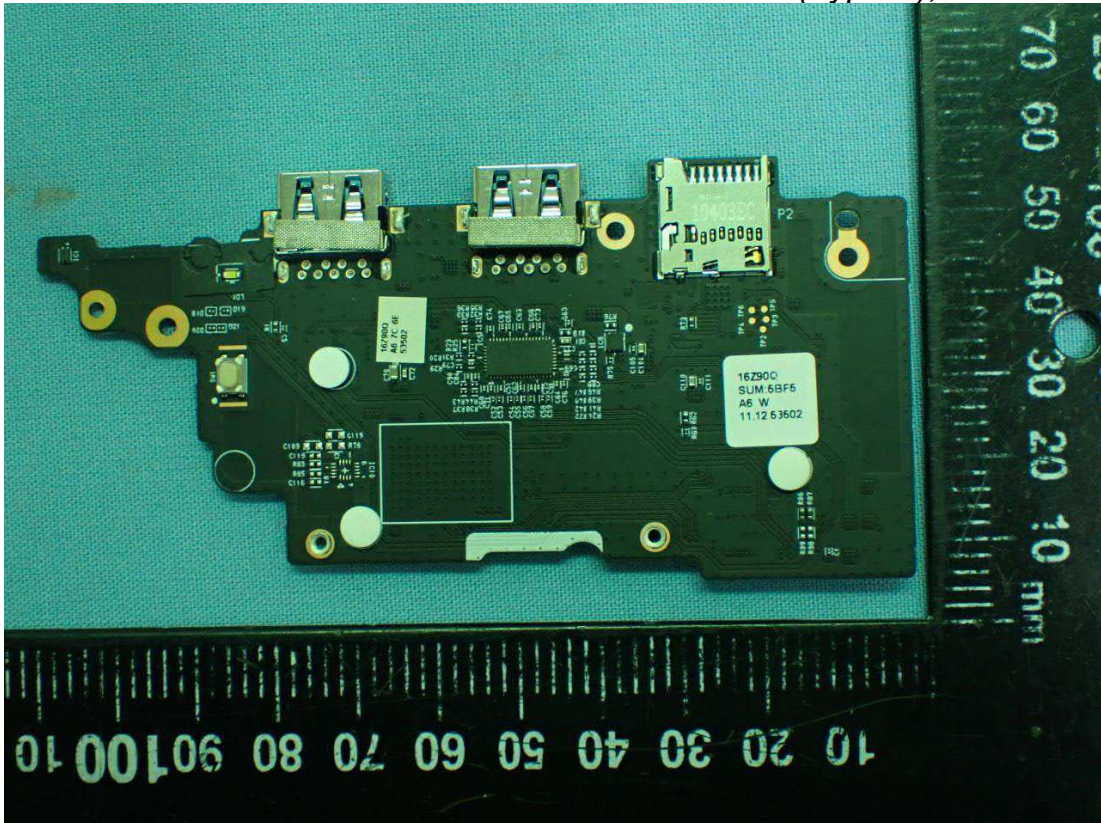
Figure 20 WLAN SUB Board (Type A), Back View
