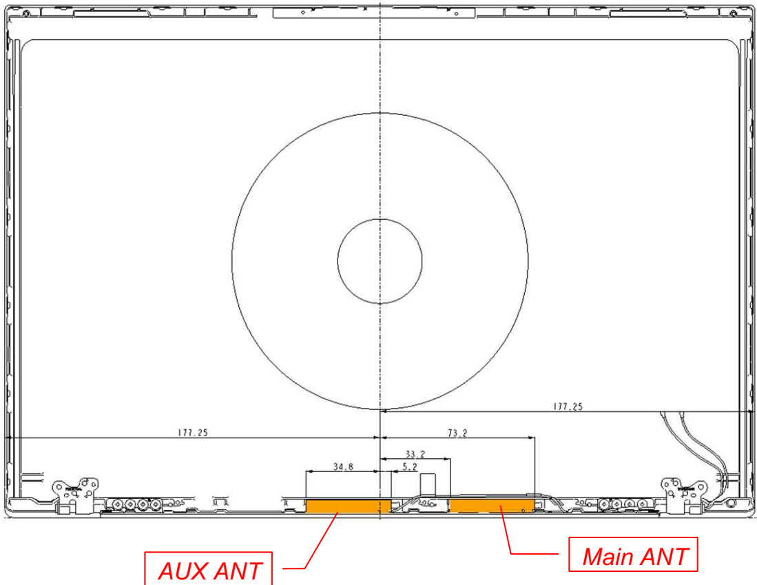
Figure 40 WA-P-LELE-04-009, WLAN Combo Antenna Position
