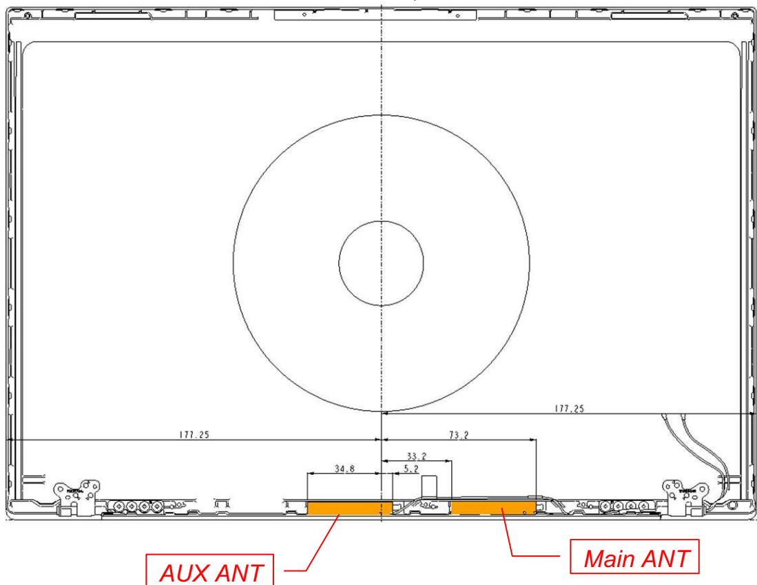
Figure 42 L1LRF008-CS-H, WLAN Combo Antenna Position
