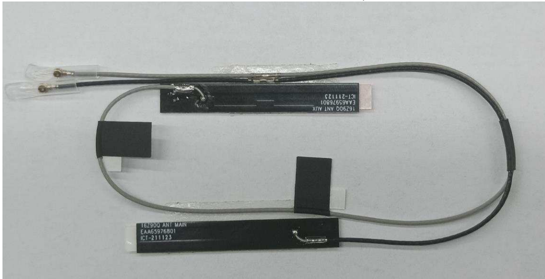
Figure 41 L1LRF008-CS-H, WLAN Combo Antenna
