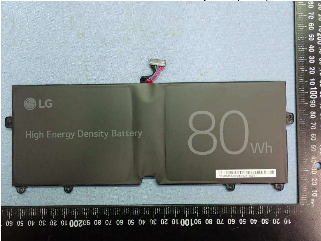
Figure 27 Battery Pack (80Wh), Front View
