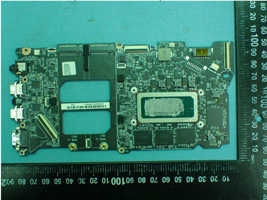
Figure 17 (Queen MAIN B/D PCB) GM Main Board, Front View
