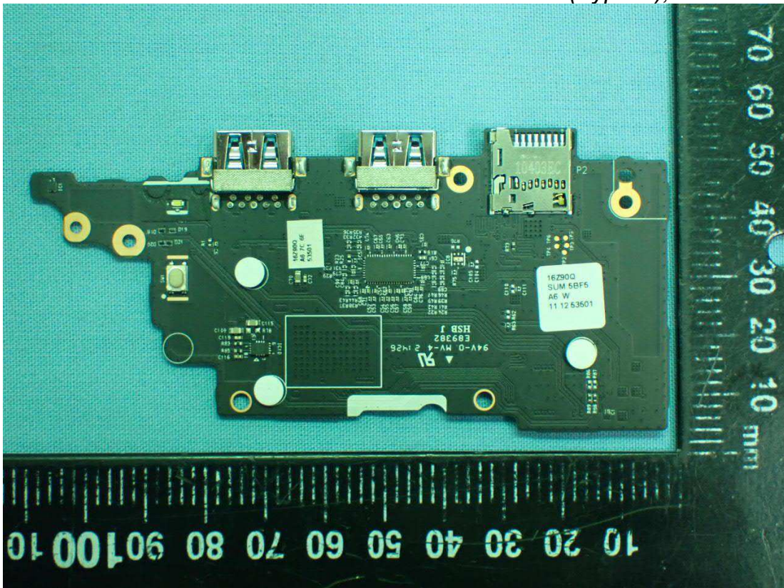
Figure 22 WLAN SUB Board (Type B), Back View
