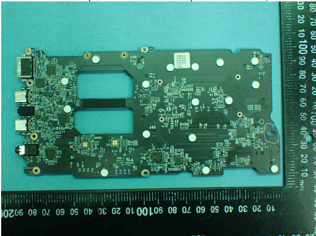
Figure 18 (Queen MAIN B/D PCB) GM Main Board, Back View
