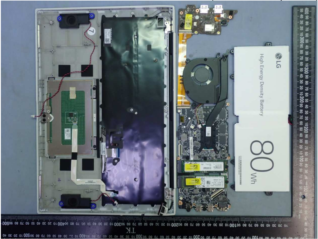
Figure 17 Internal View (Removed Components)
