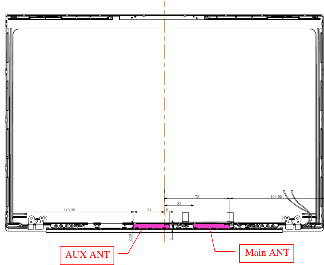
Figure 38 M/N WA-P-LELE-04-002, WLAN Combo Antenna Position
