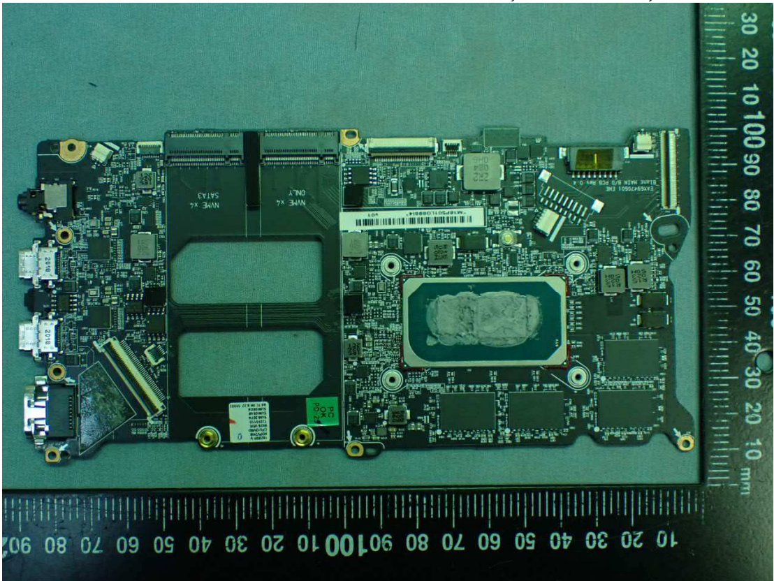
Figure 22 Elec&Eltek, Main Board, Front View
