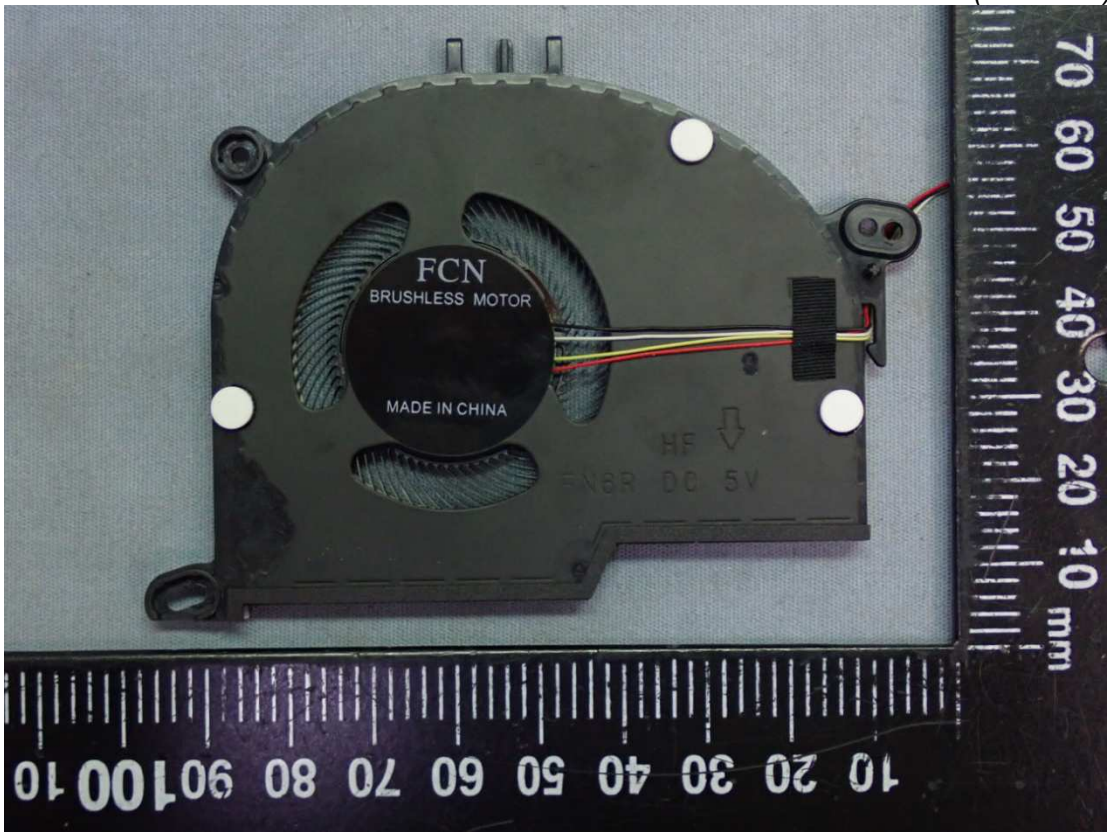
Figure 34 Internal View (DC Fan)
