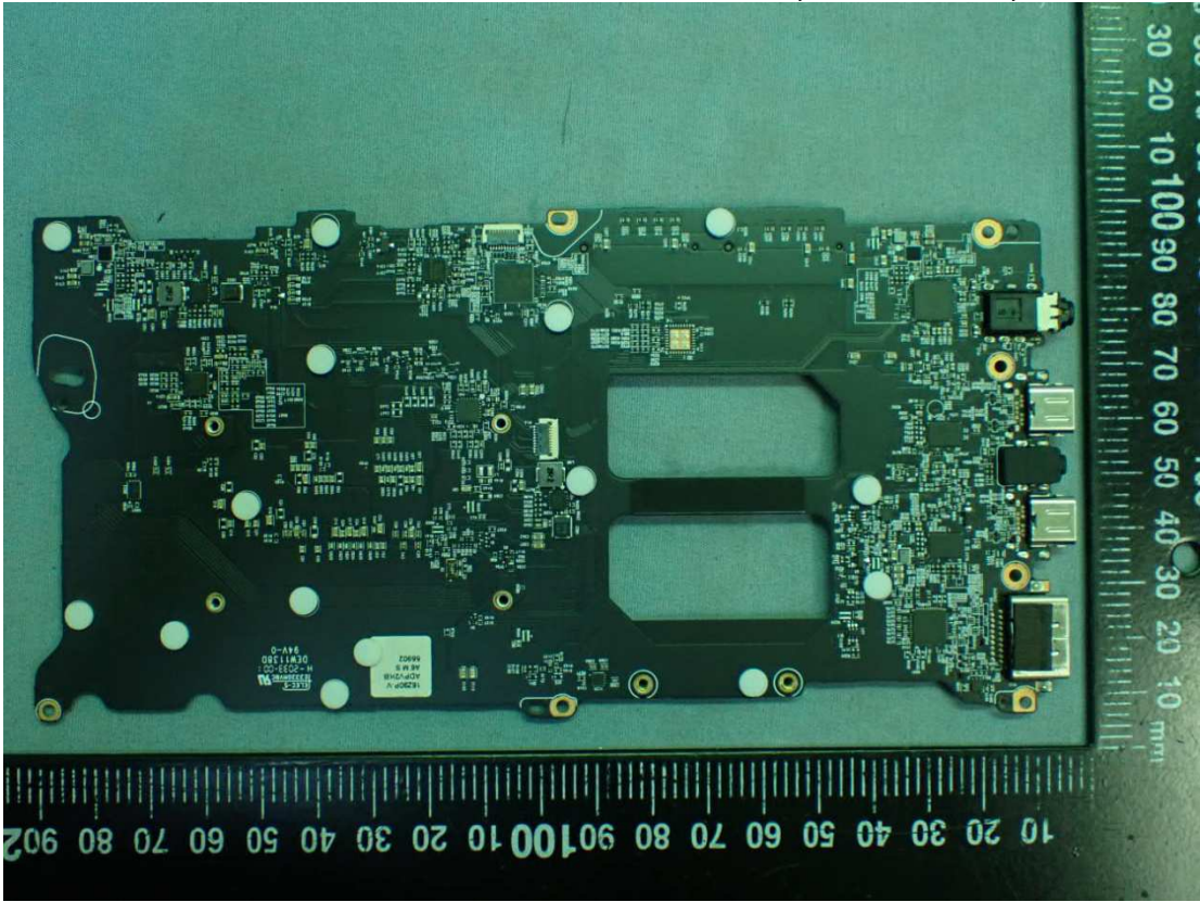
Figure 23 Elec&Eltek, Main Board, Back View
