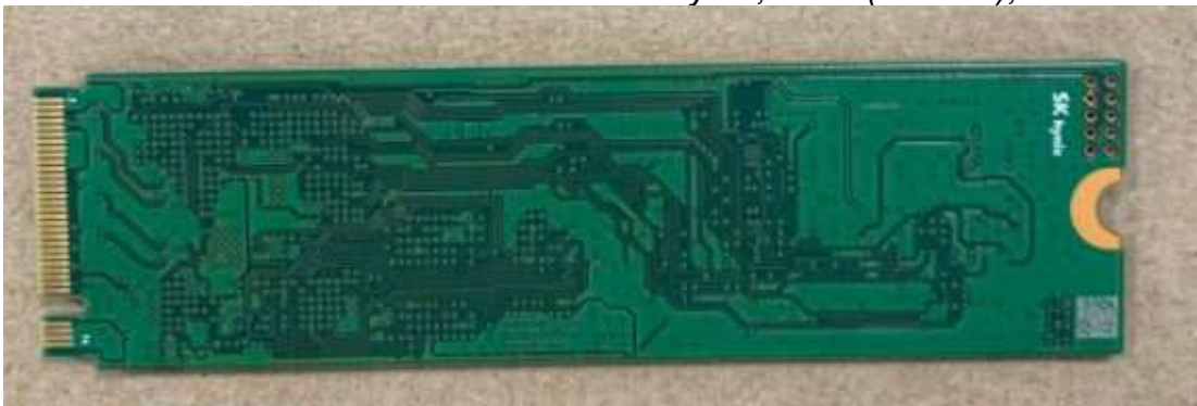
Figure 52 SK hynix, SSD (256GB), Back View
