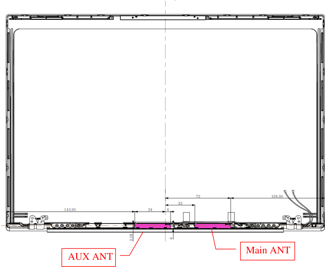
Figure 40 M/N L1LRF004-CS-H, WLAN Combo Antenna Position
