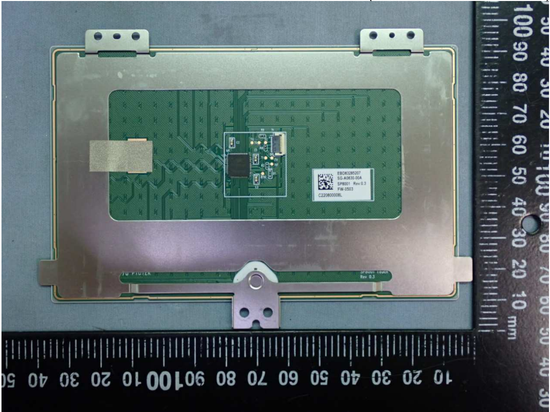
Figure 18 Internal View (Touch Pad, Back View)
