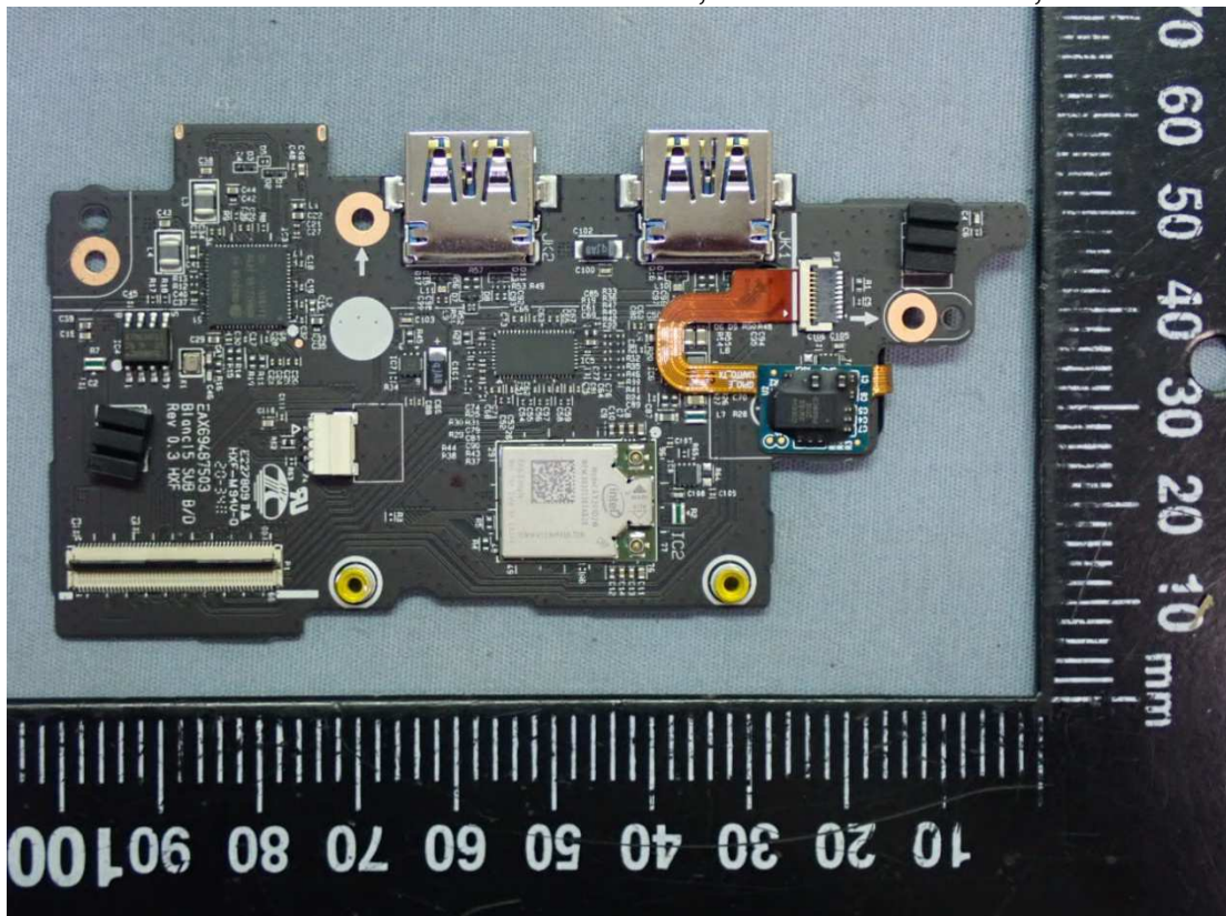
Figure 28 HXF, WLAN SUB Board, Front View
