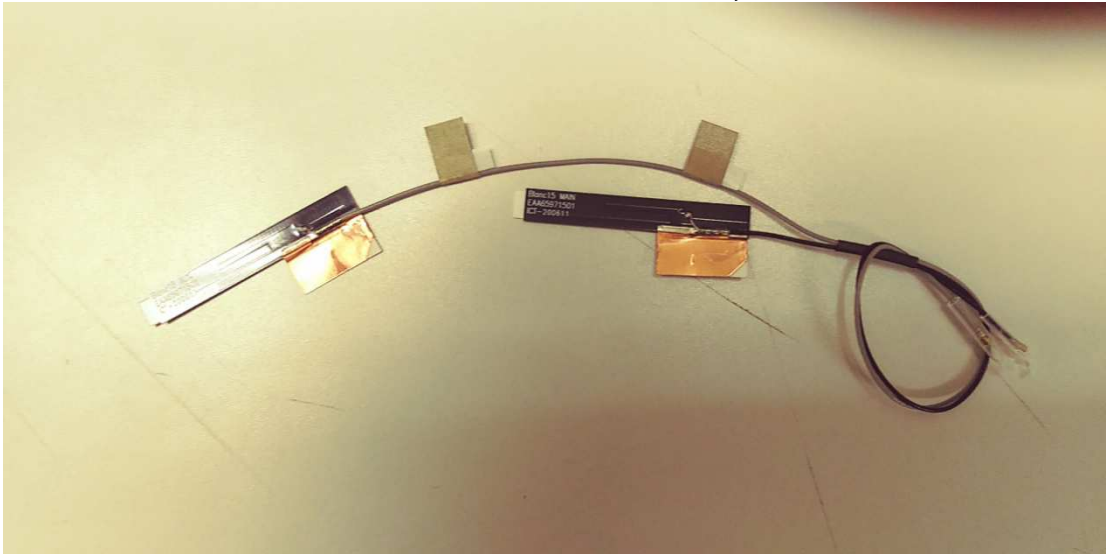
Figure 39 M/N L1LRF004-CS-H, WLAN Combo Antenna
