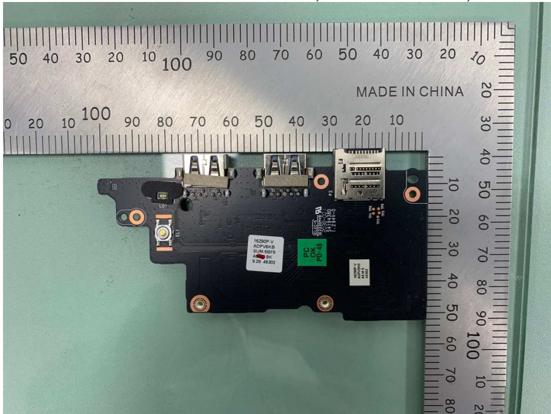
Figure 31 Elec&Eltek, WLAN SUB Board, Back View
