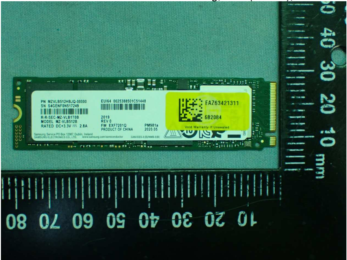
Figure 43 Samsung, SSD (512GB), Front View
