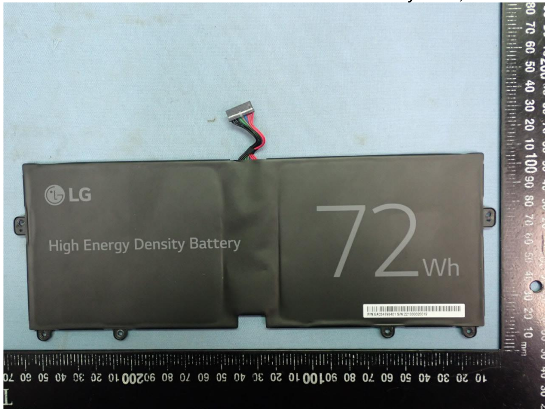
Figure 34 Battery Pack, Front View
