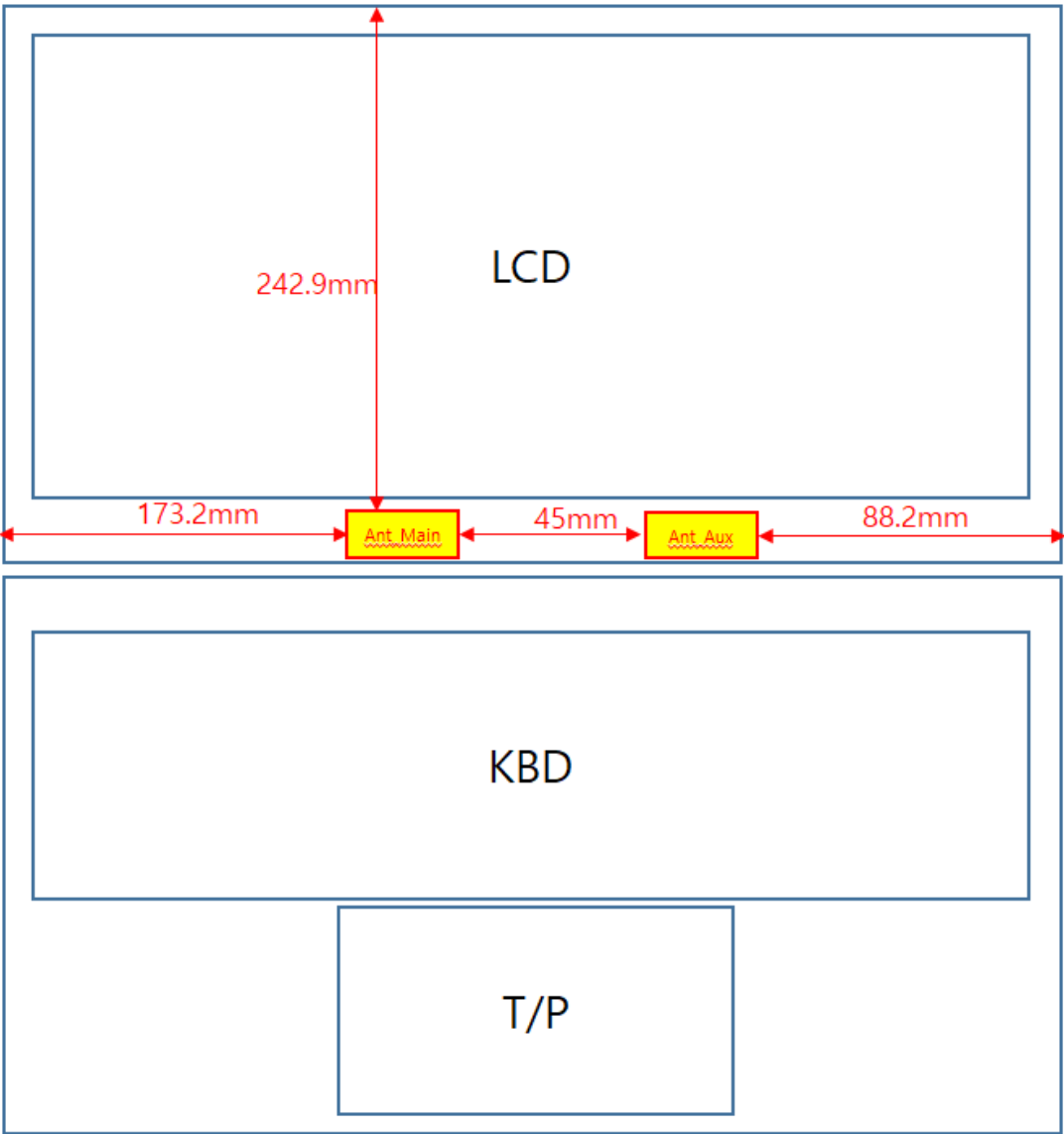
Figure 19 Internal View (Antenna Location)
