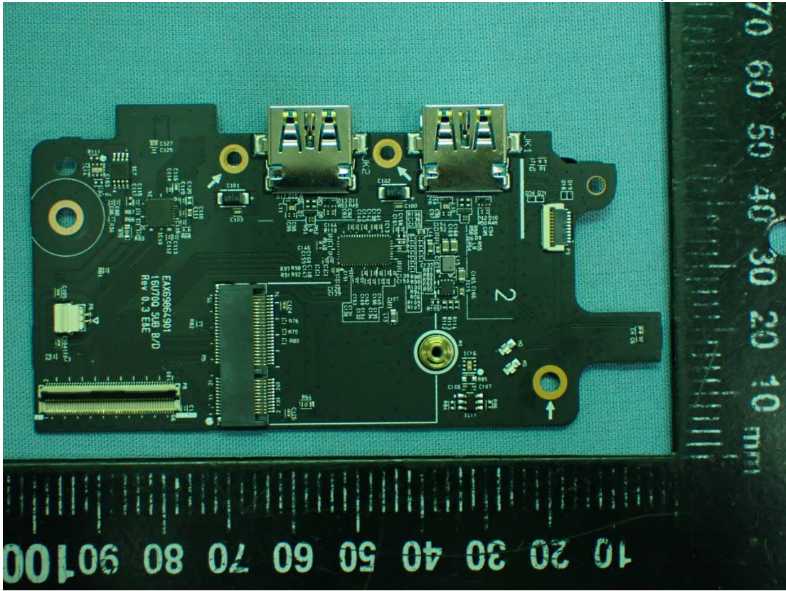
Figure 24 SUB Board, Front View
