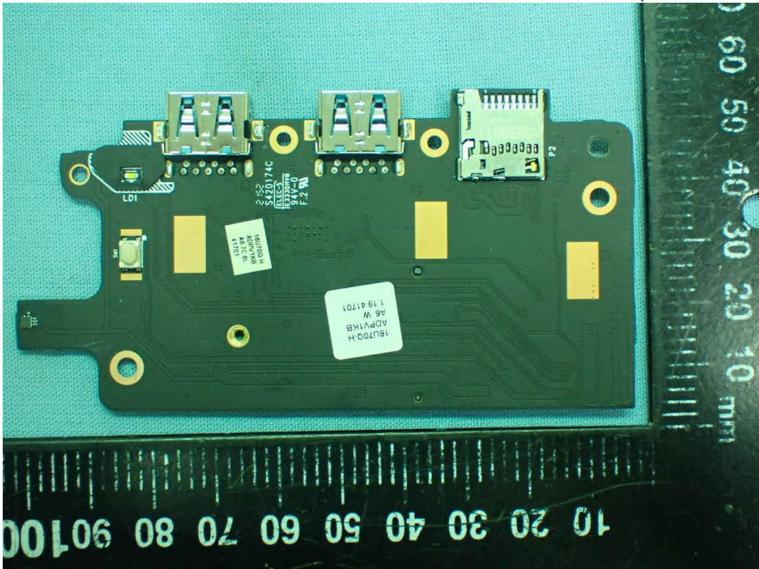
Figure 25 SUB Board, Back View
