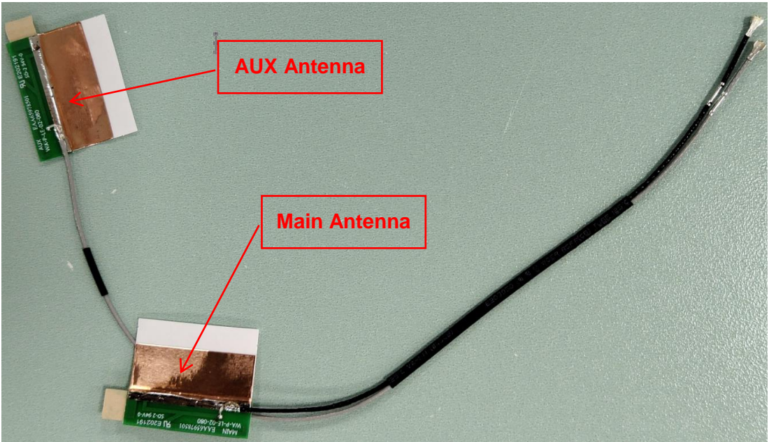
Figure 20 Antenna View, Front View
