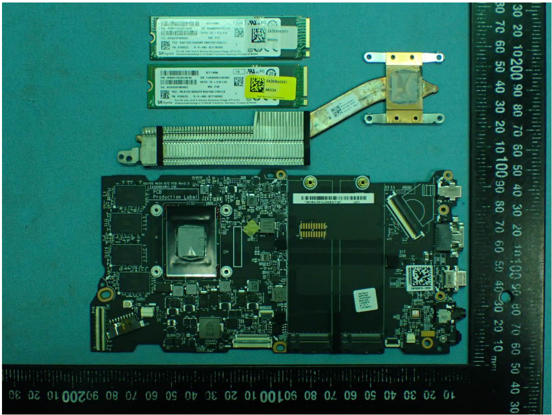
Figure 17 Internal View
