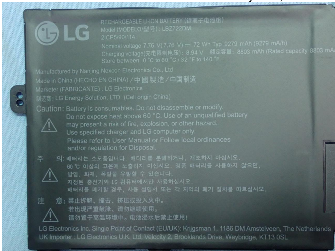
Figure 36 Battery Pack, Label View
