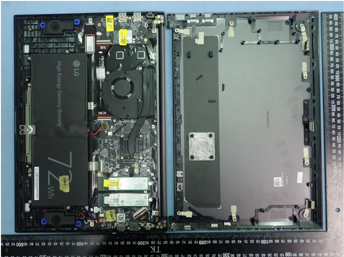
Figure 15 Internal View
