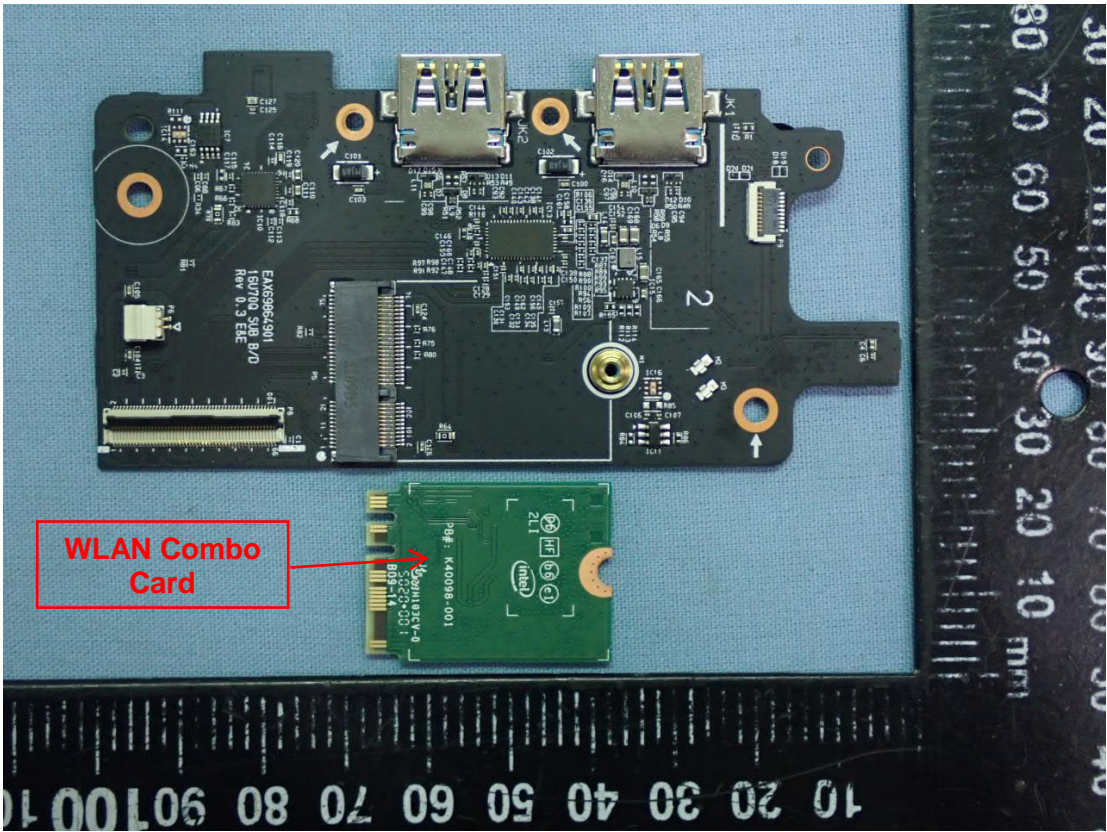
Figure 18 Internal View
