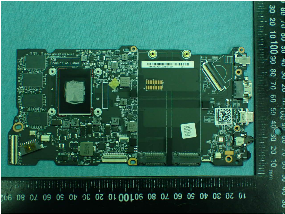
Figure 22 Main Board, Front View
