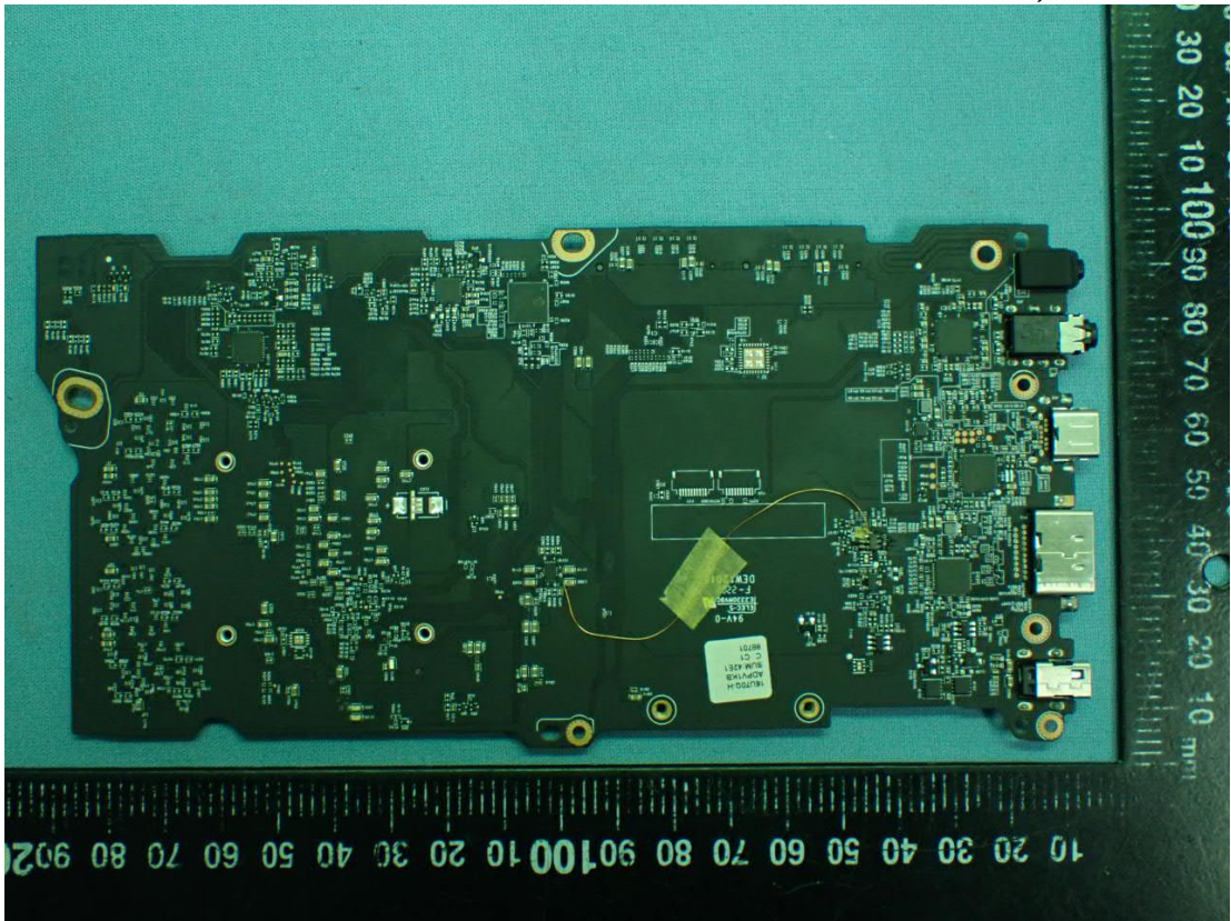
Figure 23 Main Board, Back View
