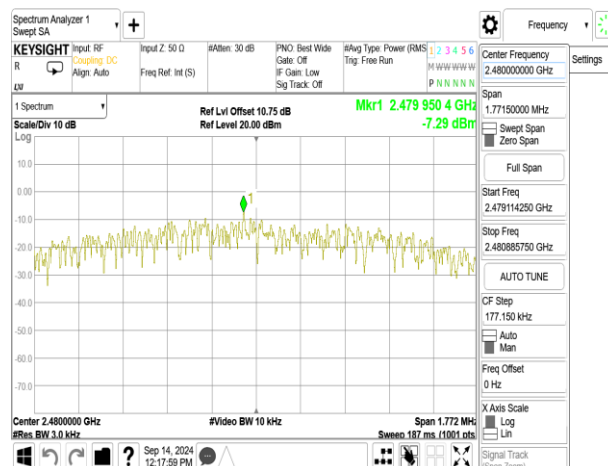
PSD_BLE 2M_HighCH39-2480MHz
