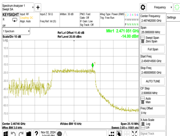
802.11ax_20MHz_ChainA_2462MHz_RU106_54
