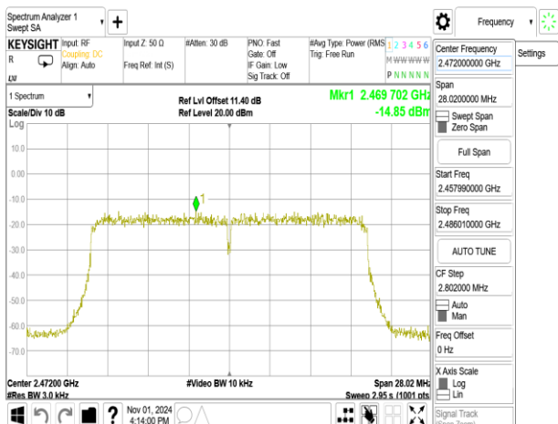
802.11ax_20MHz_ChainA_2472MHz_RU106_54
