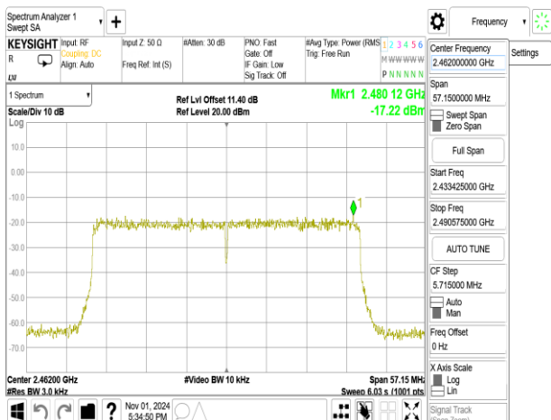
802.11ax_40MHz_ChainA_2462MHz_RU242_62
