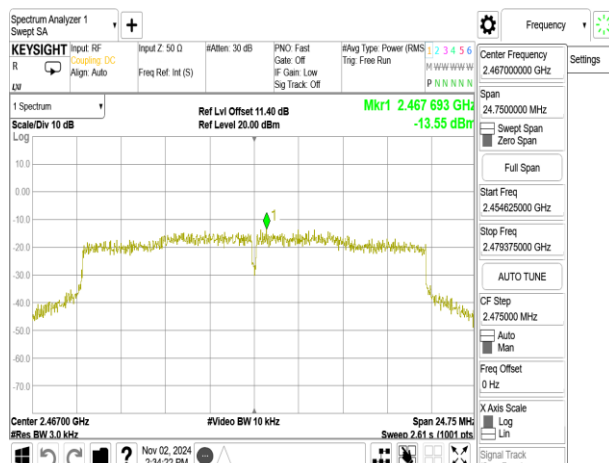
802.11ax_20MHz_ChainA_2467MHz
