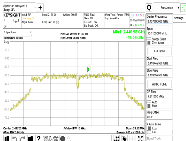
802.11n_40MHz_ChainA_2437MHz
