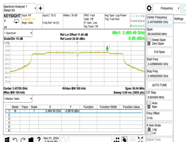
802.11ax_40MHz_ChainA_2457MHz
