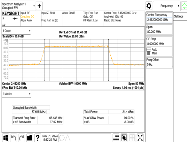
802.11ax_40MHz_ChainA_2462MHz_RU242_62
