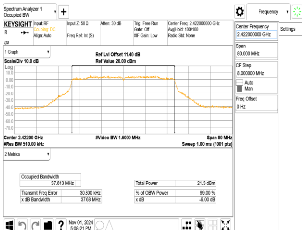
802.11ax_40MHz_ChainA_2422MHz_RU242_61
