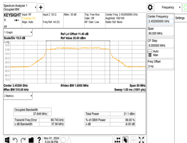
802.11ax_40MHz_ChainA_2452MHz_RU242_62
