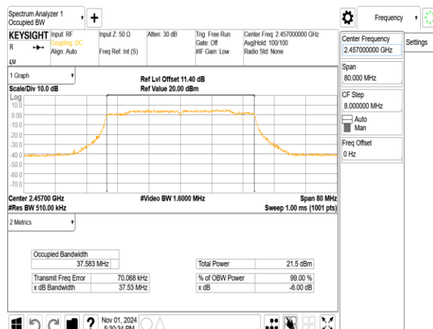
802.11ax_40MHz_ChainA_2457MHz
