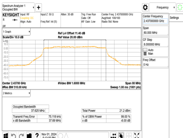
802.11ax_40MHz_ChainA_2437MHz
