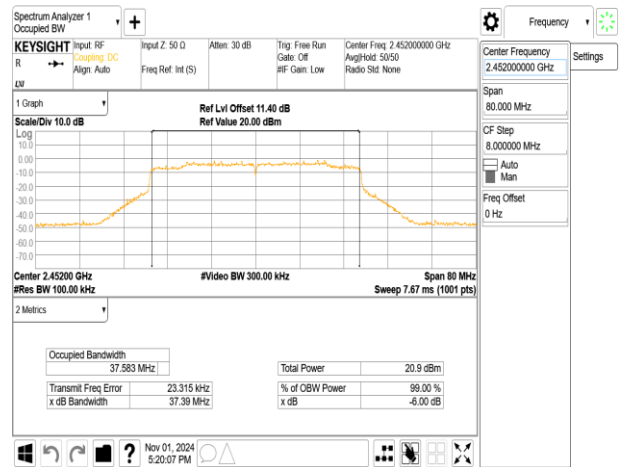
802.11ax_40MHz_ChainA_2452MHz_RU242_62
