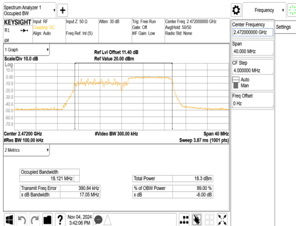
802.11ax_20MHz_ChainA_2472MHz_RU26_8
