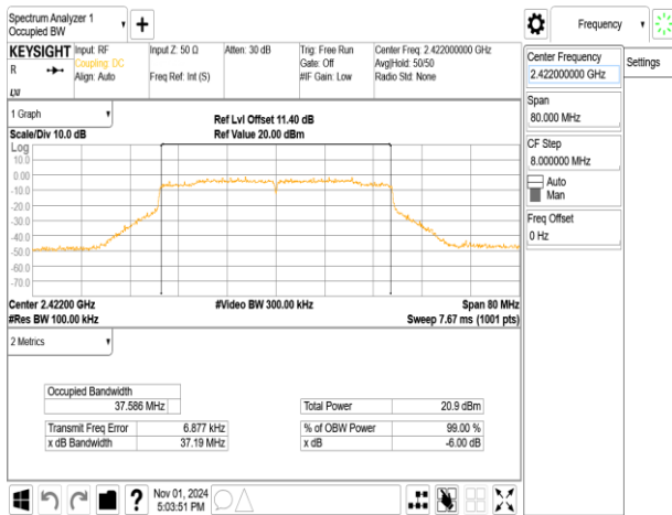
802.11ax_40MHz_ChainA_2422MHz_RU242_61
