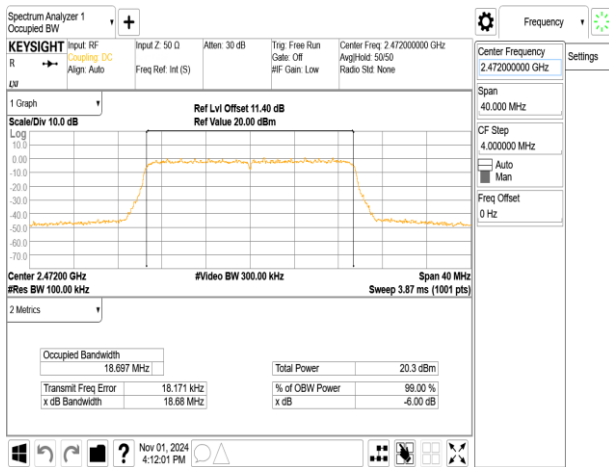
802.11ax_20MHz_ChainA_2472MHz_RU106_54
