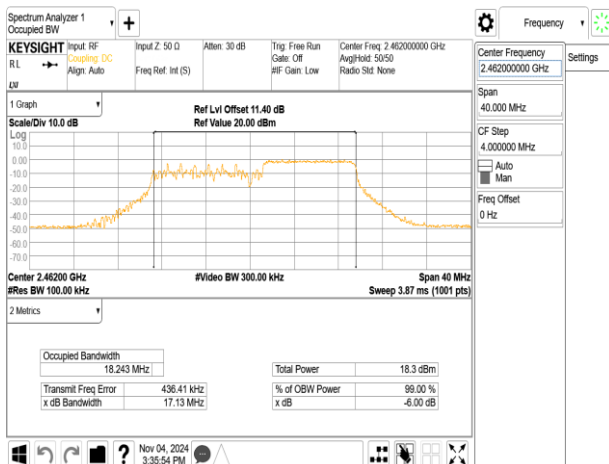
802.11ax_20MHz_ChainA_2462MHz_RU106_54
