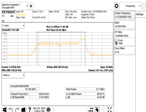
802.11ax_20MHz_ChainA_2472MHz_RU26_8
