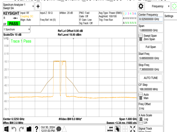
802.11be_160MHz_ChainA_6345MHz_996+484+242_MRU7
