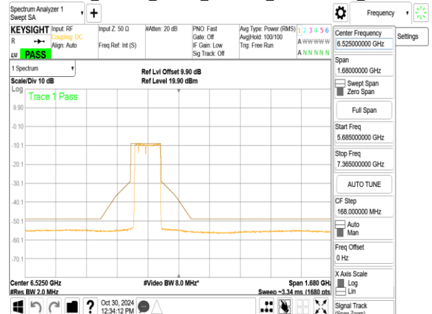
802.11be_160MHz_ChainA_6345MHz_996+484+242_MRU1
