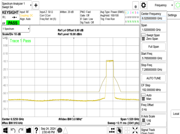
802.11be_80MHz_ChainB_6945MHz_484+242_MRU2
