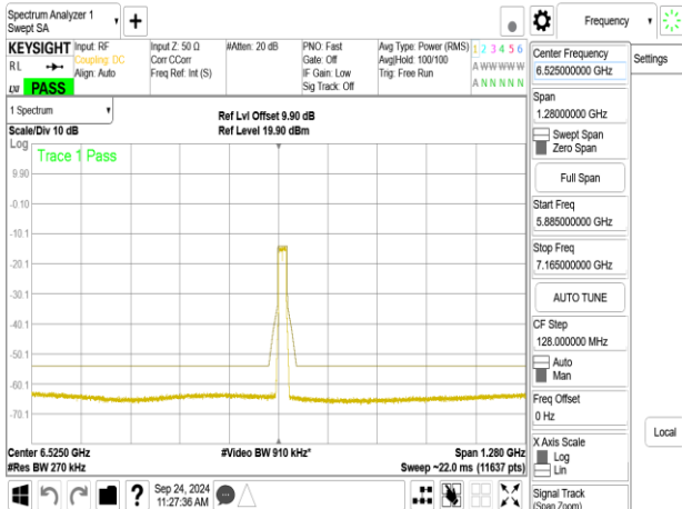
802.11be_20MHz_ChainB_6535MHz_106+26_MR1
