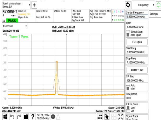
802.11be_20MHz_ChainA_6415MHz_106+26_MRUG
