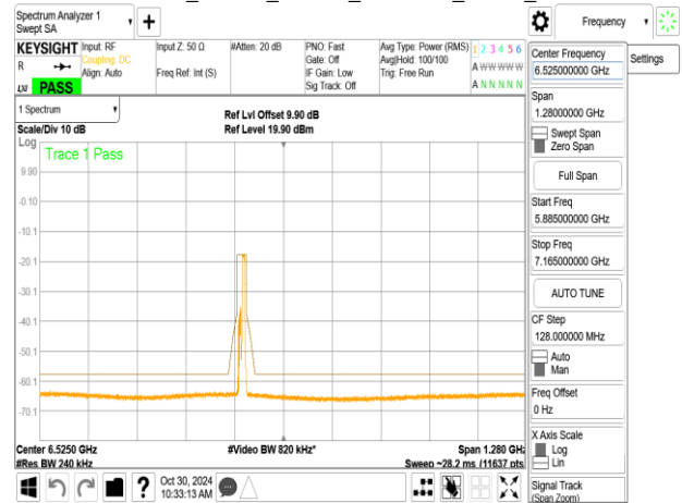
802.11be_20MHz_ChainA_6415MHz_RU106_54
