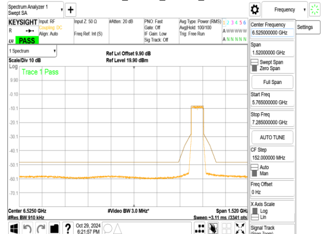
802.11ax_80MHz_ChainA_6945MHz
