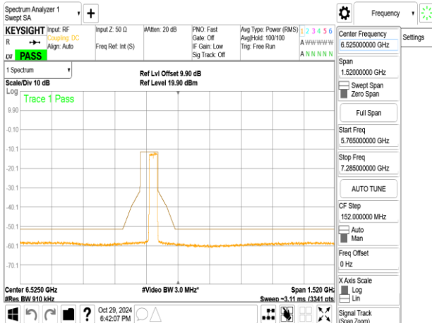
802.11ax_80MHz_ChainB_6465MHz
