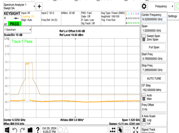
802.11ax_80MHz_ChainB_6145MHz
