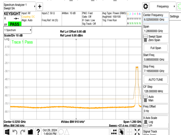
802.11ax_20MHz_ChainB_7115MHz_RU106_54
