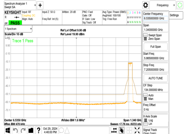
802.11ax_40MHz_ChainA_7085MHz_RU242_62
