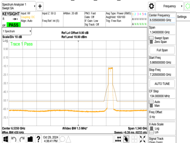
802.11ax_40MHz_ChainB_6845MHz_RU242_62
