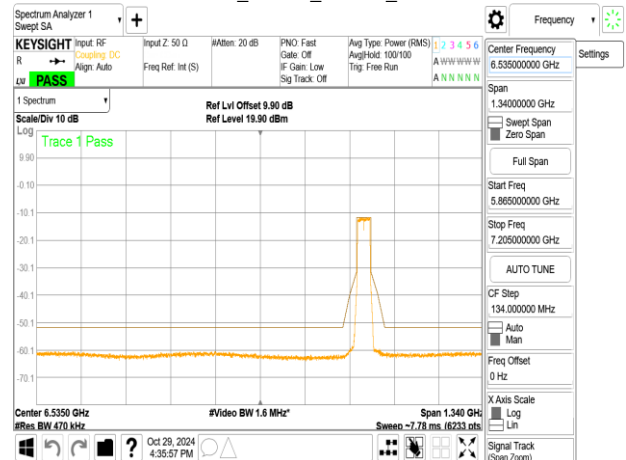
802.11ax_40MHz_ChainA_6845MHz_RU242_62
