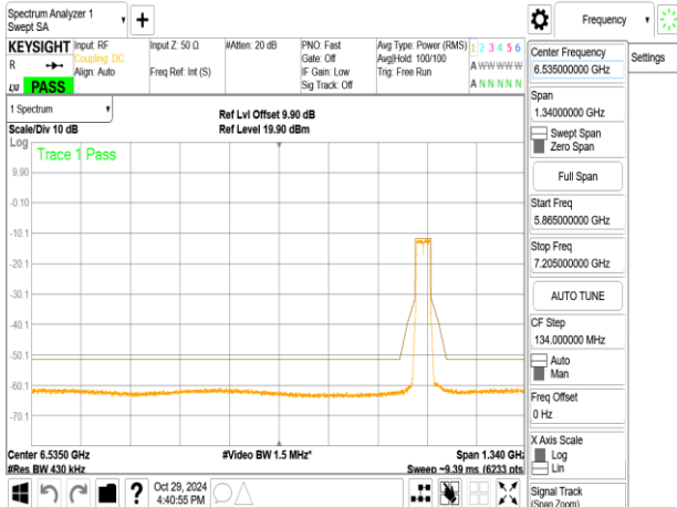
802.11ax_40MHz_ChainA_6925MHz_RU242_61
