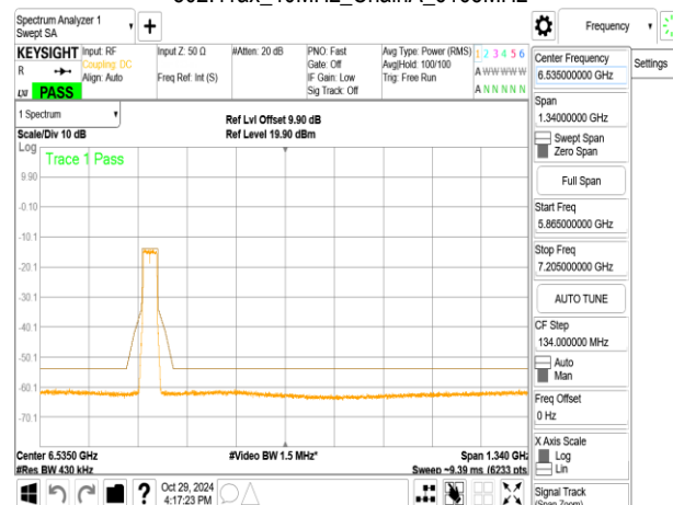
802.11ax_40MHz_ChainA_6405MHz
