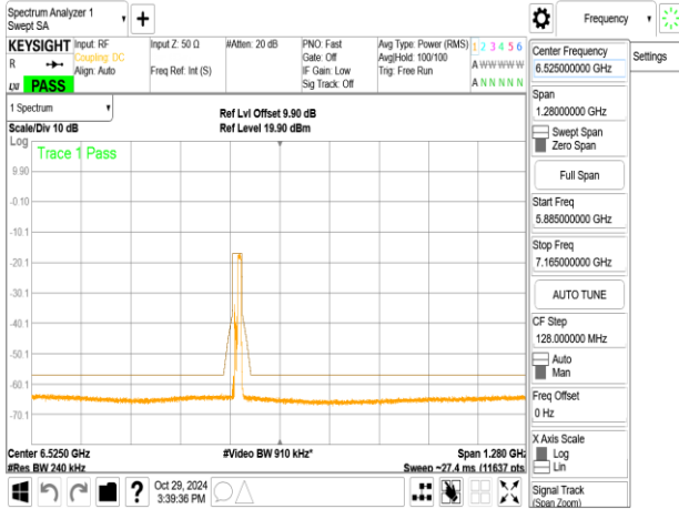
802.11ax_20MHz_ChainB_6415MHz_RU26_8
