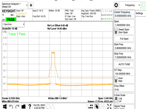
802.11ax_40MHz_ChainA_6445MHz_RU242_61
