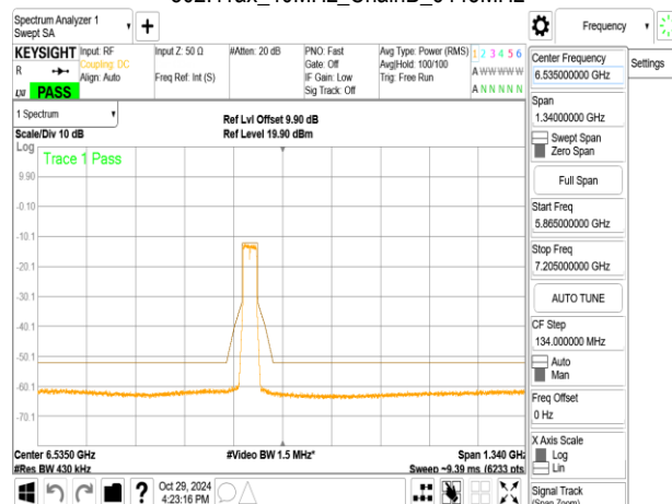
802.11ax_40MHz_ChainB_6445MHz_RU242_61
