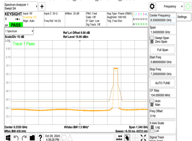
802.11ax_40MHz_ChainA_6885MHz
