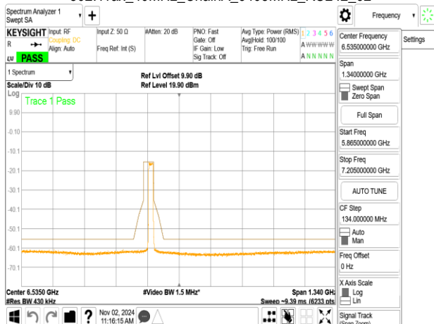
802.11ax_40MHz_ChainA_6445MHz
