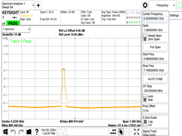
802.11ax_20MHz_ChainB_6415MHz_RU106_54
