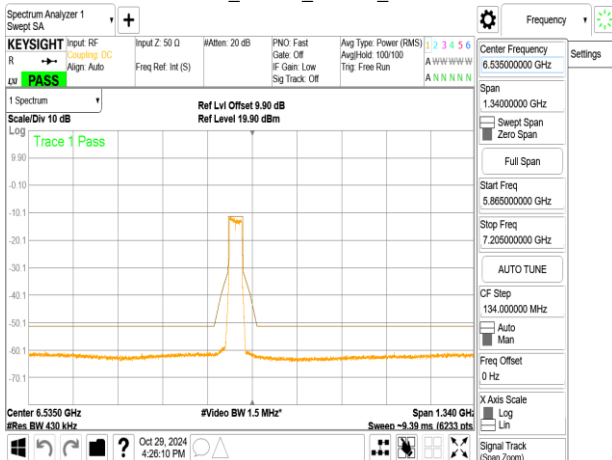
802.11ax_40MHz_ChainB_6485MHz_RU242_62
