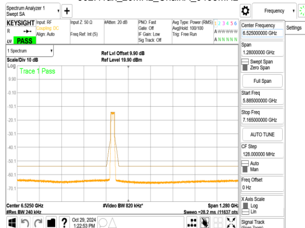
802.11ax_20MHz_ChainA_6435MHz_RU106_53
