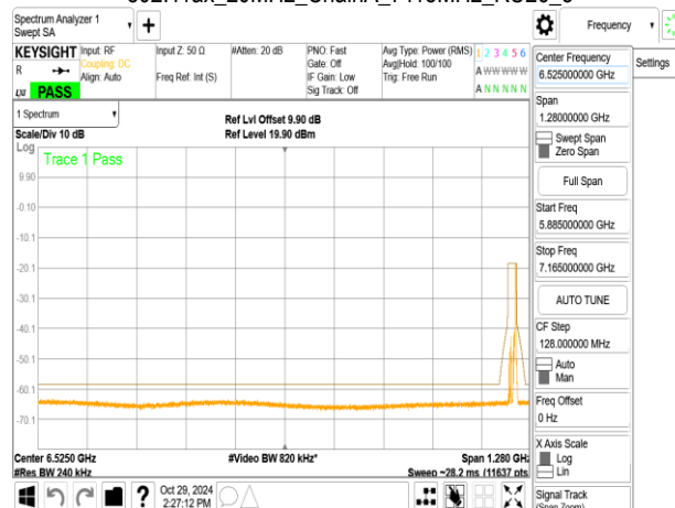
802.11ax_20MHz_ChainA_7115MHz_RU26_8
