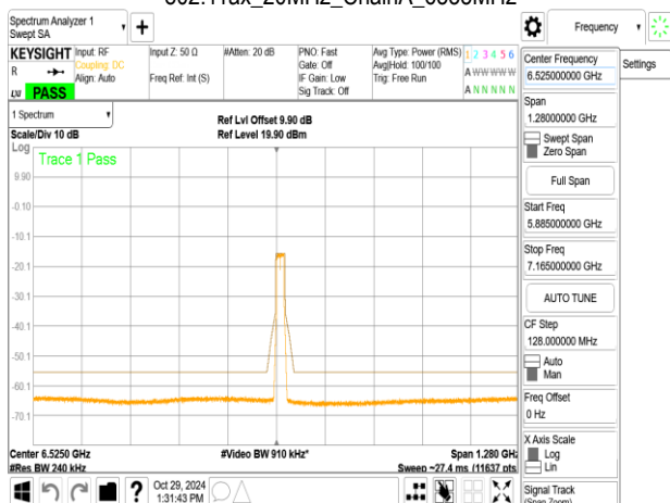
802.11ax_20MHz_ChainA_6535MHz_RU106_53
