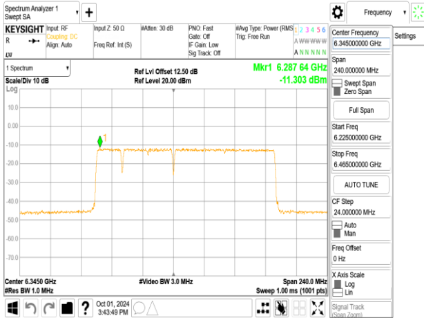
802.11be_160MHz_ChainB_6345MHz_996+484+242_MR5
