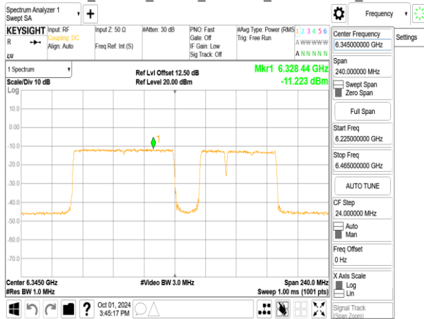
802.11be_160MHz_ChainA_6345MHz_996+484+242_MR07
