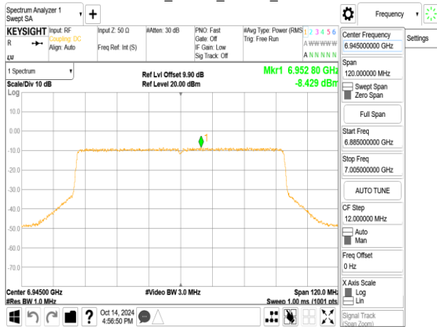
802.11be_80MHz_ChainB_6945MHz_484+242_MRU2
