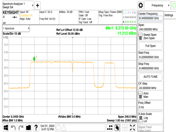
802.11be_160MHz_ChainA_6345MHz_996+484_MR01
