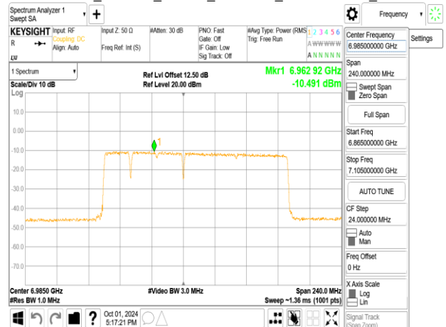
802.11be_160MHz_ChainA_6985MHz_996+484+242_MRU2
