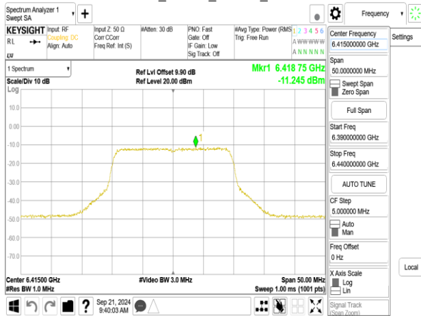
802.11be_20MHz_ChainB_6415MHz_106+26_MRU2
