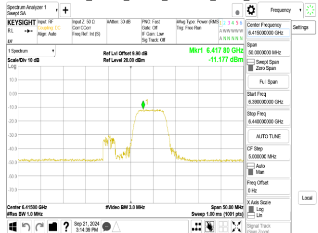
802.11be_20MHz_ChainA_6415MHz_RU106_54
