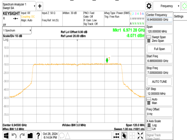
802.11ax_80MHz_ChainB_6945MHz_RU484_65
