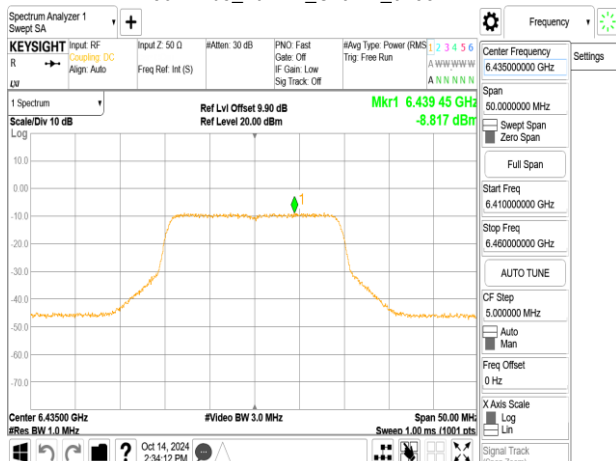
802.11be_20MHz_ChainA_6435MHz_106+26_MR1
