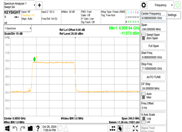
802.11ax_160MHz_ChainA_6985MHz_RU996_S67
