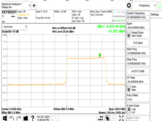
802.11ax_160MHz_ChainA_6345MHz_RU996_S67
