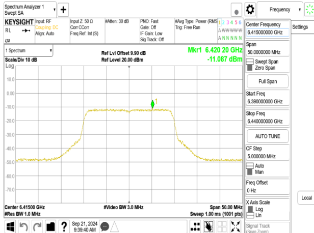
802.11be_20MHz_ChainA_6415MHz_106+26_MRUI2
