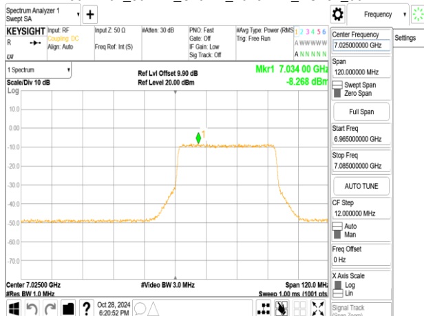
802.11ax_80MHz_ChainA_7025MHz_RU484_66
