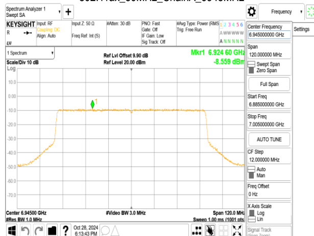
802.11ax_80MHz_ChainA_6945MHz
