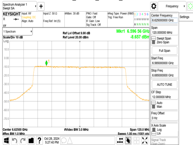
802.11ax_80MHz_ChainB_6625MHz_RU484_65
