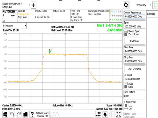
802.11ax_40MHz_ChainB_6485MHz_RU242_62
