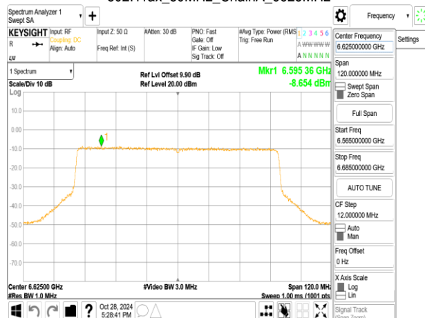
802.11ax_80MHz_ChainA_6625MHz
