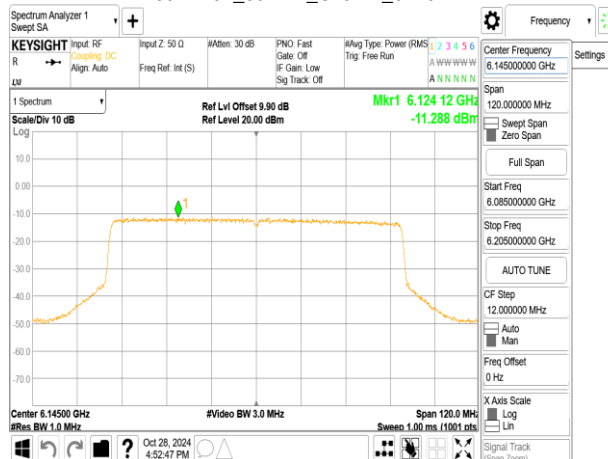
802.11ax_80MHz_ChainB_6145MHz
