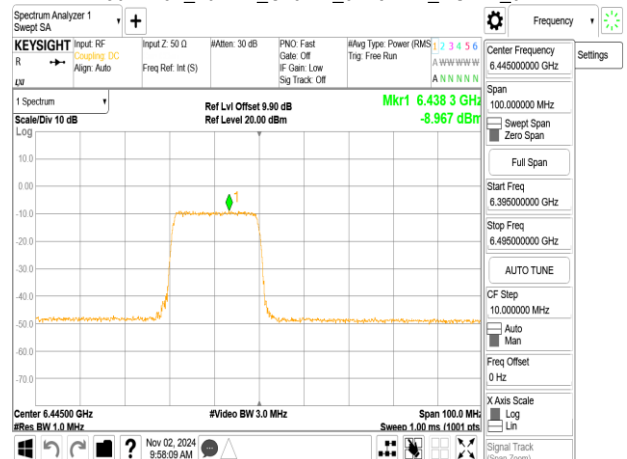
802.11ax_40MHz_ChainB_6445MHz_RU242_61
