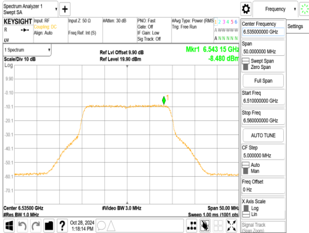
802.11ax_20MHz_ChainB_6535MHz_RU106_53
