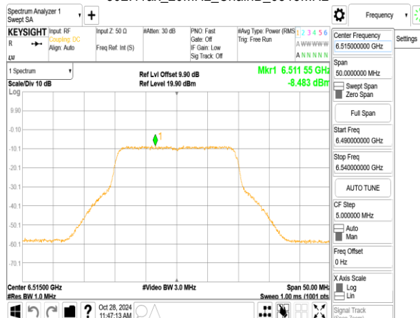
802.11ax_20MHz_ChainB_6515MHz_RU106_54
