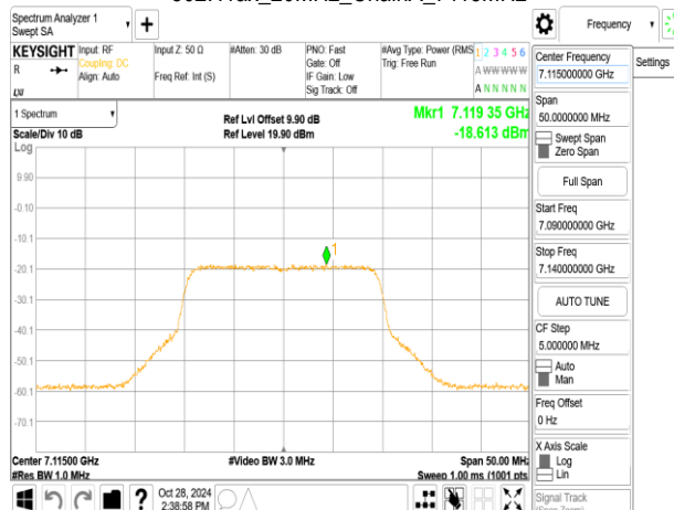
802.11ax_20MHz_ChainA_7115MHz_RU106_54
