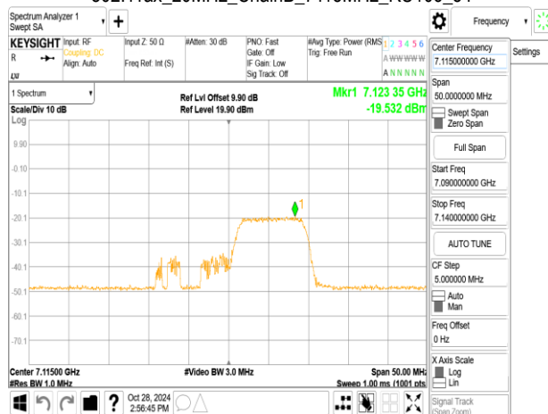
802.11ax_20MHz_ChainB_7115MHz_RU106_54
