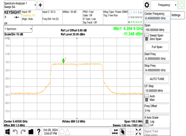
802.11ax_40MHz_ChainA_6405MHz
