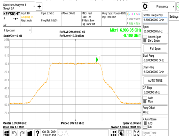
802.11ax_20MHz_ChainA_6895MHz_RU106_53
