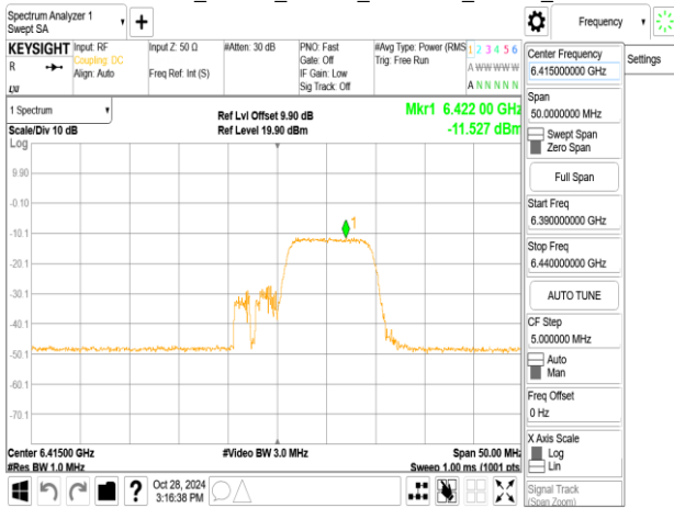
802.11ax_20MHz_ChainB_6415MHz_RU26_8
