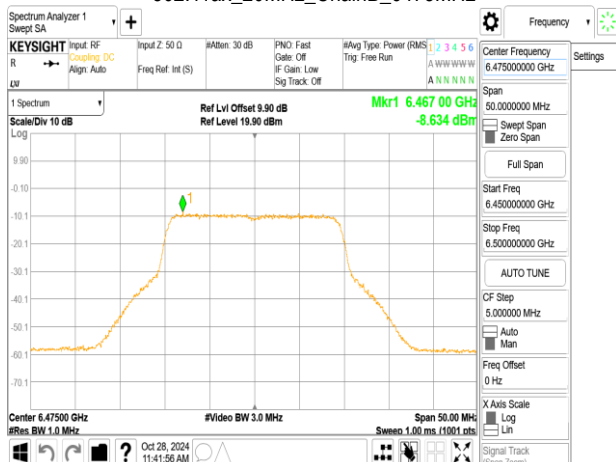
802.11ax_20MHz_ChainB_6475MHz
