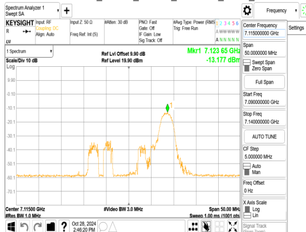
802.11ax_20MHz_ChainA_7115MHz_RU26_8
