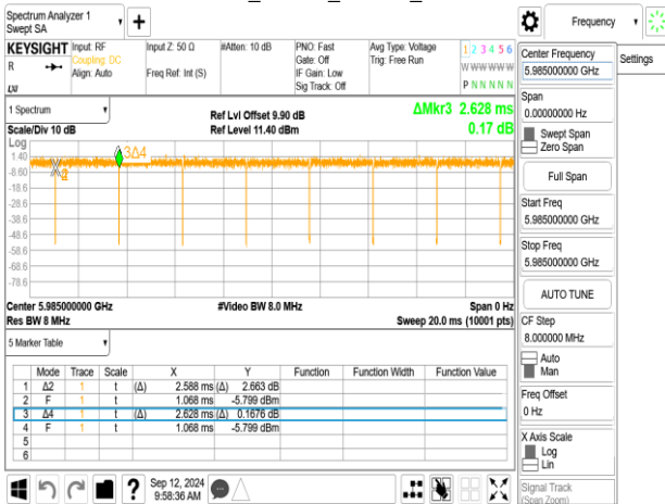
802.11ax_80MHz_ChainA_5985MHz_RU484_65
