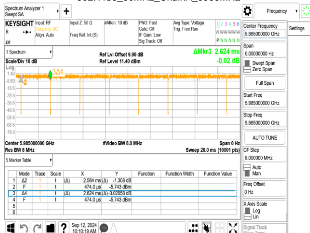
802.11be_80MHz_ChainA_5985MHz_484+242 MRU2
