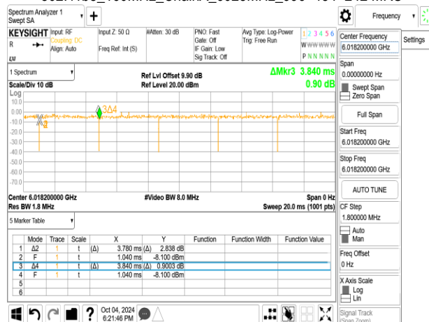
802.11be_160MHz_ChainA_6025MHz_996+484+242 MRU
