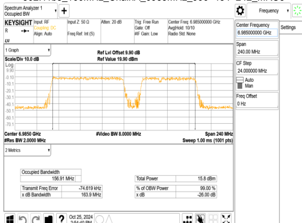
802.11be_160MHz_ChainA_6985MHz_996+484+242_MRU7
