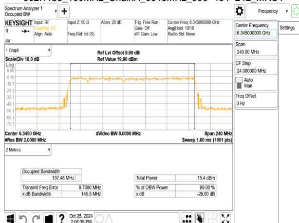
802.11be_160MHz_ChainA_6345MHz_996+484+242_MRU1
