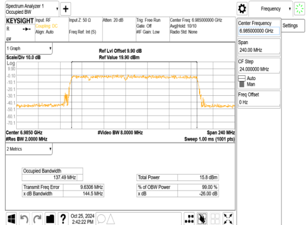
802.11be_160MHz_ChainA_6985MHz_996+484+242_MRU2
