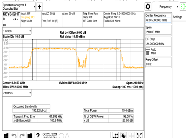
802.11be_160MHz_ChainA_6345MHz_996+484+242_MRU7
