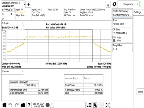
802.11be_80MHz_ChainB_6945MHz_484+242_MRU2
