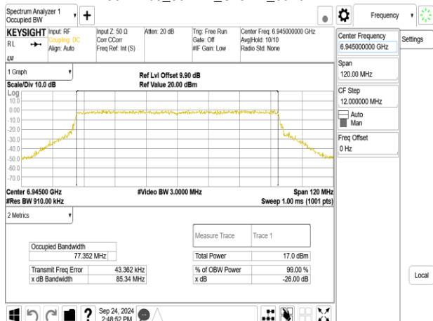
802.11be_80MHz_ChainA_6945MHz_484+242_MRU2
