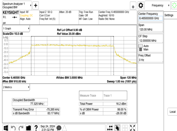
802.11be_80MHz_ChainA_6465MHz_484+242_MRU1
