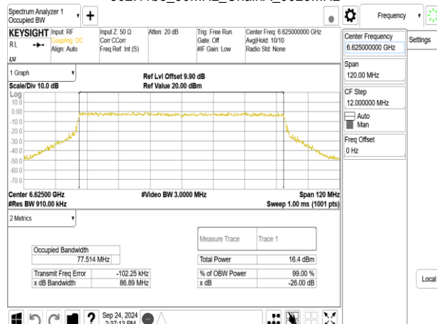
802.11be_80MHz_ChainA_6625MHz_484+242_MRU2
