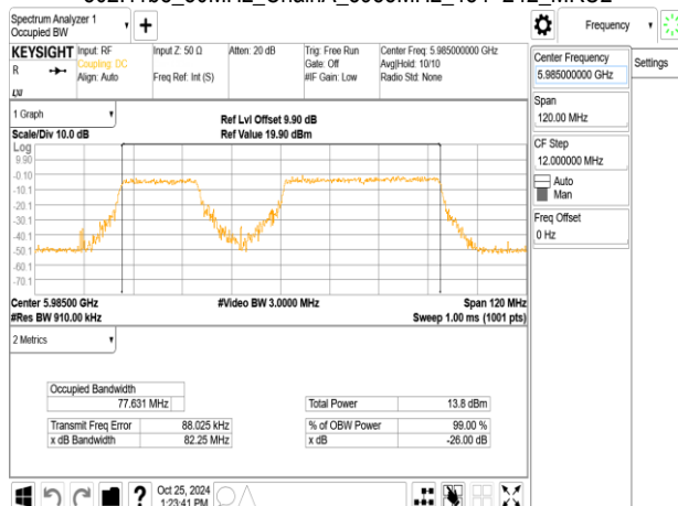
802.11be_80MHz_ChainA_5985MHz_484+242_MRU2
