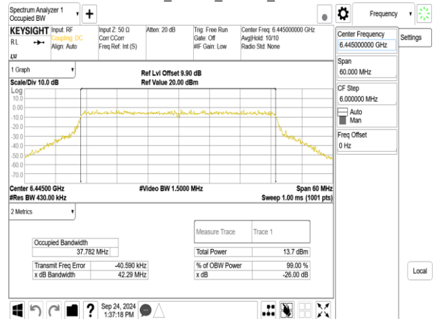
802.11be_40MHz_ChainA_6445MHz_RU242_61
