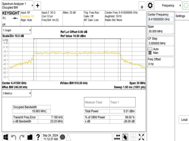
802.11be_20MHz_ChainB_6415MHz_106+26_MRU2
