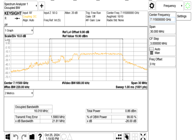
802.11be_20MHz_ChainB_7115MHz_106+26_MR2
