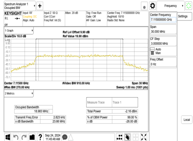
802.11be_20MHz_ChainB_7115MHz_106+26_MR2
