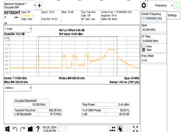
802.11ax_20MHz_ChainA_7115MHz_RU26_8
