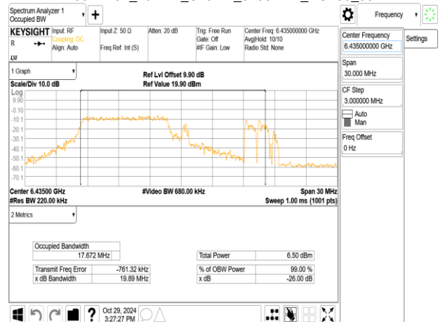
802.11ax_20MHz_ChainB_6435MHz_RU106_53
