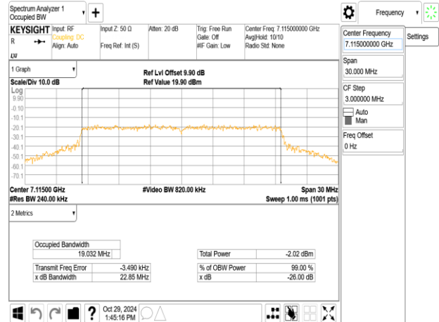
802.11ax_20MHz_ChainA_7115MHz_RU106_54
