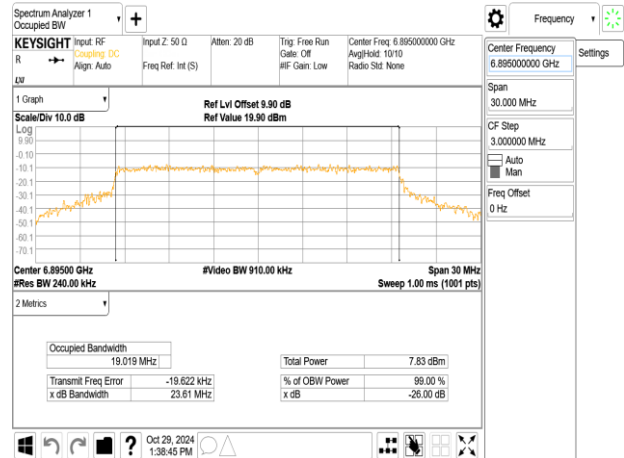
802.11ax_20MHz_ChainA_6895MHz_RU106_53
