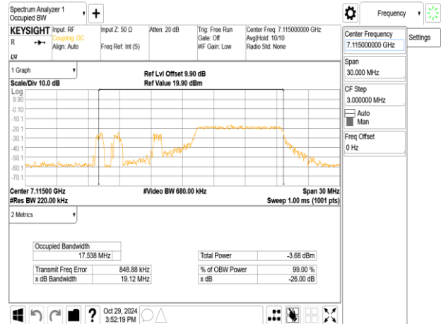
802.11ax_20MHz_ChainA_7115MHz_RU26_8
