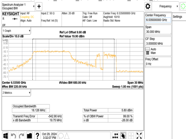
802.11ax_20MHz_ChainB_6535MHz_RU106_53
