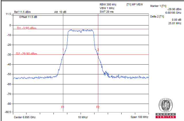
802.11ax (HE20)_Chain 0 / CH 149 (U-NII-7 Band)
