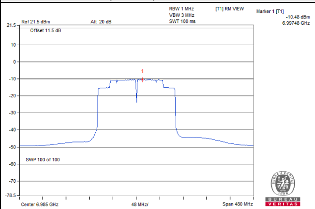
802.11ax (HE160) / Chain 1 / CH 207
