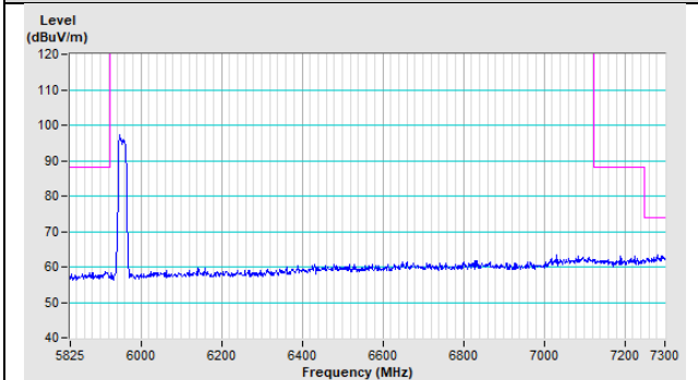
802.11ax (HE20) Channel 233
