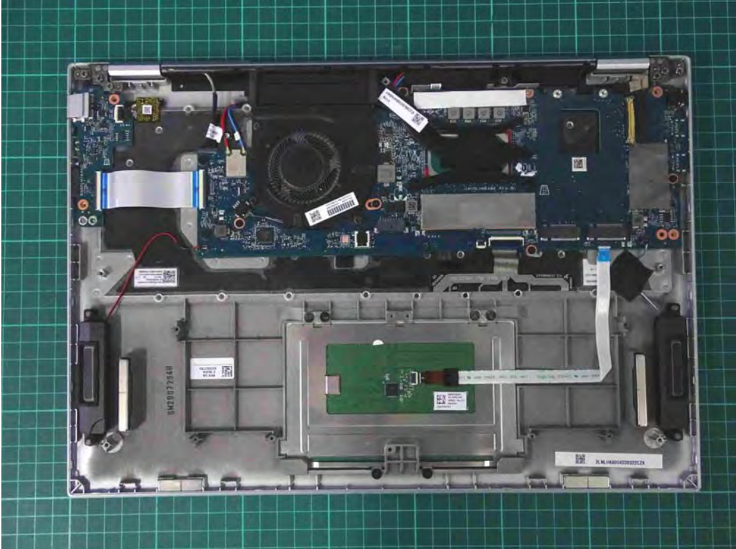
(25) EUT Photo
