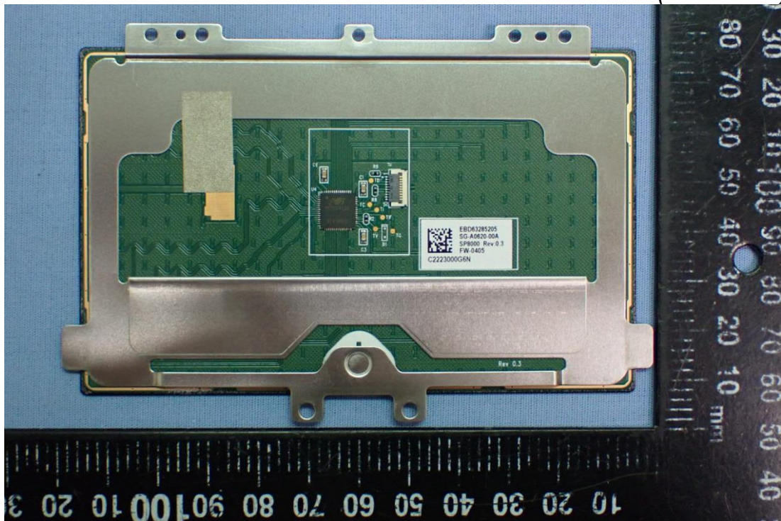
Figure 30 Touch Pad (Back View)
