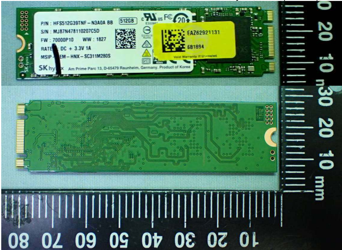
Figure 43 SK hynix, SSD (512GB) View
