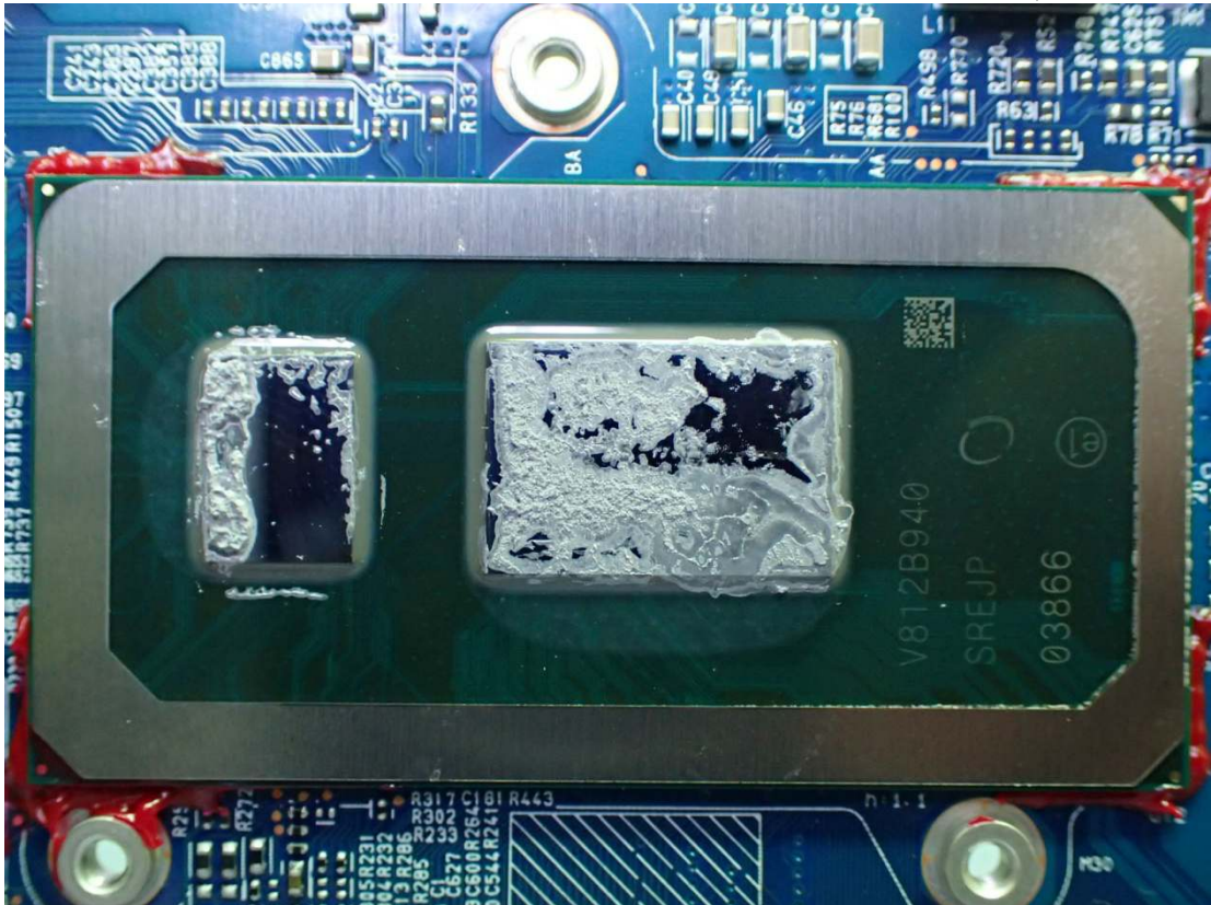
Figure 40 i5-8265U, CPU View
