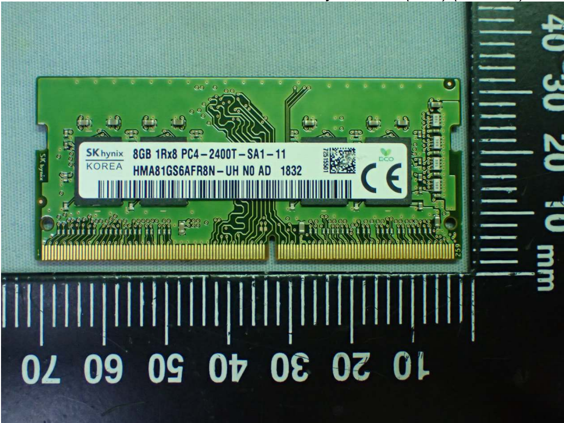
Figure 46 SK hynix, RAM (8GB) (On Card) View
