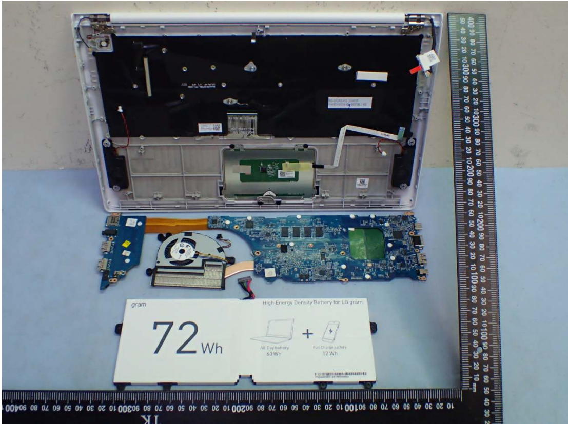
Figure 18 Internal View
