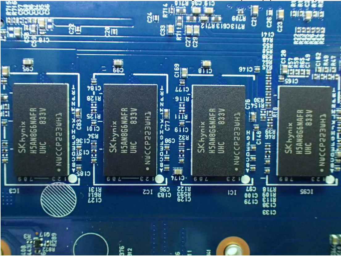
Figure 45 SK hynix, RAM (8GB) (On Board) View
