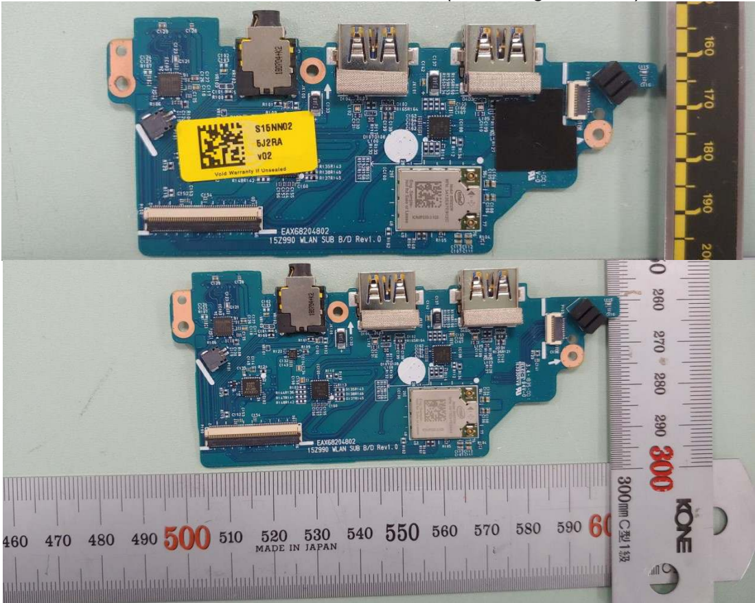
Figure 29 SUB Board (With Finger Printer), Front View
