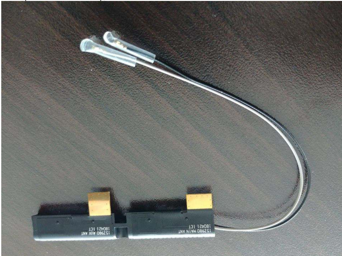
Figure 38 LG (LUXSHARE-ICT), M/N 15Z980 ANTENNA ASM WLAN Combo Antenna
