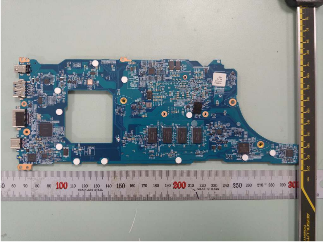
Figure 26 Main Board (with Thunderbolt), Back View
