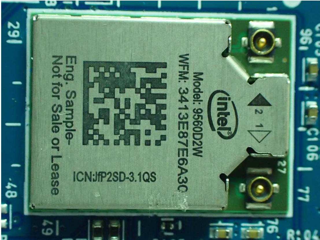
Figure 33 WLAN Combo Card View
