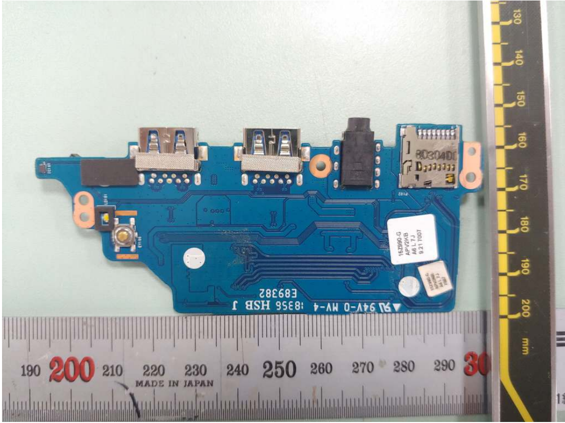
Figure 32 SUB Board (Without Finger Printer), Back View
