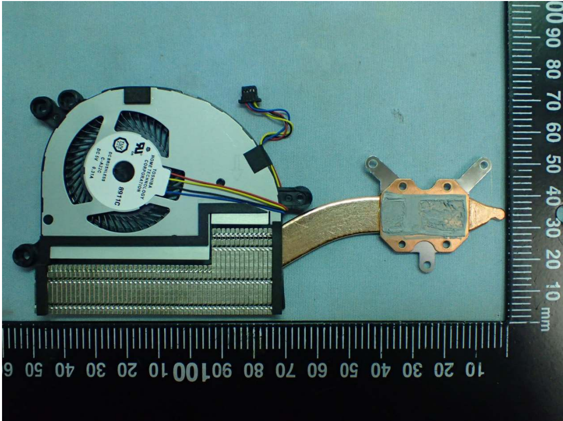
Figure 19 Internal View
