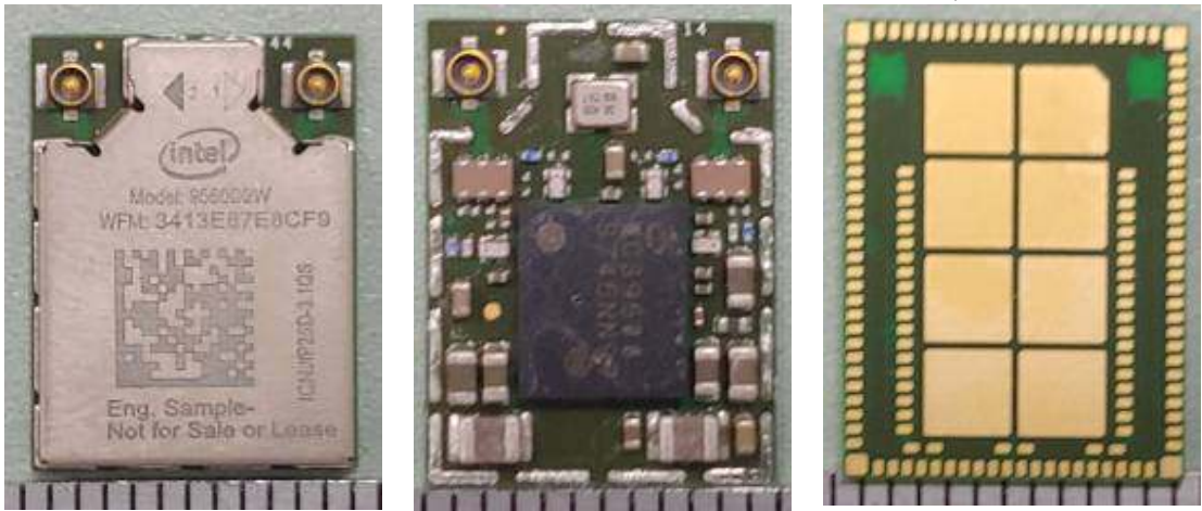
Figure 34 WLAN Combo Card, Remove Cover
