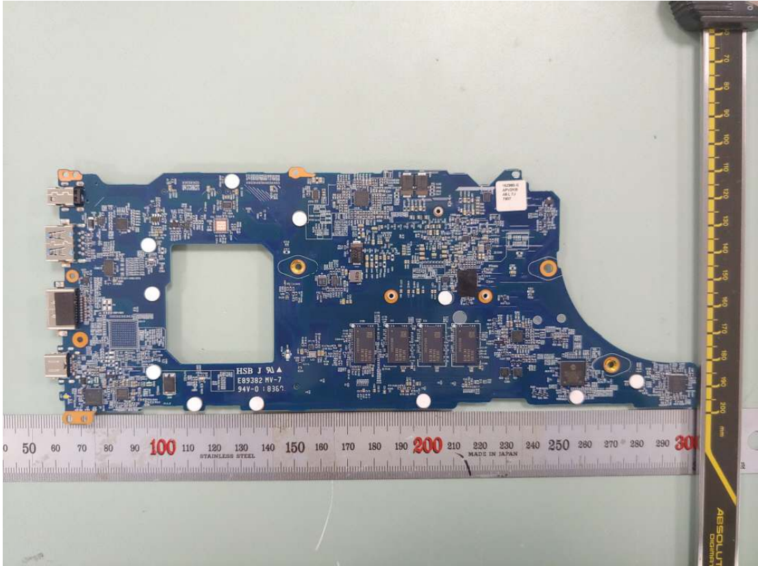
Figure 28 Main Board (without Thunderbolt), Back View
