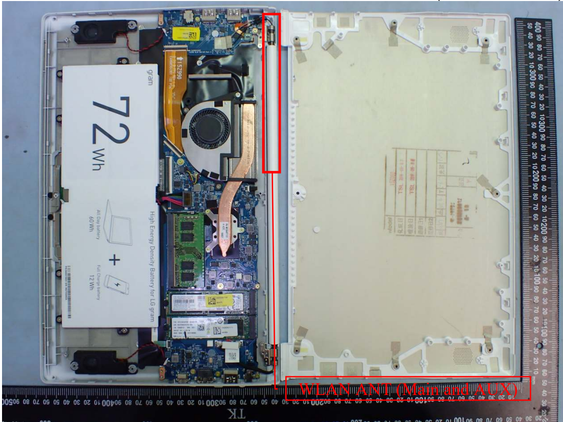
Figure 17 Internal View (Removed Cover)
