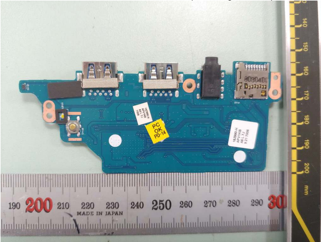
Figure 30 SUB Board (With Finger Printer), Back View
