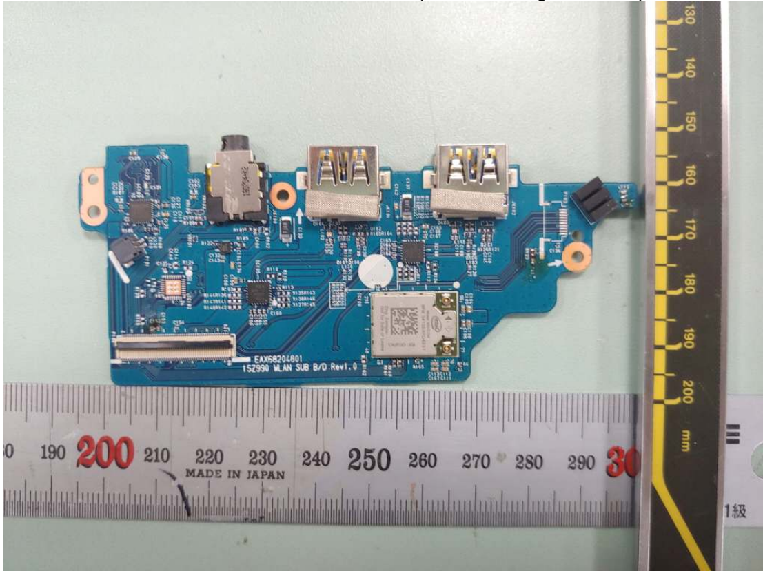
Figure 31 SUB Board (Without Finger Printer), Front View
