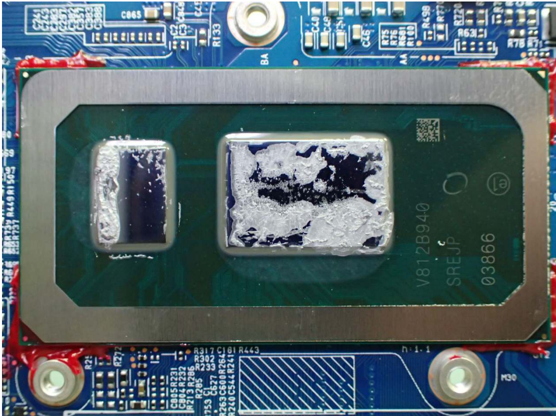
Figure 39 i7-8565U, CPU View
