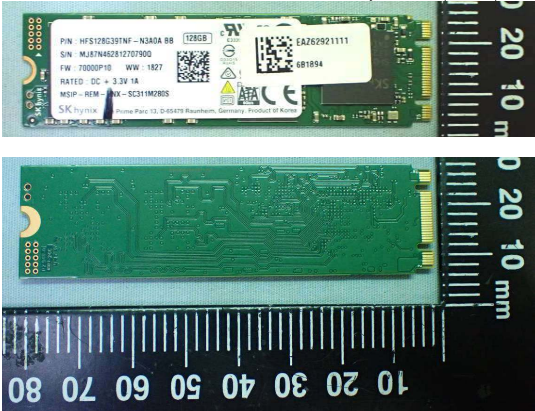
Figure 44 SK hynix, SSD (128GB) View
