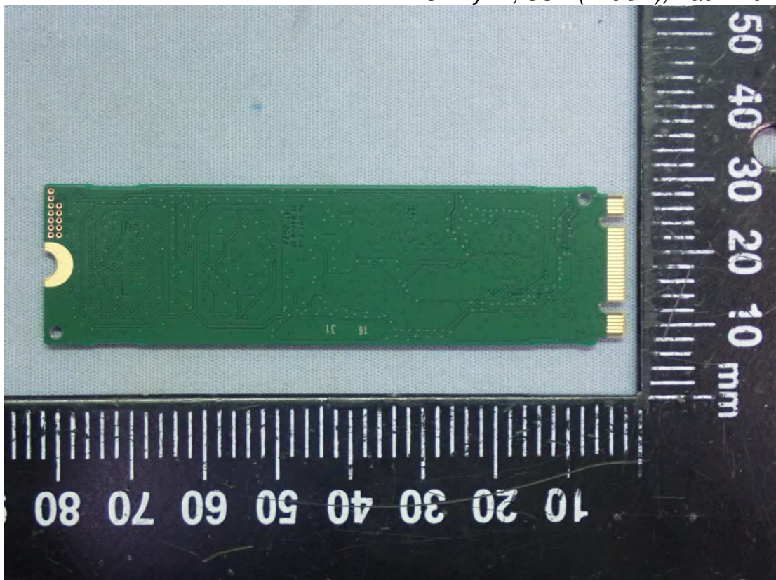
Figure 50 SK hynix, SSD (128GB), Back View
