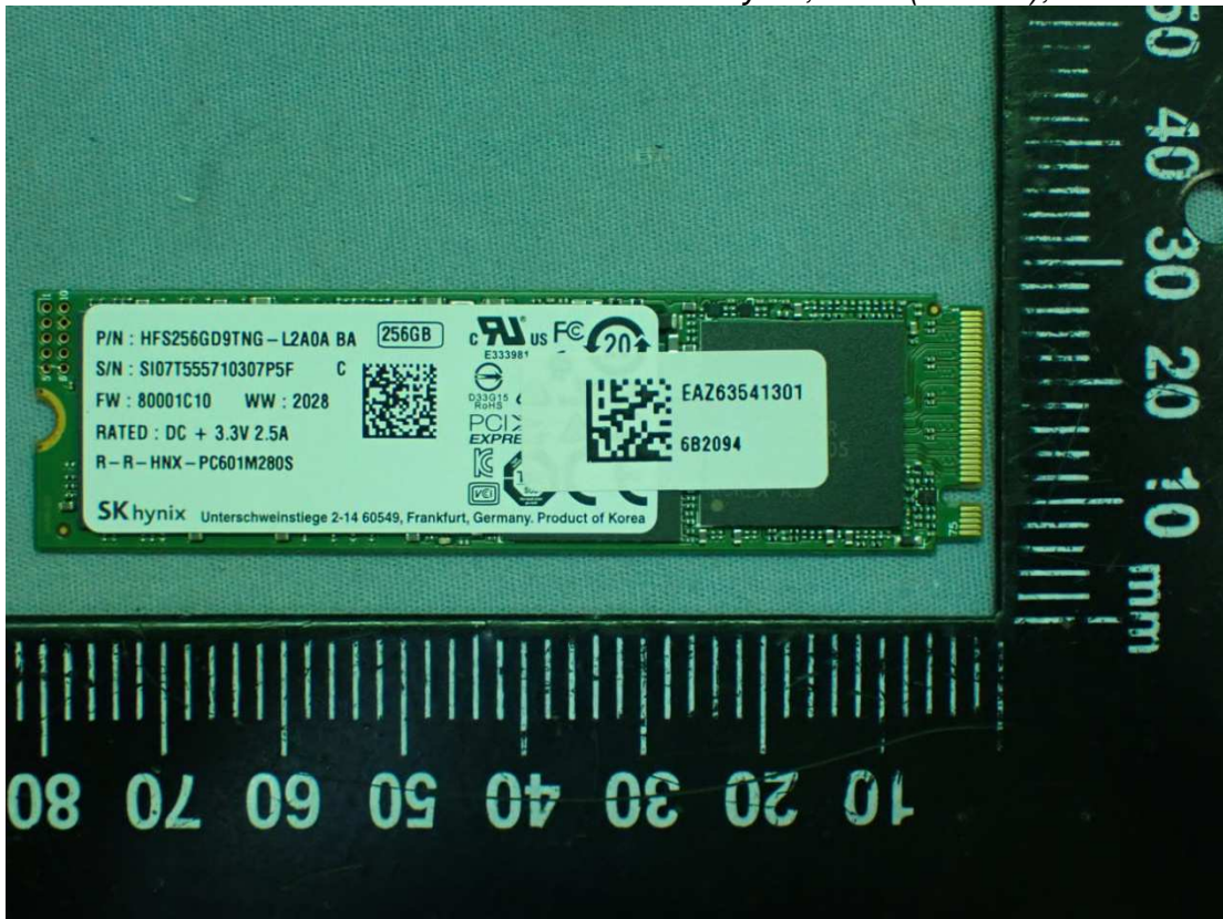
Figure 47 SK hynix, SSD (256GB), Front View
