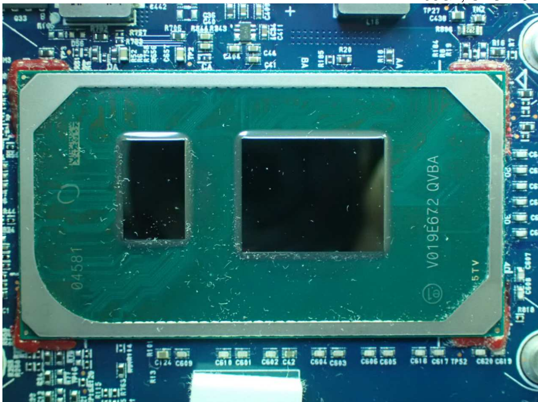
Figure 24 i7-1165G7, CPU View
