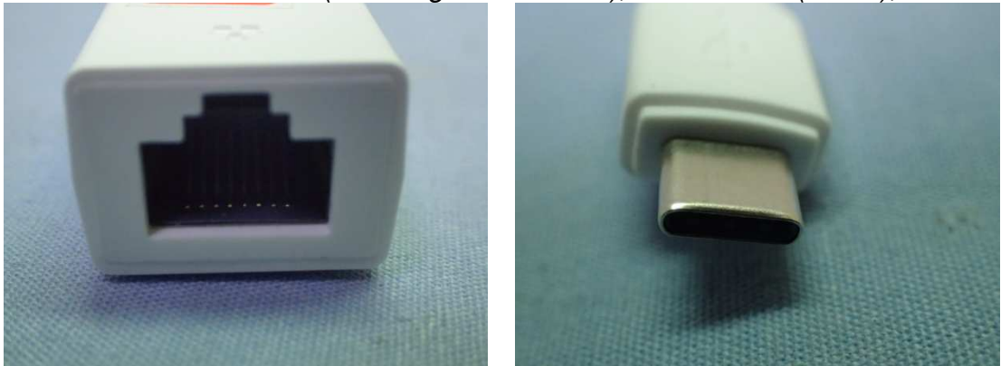
Figure 54 ARIN (100 Megabit Ethernet), LANGender (White), IO View
