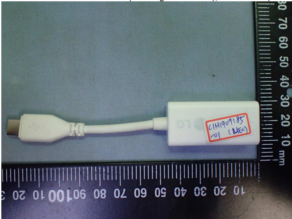
Figure 51 SUZHOU MEC (100 Megabit Ethernet), LANGender (White)
