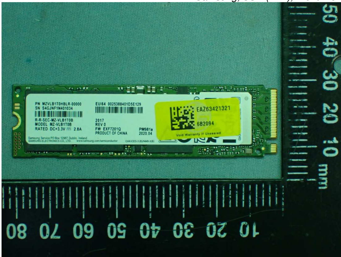
Figure 45 Samsung, SSD (1TB), Front View
