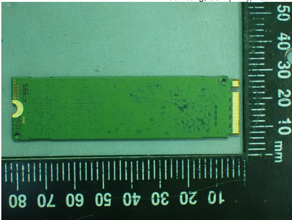
Figure 46 Samsung, SSD (1TB), Back View
