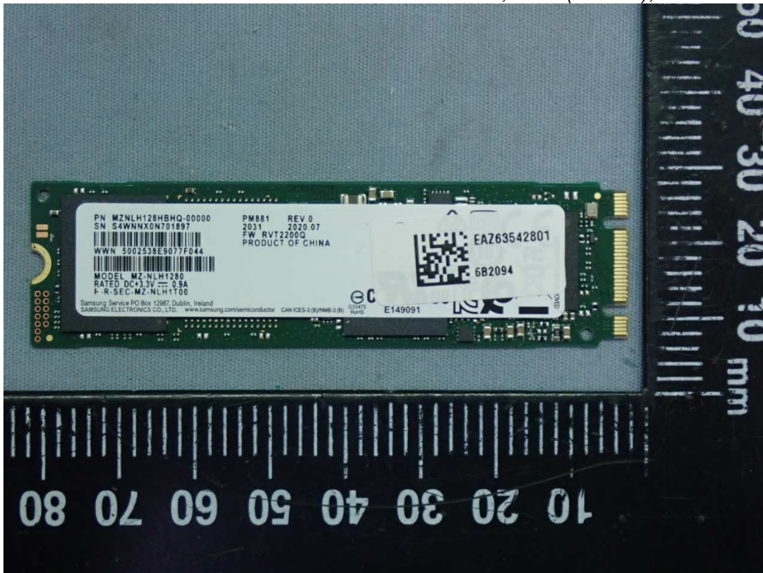
Figure 49 SAMSUNG, SSD (128GB), Front View
