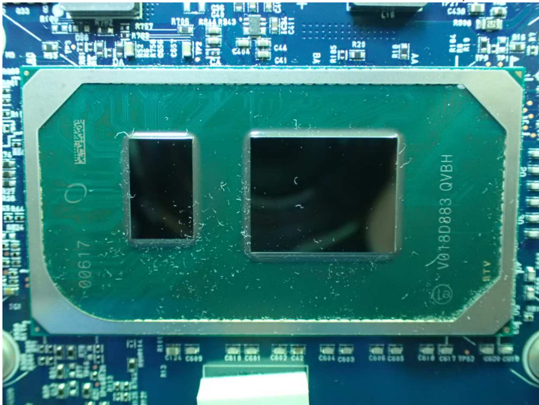
Figure 25 i5-1135G7, CPU View
