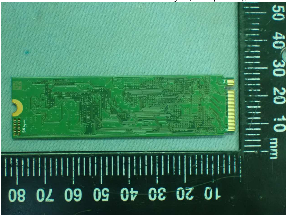
Figure 48 SK hynix, SSD (256GB), Back View
